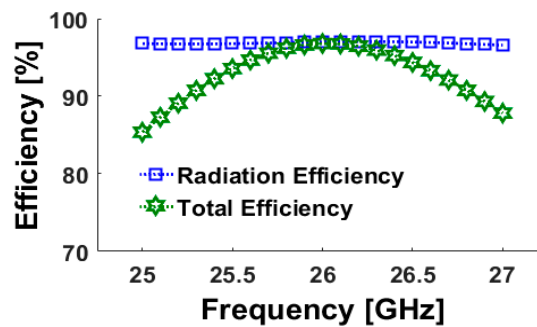
Figure 5. Simulated efficiencies.
