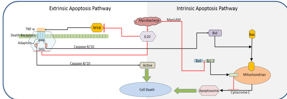
Fig. 2: Apoptotic pathway inhibition by pathogenic mycobacteria according to Koul et al. [16]. Pathogen mycobacteria interfere in intrinsic apoptotic pathway suppressing Ca^{2+} and releasing Bcl-2. In the extrinsic apoptotic pathway it inhibits binding ligands and DISC formation.
