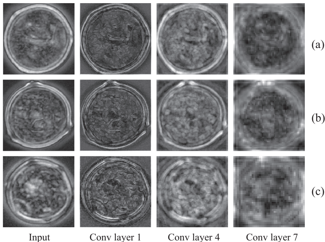
Fig. 8. Example of feature maps of VGG16. (a) Parietaria . (b) Urtica . (c) Urtica membranacea . Column 1 represents the input data, column 2–4 are the output of convolutional layer 1, 4, and 7, respectively.
