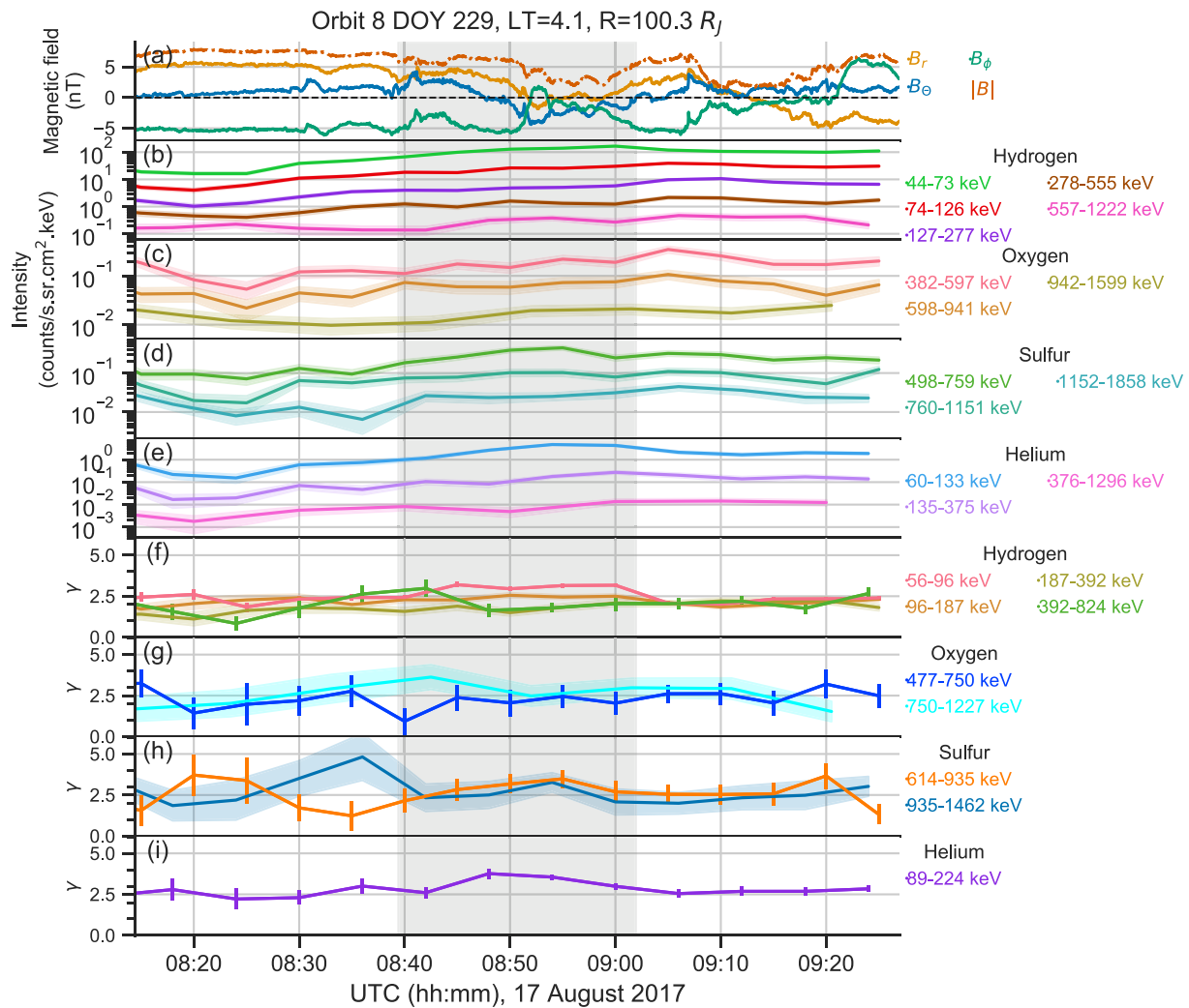
Figure 3. (a): JUNO magnetometer data of the magnetic field components during the plasmoid event on DOY 229 of 2017. (b–e): Ion intensities for hydrogen, oxygen, sulfur, and helium ions at different energy channels observed with Juno Energetic particle Detector Instrument. The intensities are averaged over a sampling interval which we adjust for each ion species and energy channel separately according to Section 4.3. For further information see text in Section 4.4. (f–i): Spectral index \gamma calculated from the ion intensities shown in (b–e) for different energy ranges. The energy ranges represent the geometric mean between the lowest energies of the neighboring channels. \gamma for helium ions at 224–698 keV was not calculated for this event because the relative error in helium ion intensity at 376–1296 keV (panel (e)) is above 30%. The bands and bars in panels (b–e) show the relative error obtained from the Poisson statistical error of the counts and in panels (f–i) the uncertainty in \gamma using error propagation of the errors in the ion intensities and Equation 1. Gray bars indicate the time of the plasmoid signature.
