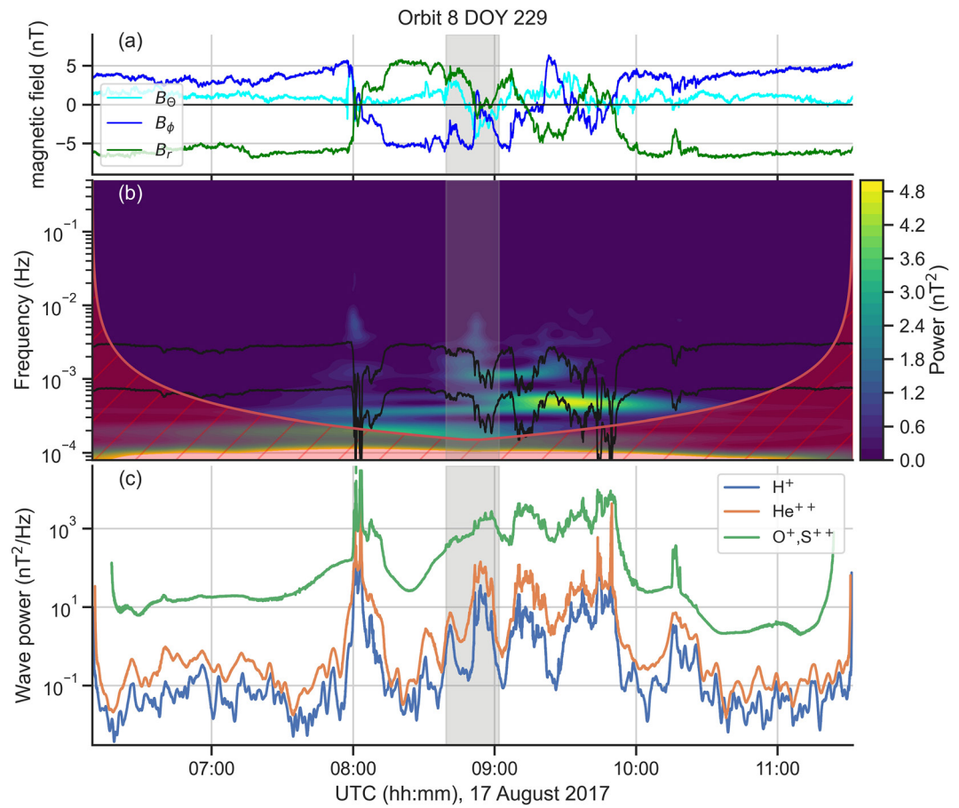
Figure 2. (a) Time series of the magnetic field components observed by Juno magnetometer. (b) Continuous wavelet power spectrum calculated from the wavelet analysis of B_\phi fluctuations. Black lines on the wavelet power spectrum indicate the integration range at 0.1f_{\text{SC}} and 0.4f_{\text{SC}} for \text{O}^+ for the calculation of wave power. The cone of influence is indicated by the red line and the red hatched area. (c) Wave power of the magnetic field fluctuations at characteristic frequencies of each ion species for \text{H}^+ , \text{He}^{++} , \text{O}^+ , and \text{S}^{++} . Gray bars indicate the time of the plasmoid event.
