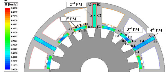
Fig. 22. Flux density distribution of PMs in the proposed machine under a two-times overload current.
