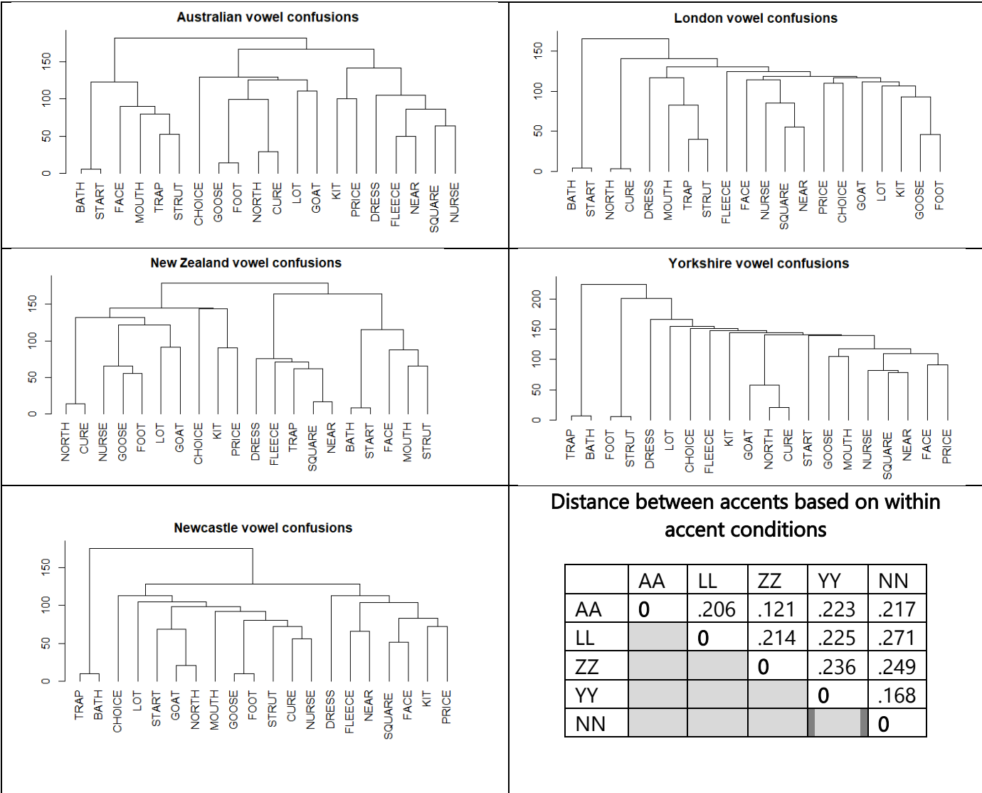
Figure 3: Dendrogram of each accent, based on listeners hearing their own accent, and a table showing the normalized distance between each accent (within-accent conditions). Greater numbers indicate a larger distance between responses. Distances are normalized to fall between 0 and 1, where 0 indicates identical responses and 1 indicates maximally different responses.
