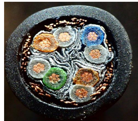
Fig. 2. Cross-section of a typical 8-wire RailCat 7 twisted-pair cable with seven conductor strands
