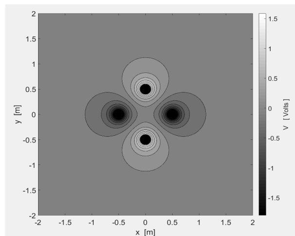
Fig. 6. 2D quadrupole potential of four charges, equal magnitude and alternating signs
