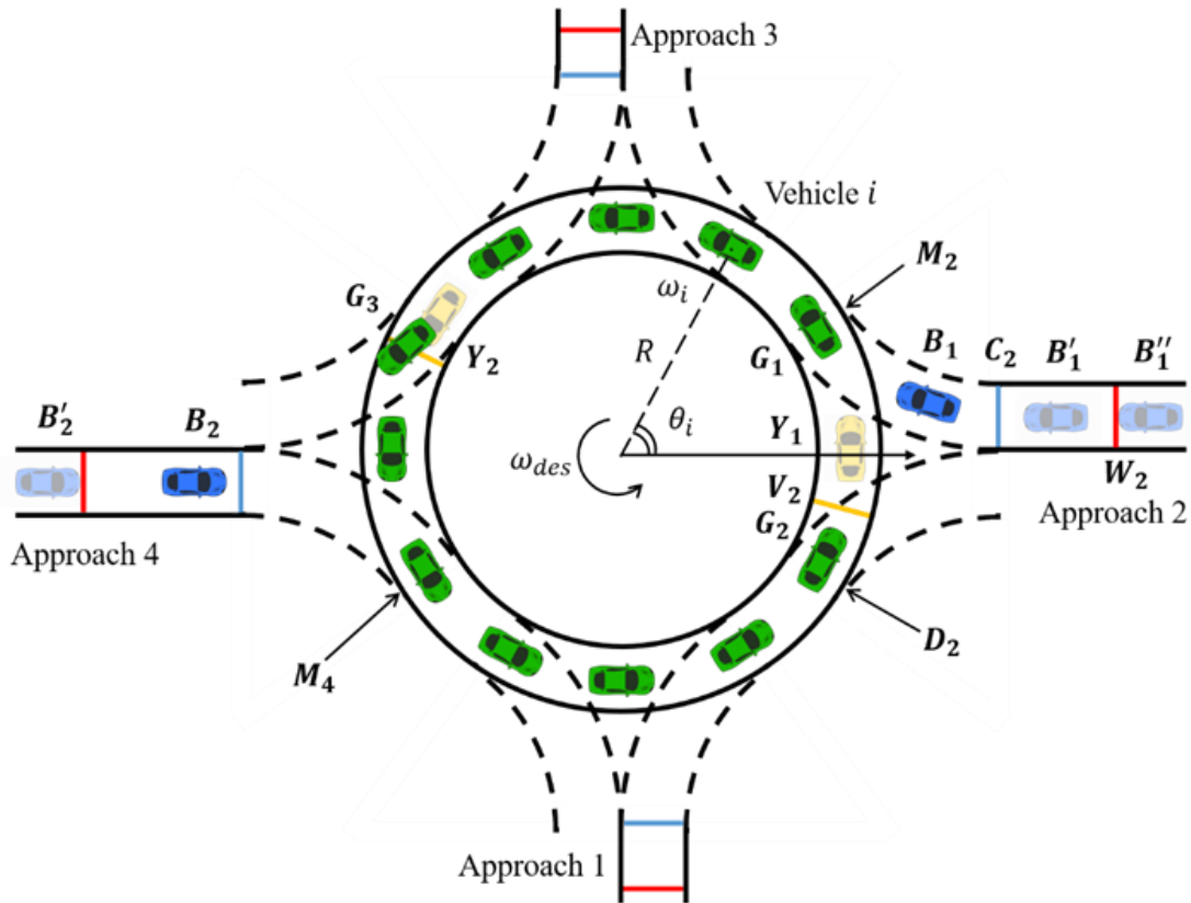
Figure 2.2: Illustration of self-adjusting stage and virtual platoon control stage in vehicles' merge-in procedure
