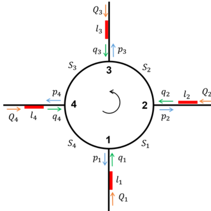
Figure 2.1: Four-approach roundabout
