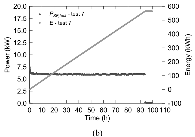
Fig. 8. Temperature and flow (a), and energy and power (b) evolution during tests 7.
