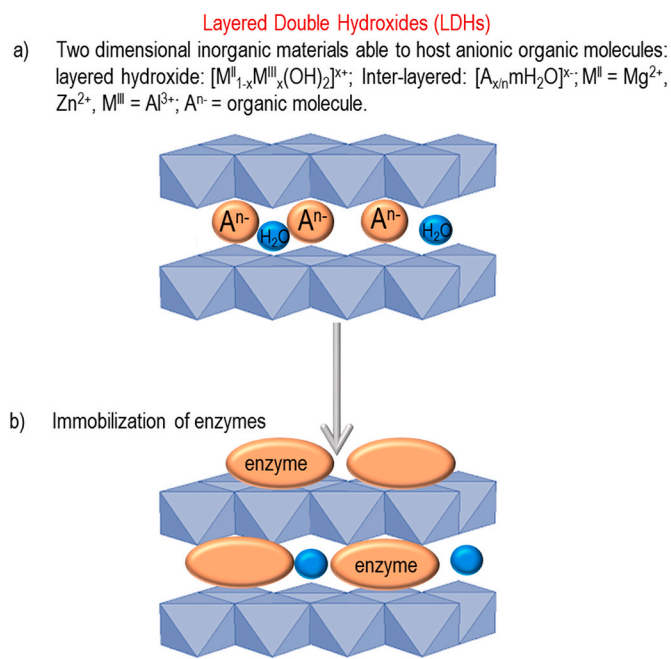
Fig. 2. a) Schematic representation of LDH and b) immobilization of enzymes for their thermal stabilisation.
