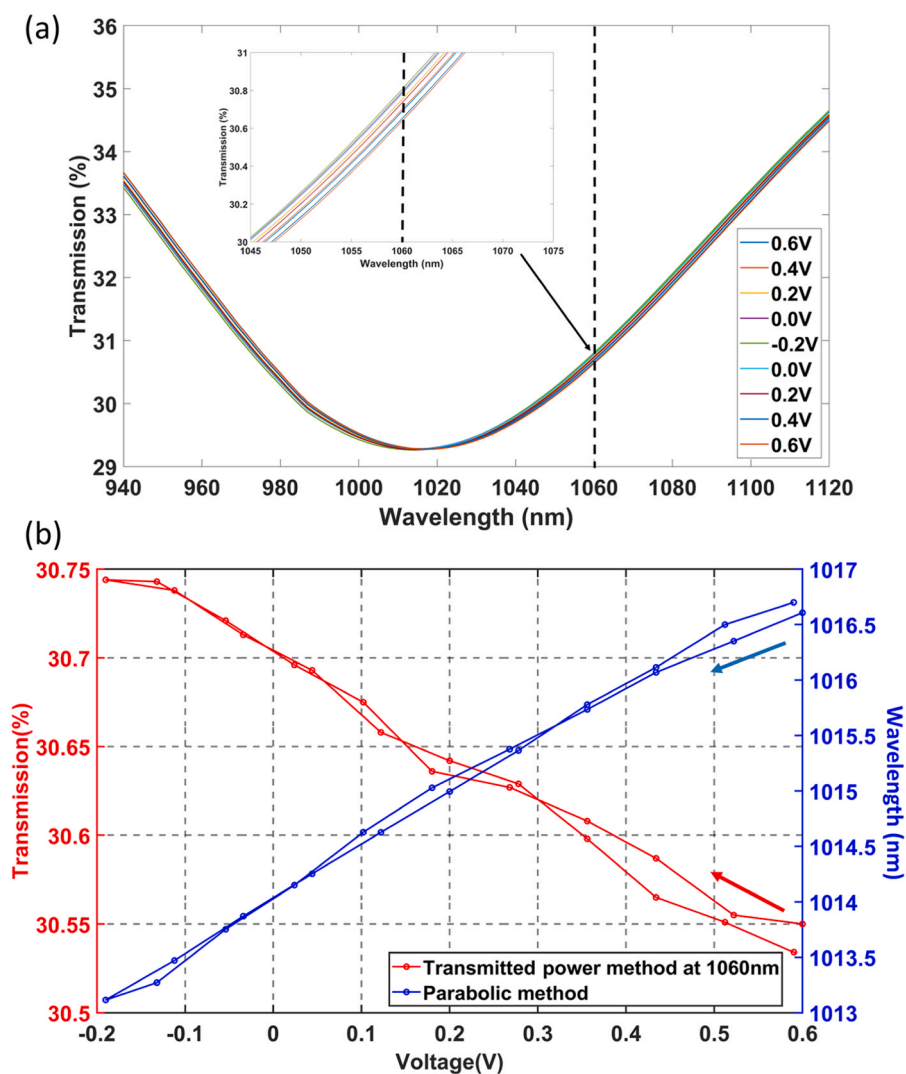
Fig. 3. Optical response of the LMR sensor to CV between 0.6 and -0.2 V with a scan rate of 100 mV/s in 0.1 M KCl solution containing \text{K}_3[\text{Fe}(\text{CN})_6] 1 mM: (a) Spectral evolution of the LMR for the 10th CV cycle; (b) Shift of the LMR wavelength and variation of the lateral slope of the LMR at the specific wavelength of 1060 nm for the 10th CV cycle.
