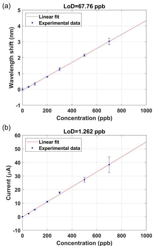
Fig. 7. Calibration curve of three experiments ( n = 3 ) for detection of Mn^{2+} ions in buffer obtained with the lineal fitting curve of the experimental points for the: (a) average value of the three slopes of the LMR wavelength shift obtained for each of the three cycles of CSV; (b) average value of the three current values obtained for each of the three cycles of CSV.
