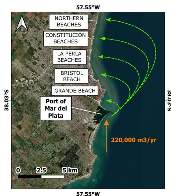
Figure 10. Schematic representation of a potential beach nourishment in the city of Mar del Plata, taking into account those sand embankments at the port entrance and the southern breakwater as loan zones.
