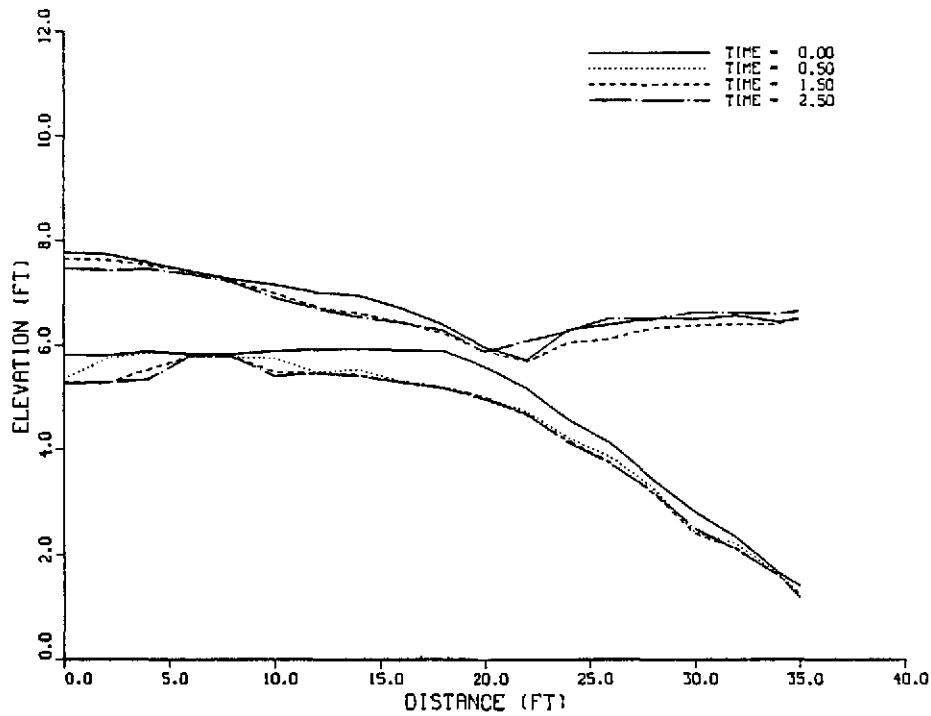
Bare-soil embankment.
