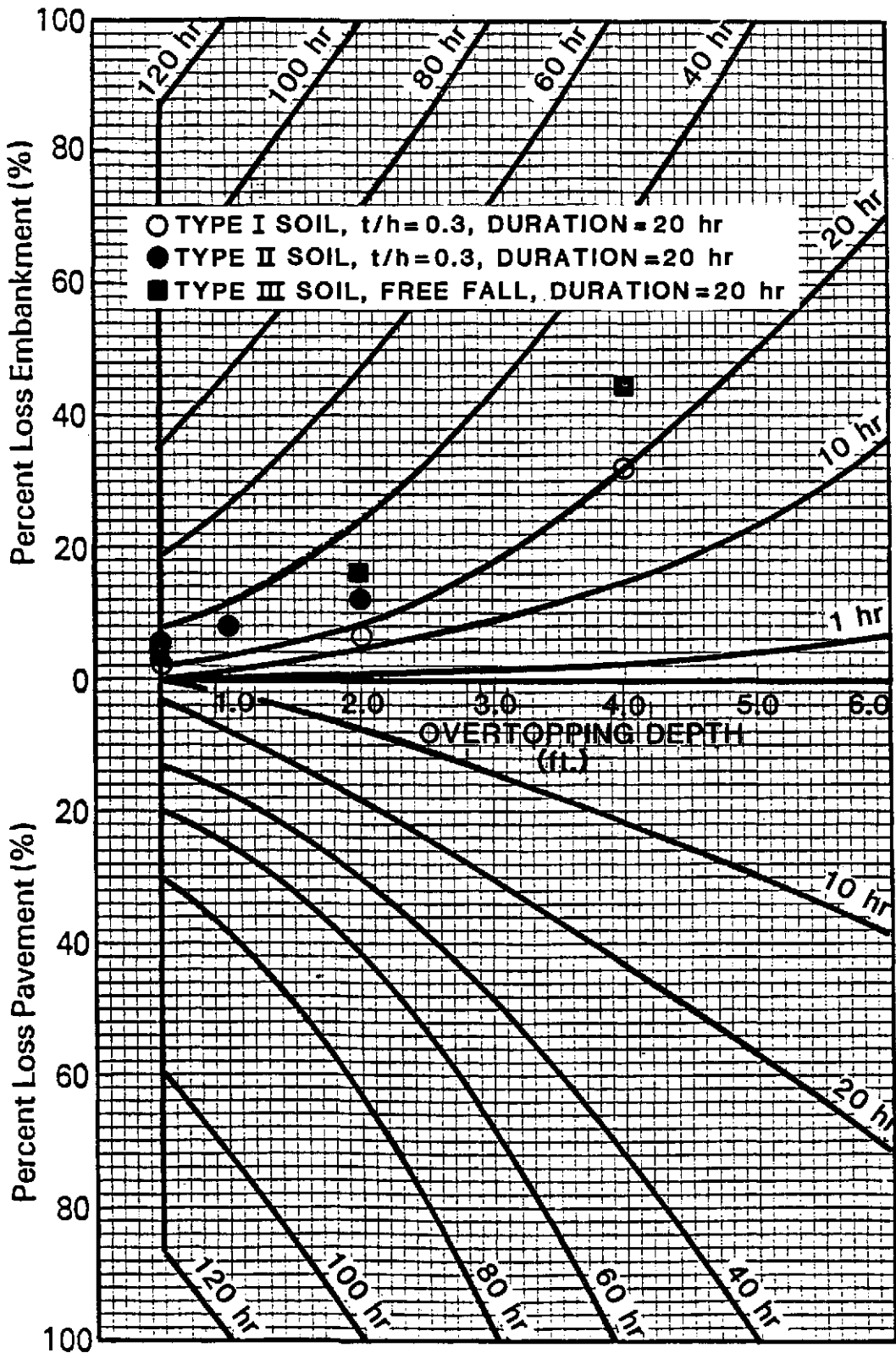
Figure 40. Embankment pavement losses (after Schneider and Wilson. (24))
