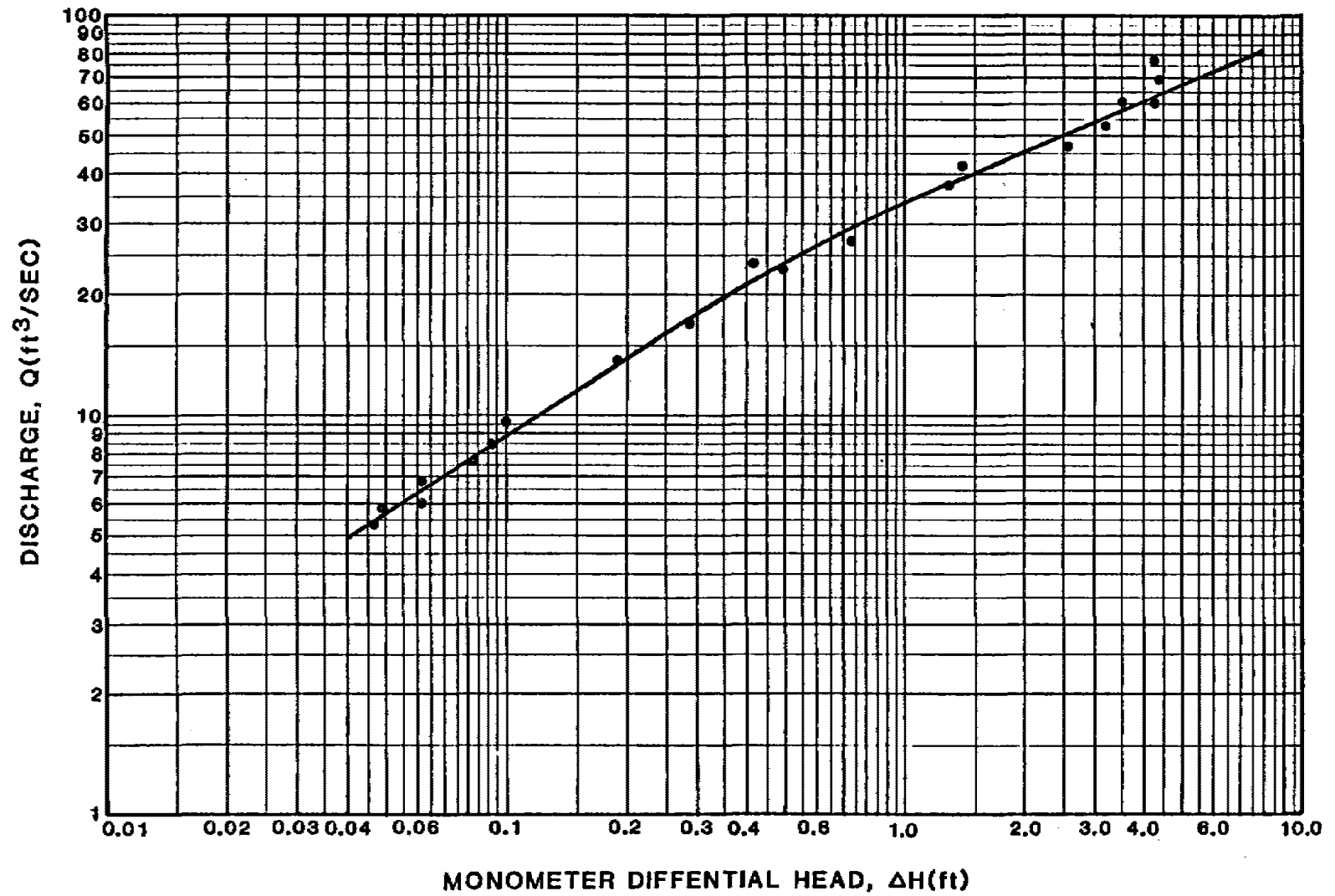
Figure 7. Calibration curve for discharge measurements.
