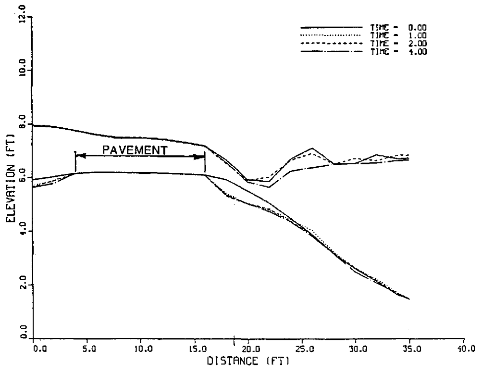
Paved embankment.
