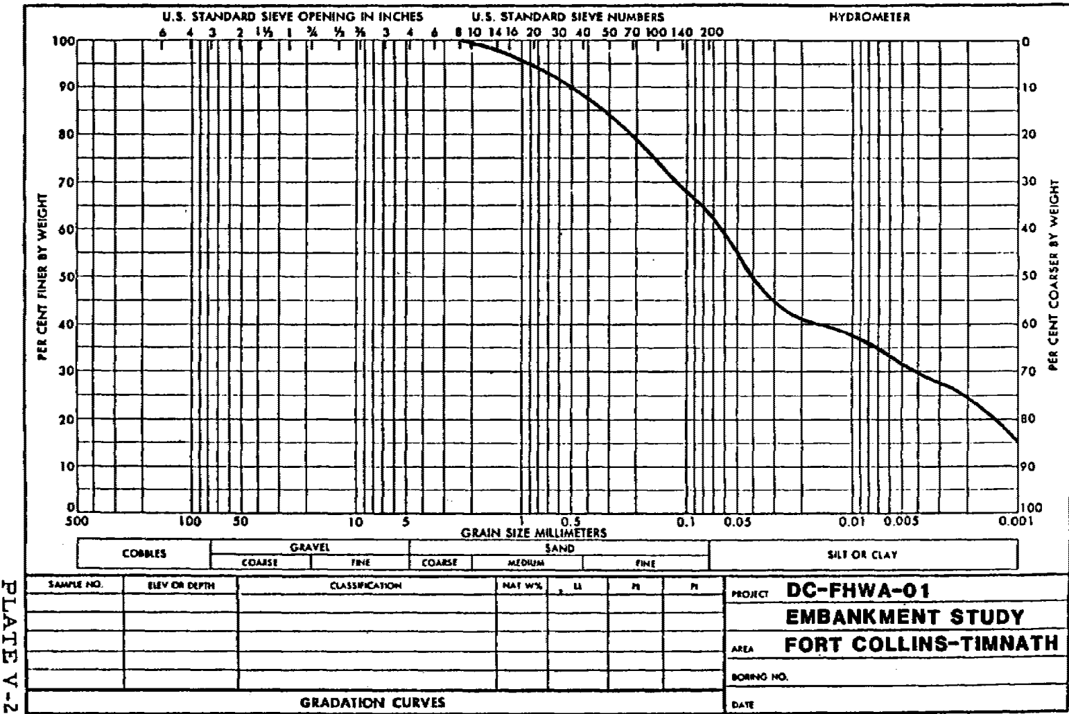
Figure 8. Size distribution for soil type I.
