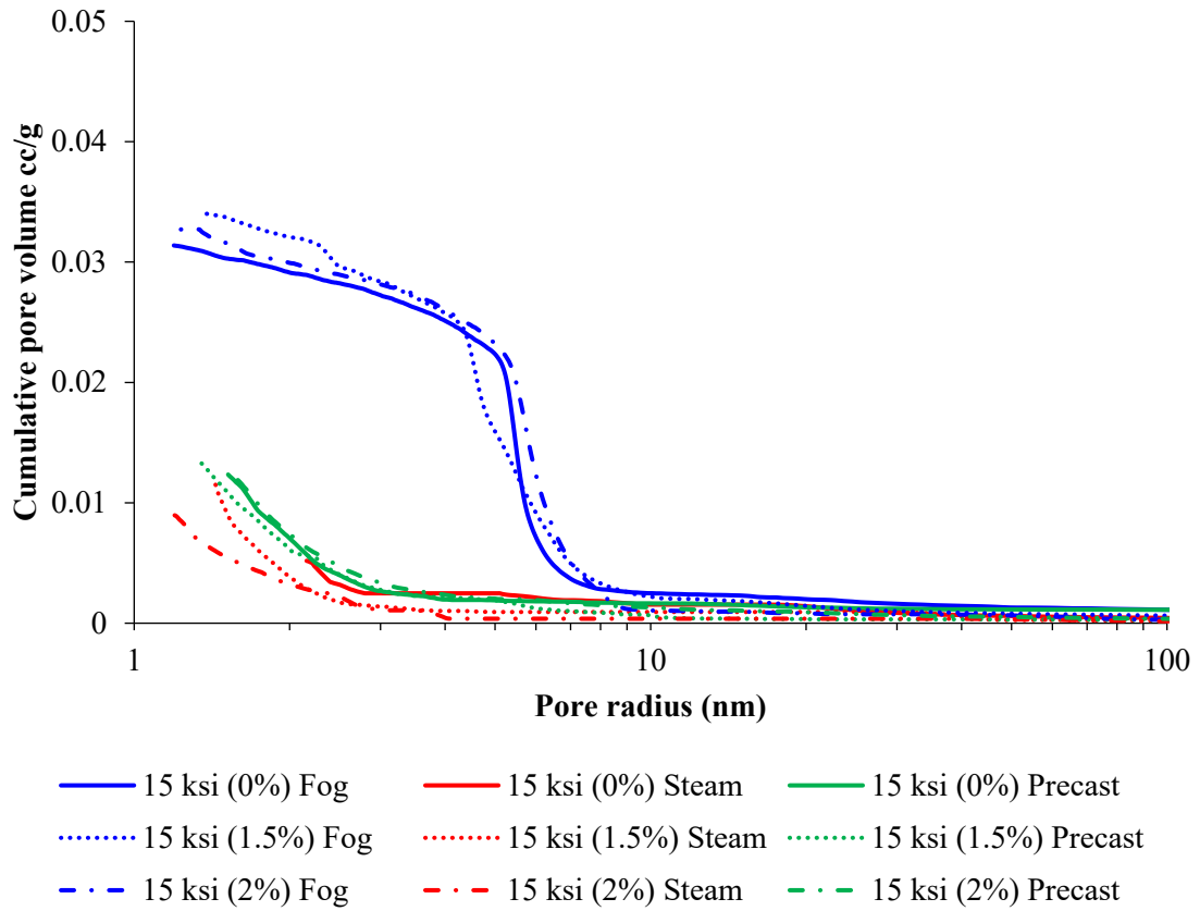
Figure 174: MIP cumulative pore volume of the 15 ksi mixture
