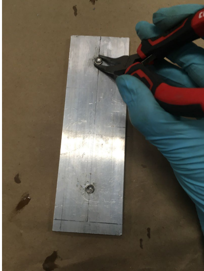
Figure 105: Gauge points with epoxy are placed in template notches
