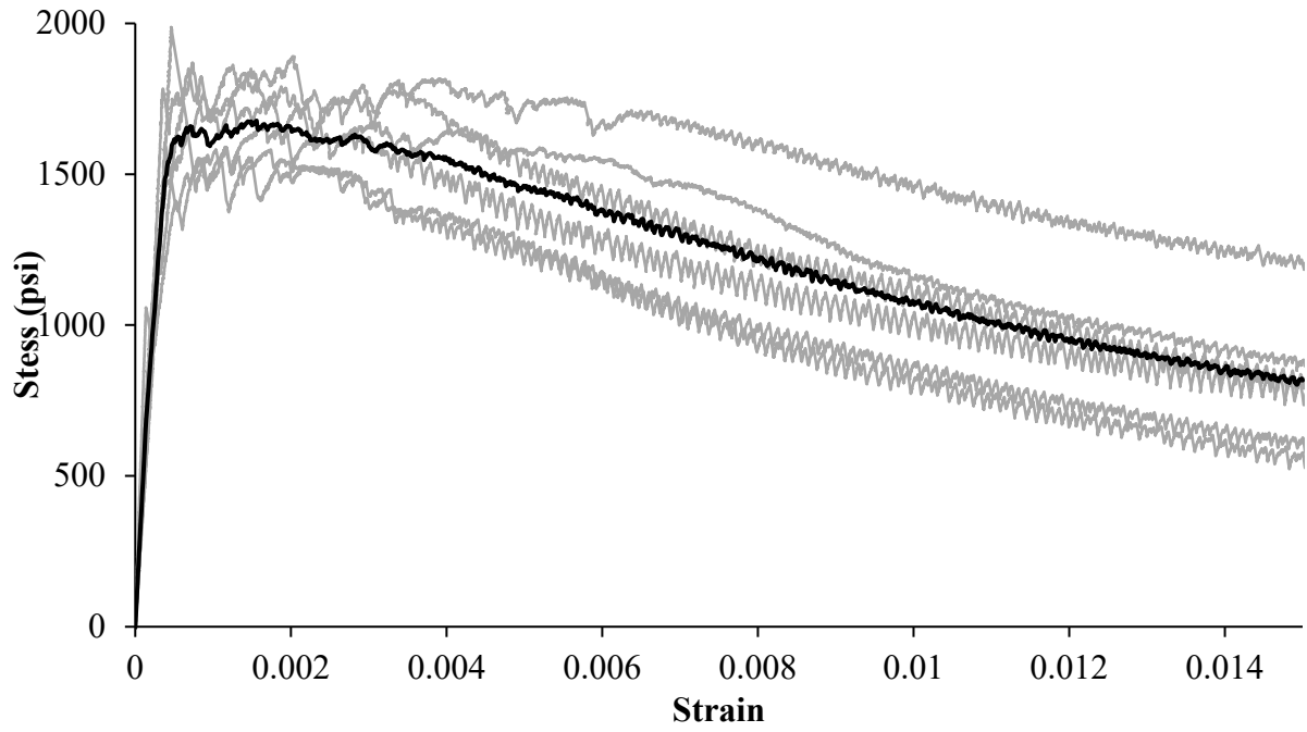
Figure B-12: 21+ Steam direct tension results
