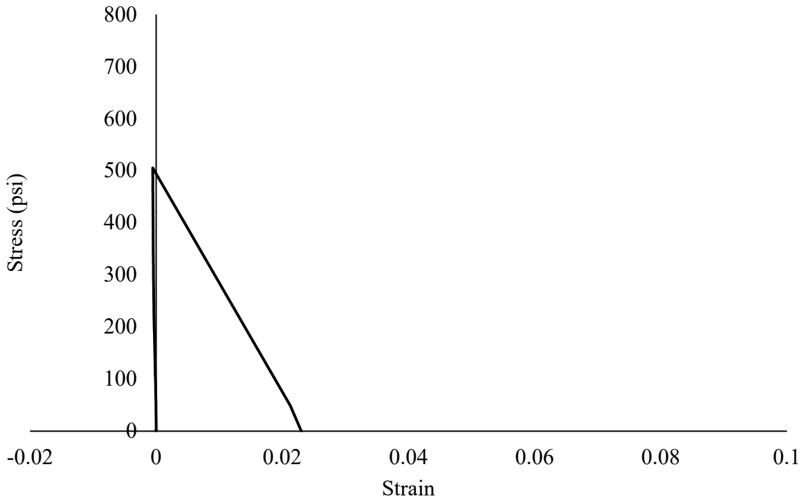
Figure 87: Stress vs. strain data for a specimen failure in the bottom concrete layer
