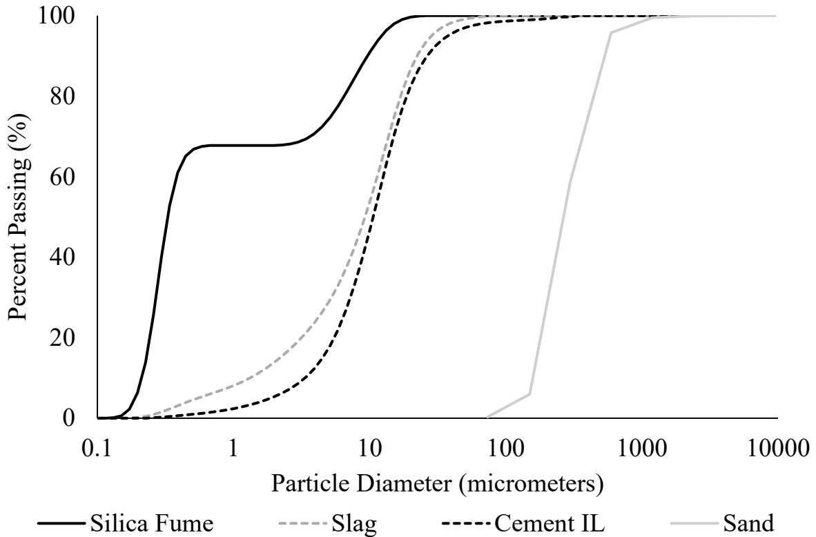
Figure 80: Particle size analysis of materials
