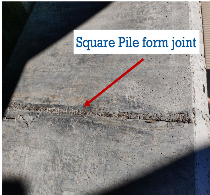
Figure 229: Photograph of concrete at location of form joint
