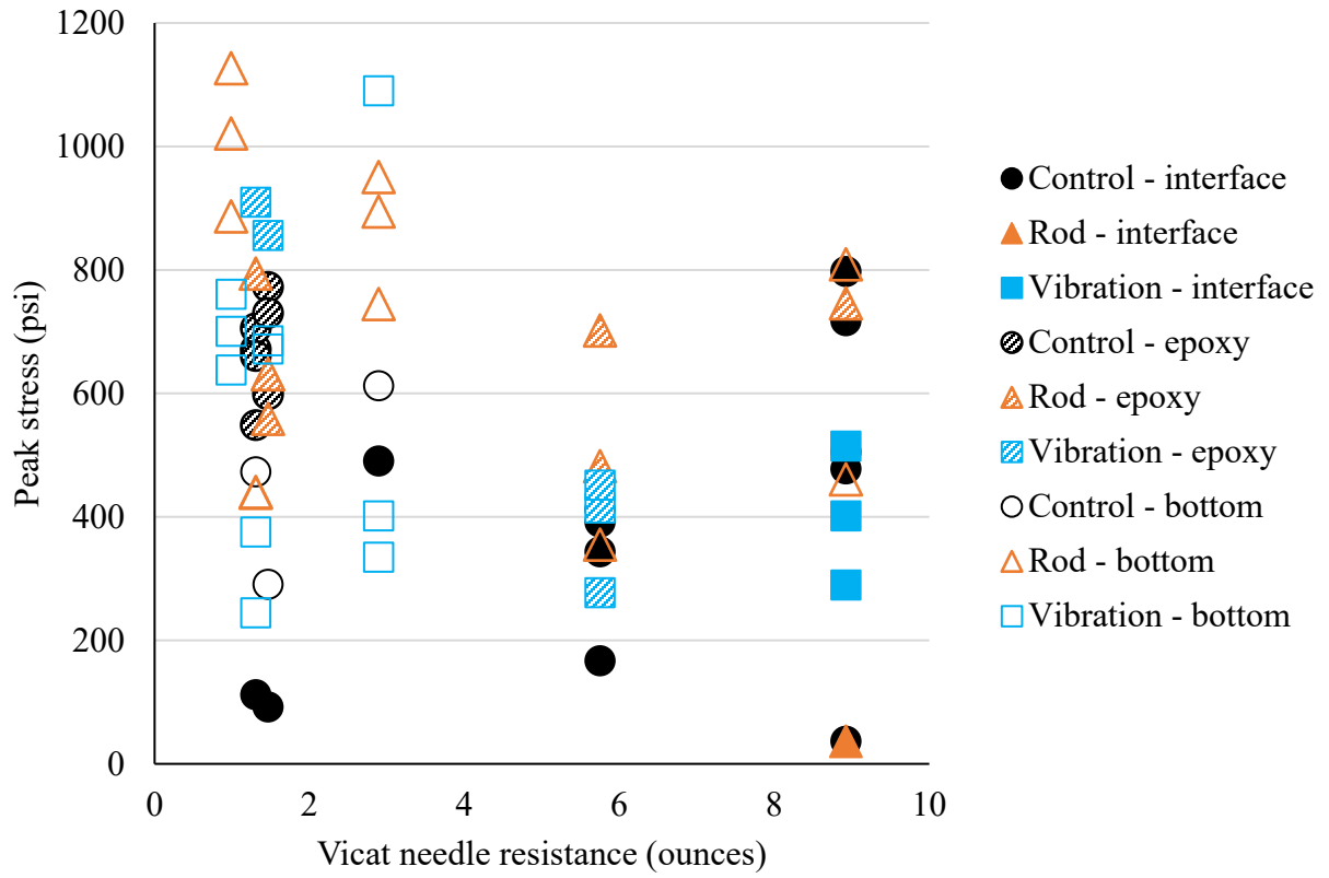
Figure 90: Core peak stress vs. first layer stiffness
