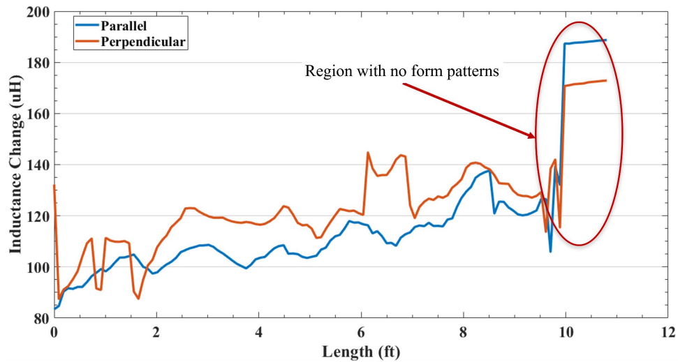
Figure 233: The form pattern on the surface of an octagonal pile and the corresponding inductance changes
