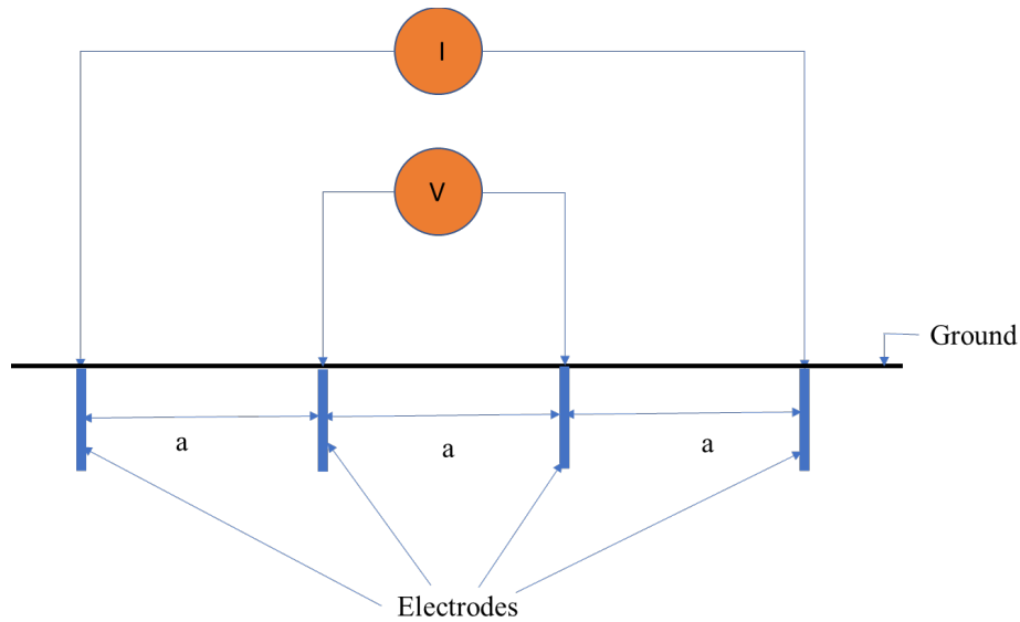
Figure 20: Wenner method
