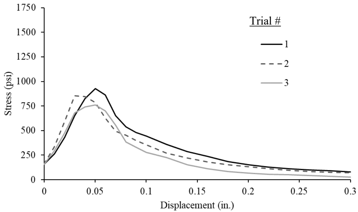
Figure A-10: Double-punch results for 3% twisted fiber specimens
