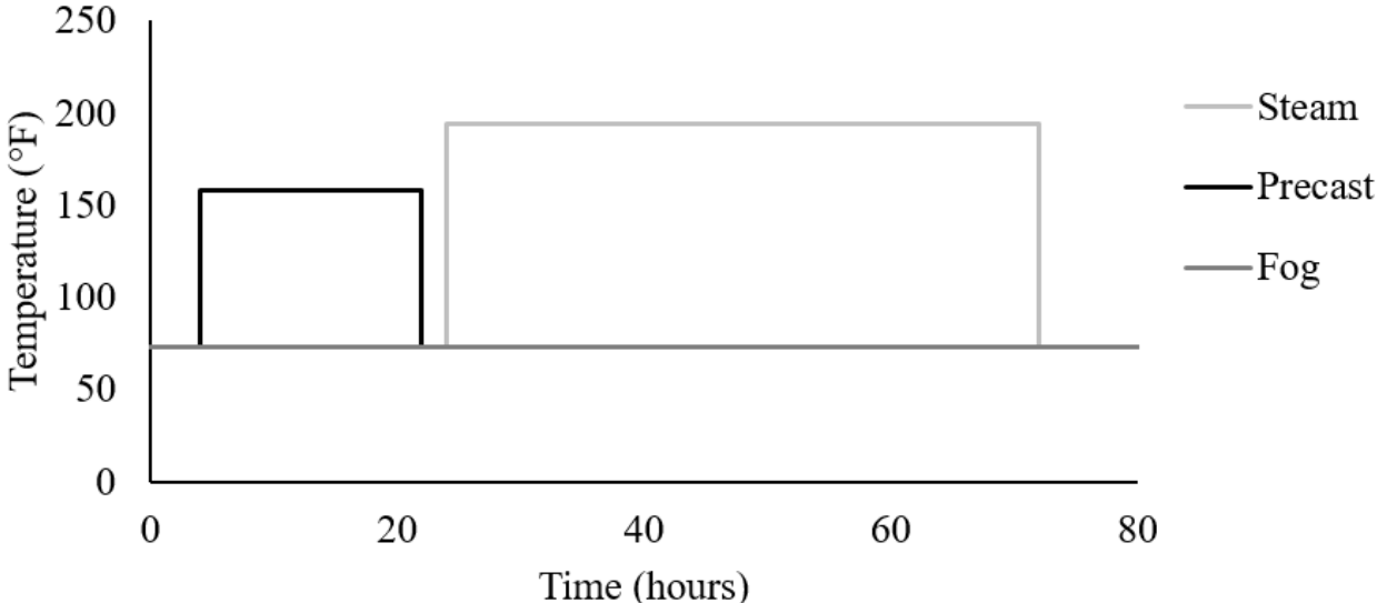
Figure 46: Curing temperatures for first three days
