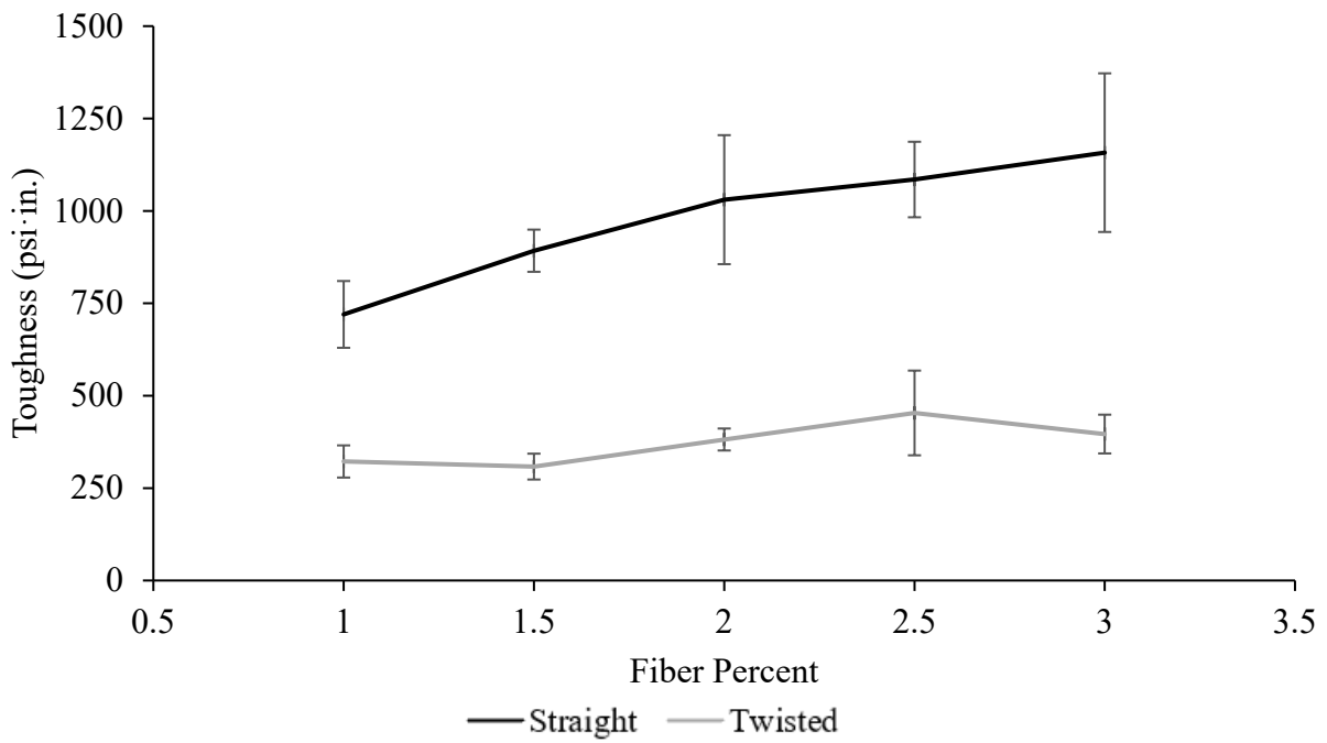
Figure 31: Average toughness from ASTM C1609 flexural testing
