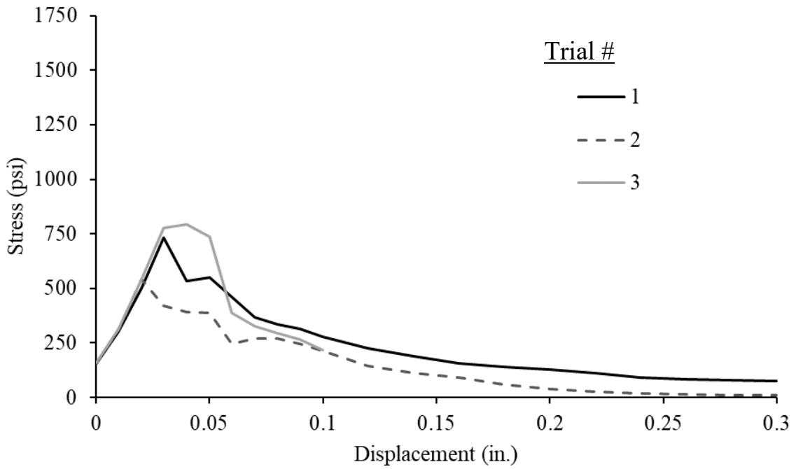
Figure A-6: Double-punch results for 1% twisted fiber specimens
