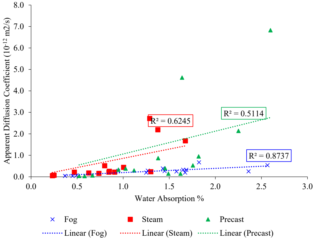
Figure 192: Water absorption vs chloride diffusion for all samples including fibers
