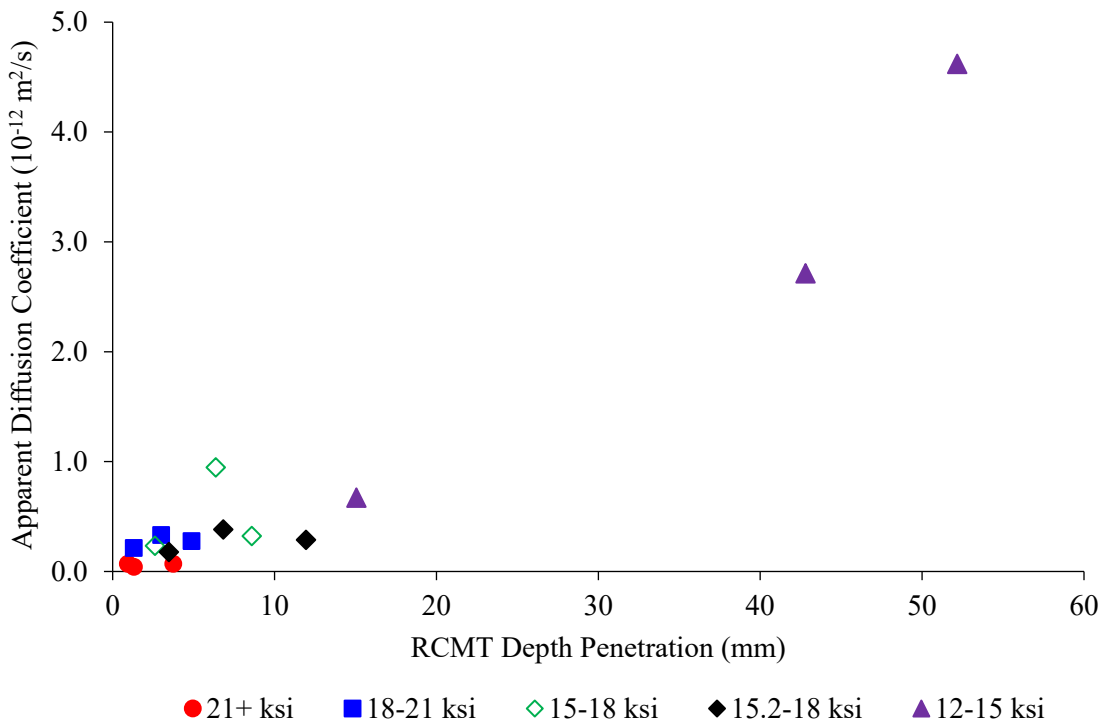
Figure 184: 7-day RCM testing for samples without fibers vs chloride diffusion coefficient
