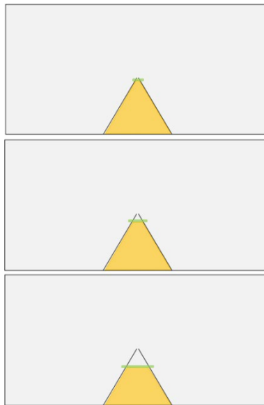
Figure 9. Example of Target Speed Predictor (green bar) and Headway (yellow) symbols as the locomotive approaches the target
