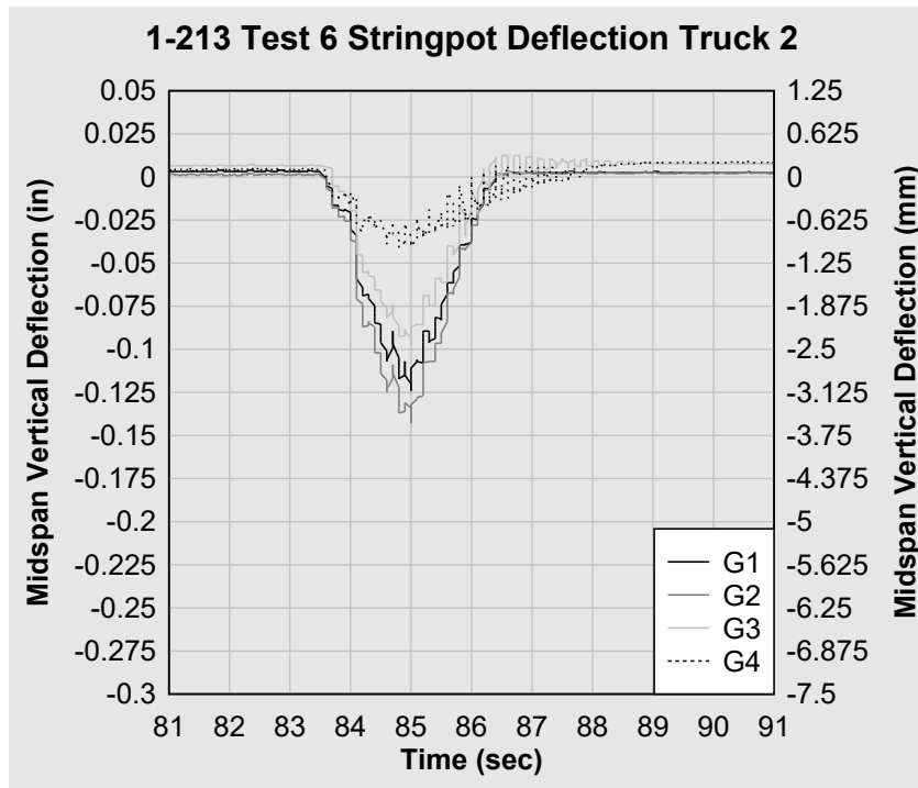
Figure 46. 1-213 Test 6 string pot truck 2 midspan deflection.
