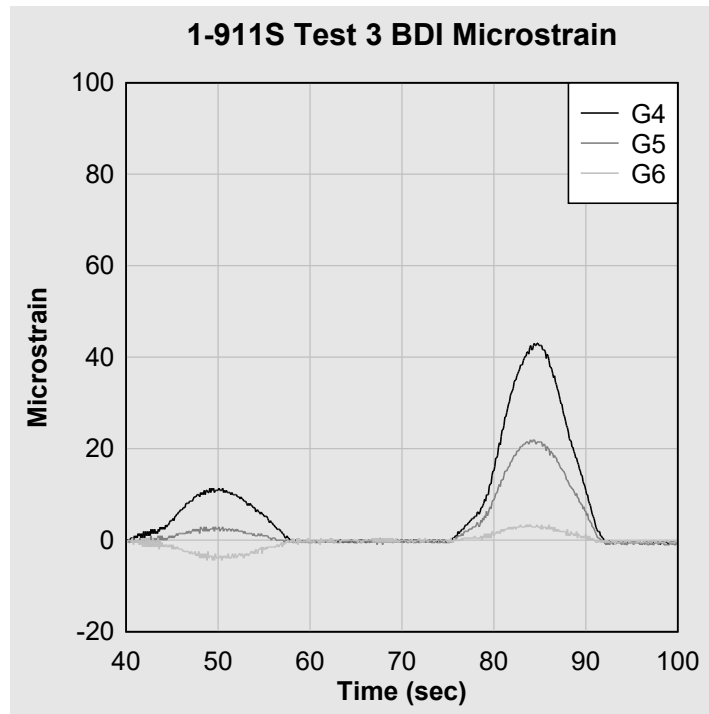
Figure 21. 1-911S Test 3 midspan bottom flange BDI microstrain.
