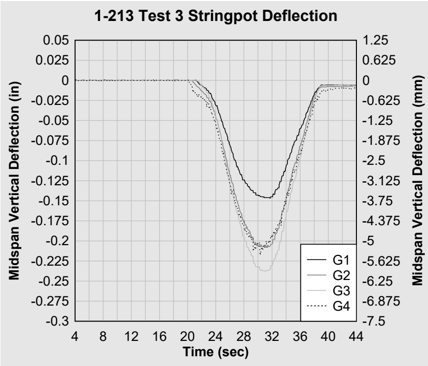
Figure 31. 1-213 Test 3 string pot midspan deflection.
