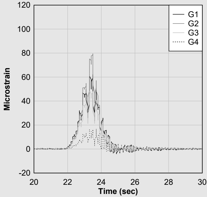
Figure 47. 1-213 Test 5 truck 1 midspan bottom flange BDI microstrain.
