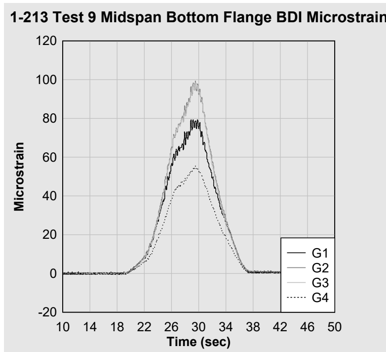
Figure 38. 1-213 Test 9 midspan bottom flange BDI microstrain.
