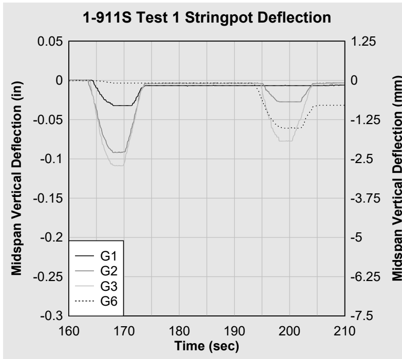
Figure 12. 1-911S Test 1 string pot midspan deflection.
