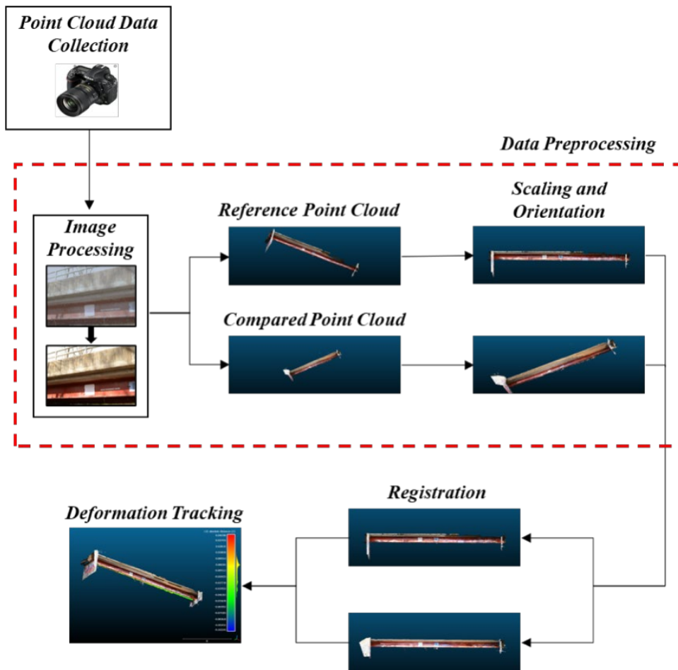
Figure 2. Overview of point cloud analysis methodology.
