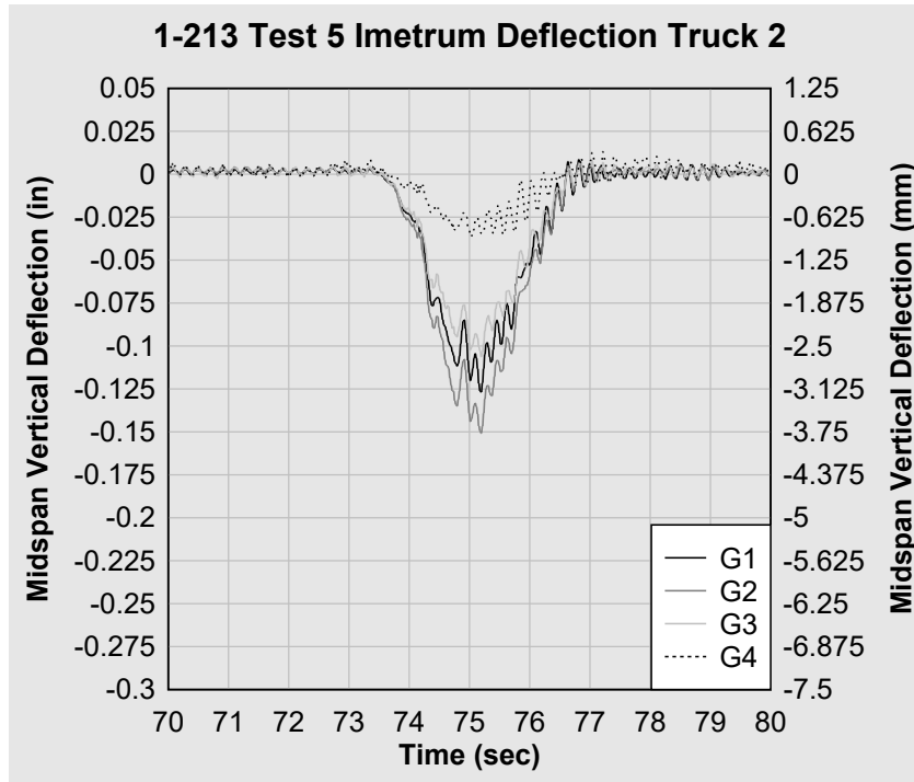
Figure 41. 1-213 Test 5 Imetrum truck 2 midspan deflection.
