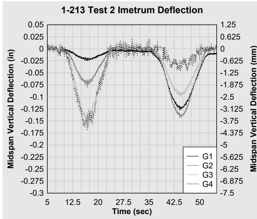
Figure 26. 1-213 Test 2 Imetrum midspan deflection.
