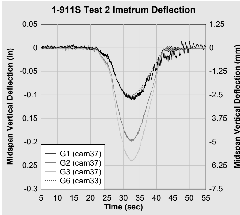
Figure 13. 1-911S Test 2 Imetrum midspan deflection.
