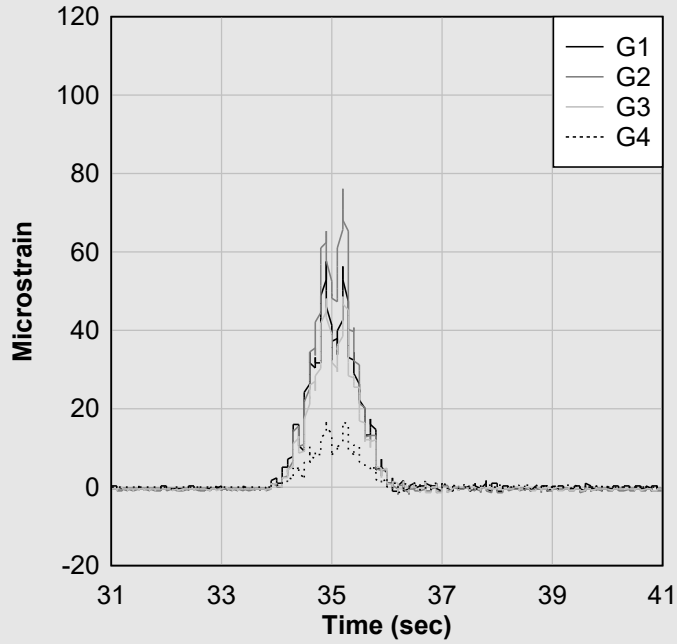
Figure 49. 1-213 Test 6 truck 1 midspan bottom flange BDI microstrain.
