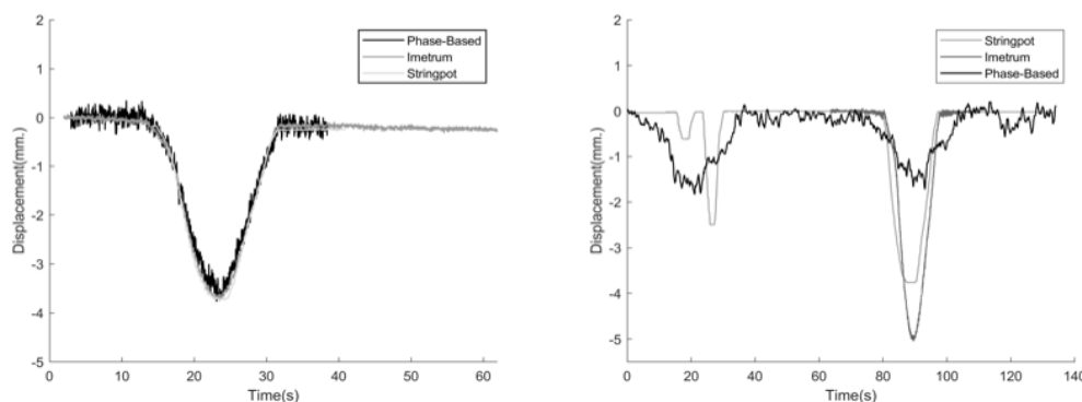
Figure 23. Comparison of measurement methods: (a) strong correlation of results for fascia girder nearest to the phase-based camera and (b) inaccurate results for the phase-based approach, for girder farther away from camera.
