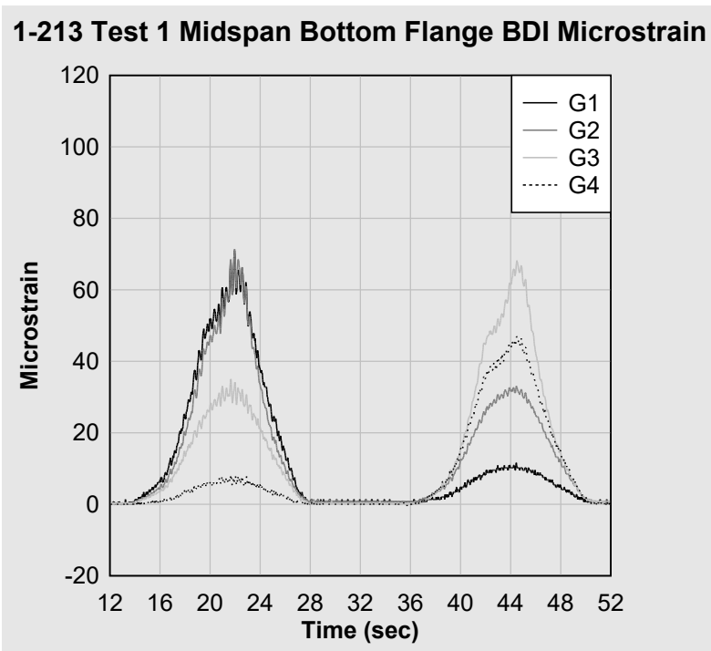
Figure 28. 1-213 Test 1 midspan bottom flange BDI microstrain.
