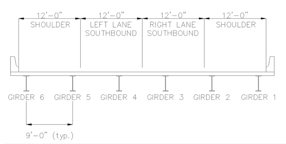
Figure 4. Bridge 1-911S cross-sectional view.
