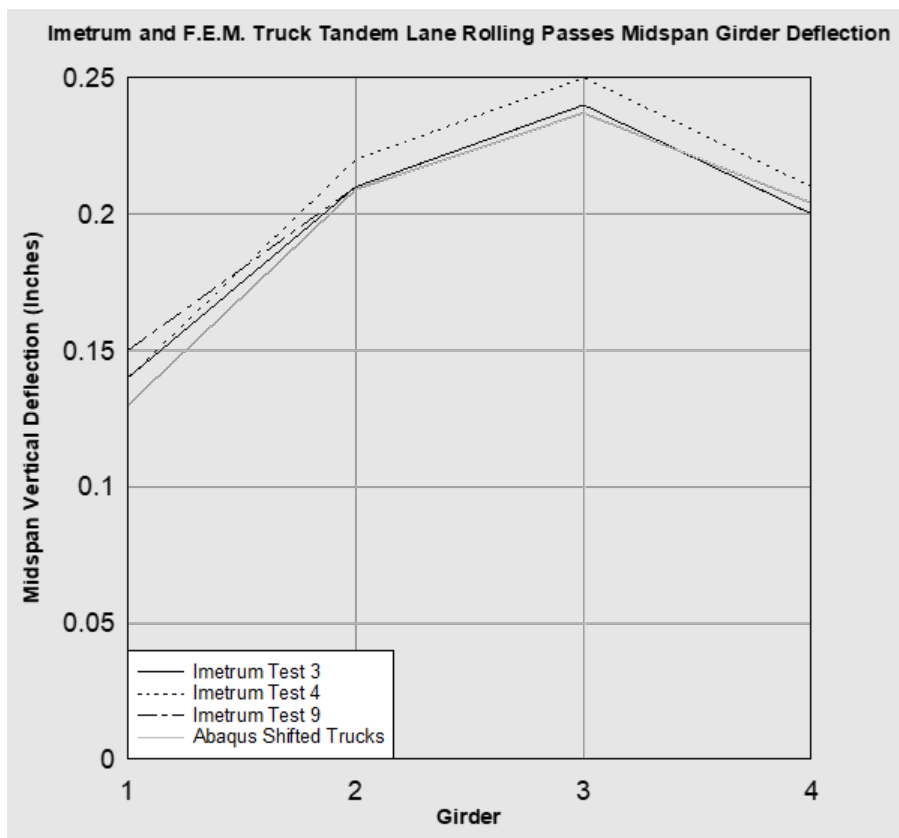
Figure 70. 1-213 Imetrum and F.E.M. truck tandem lane rolling passes midspan girder deflection.
