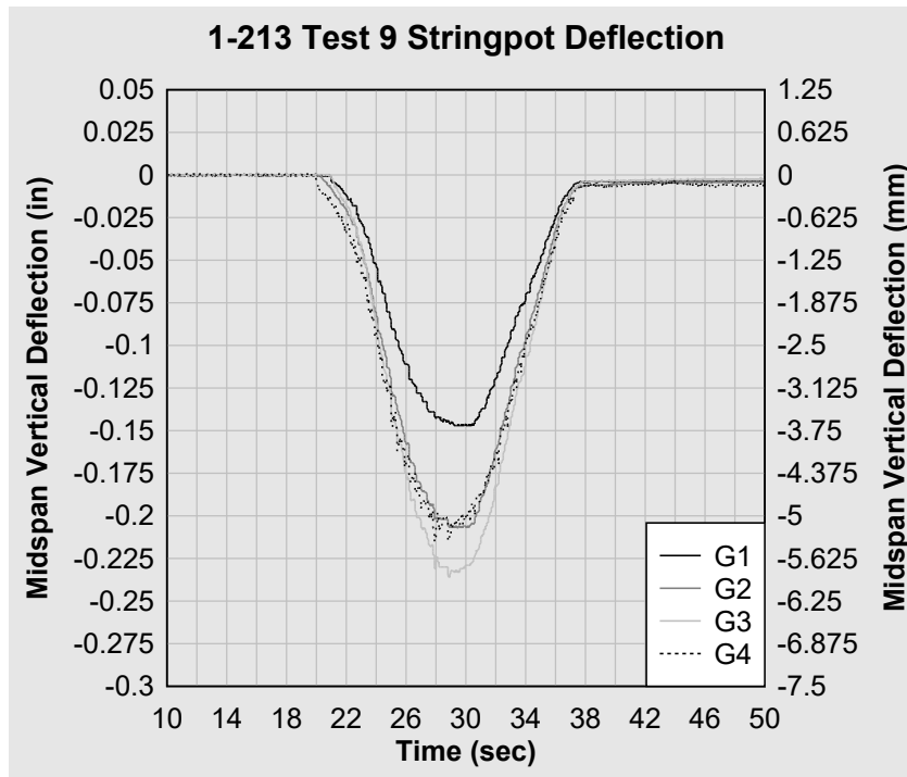
Figure 35. 1-213 Test 9 string pot midspan deflection.
