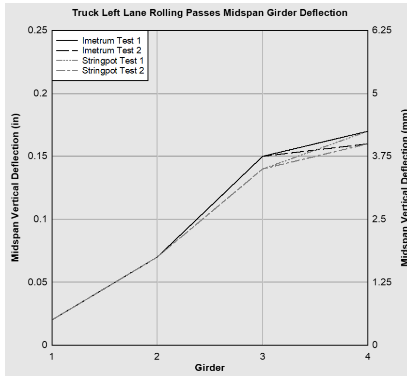
Figure 57. 1-213 Test truck left lane rolling passes midspan girder deflection.
