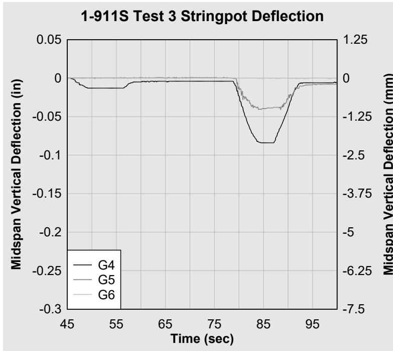
Figure 18. 1-911S Test 3 string pot midspan deflection.
