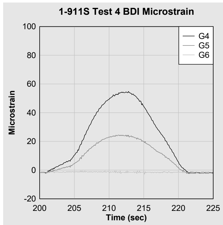
Figure 22. 1-911S Test 4 midspan bottom flange BDI microstrain.
