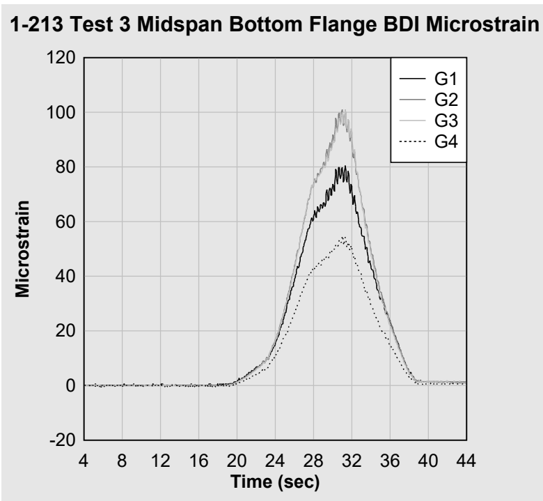
Figure 36. 1-213 Test 3 midspan bottom flange BDI microstrain.
