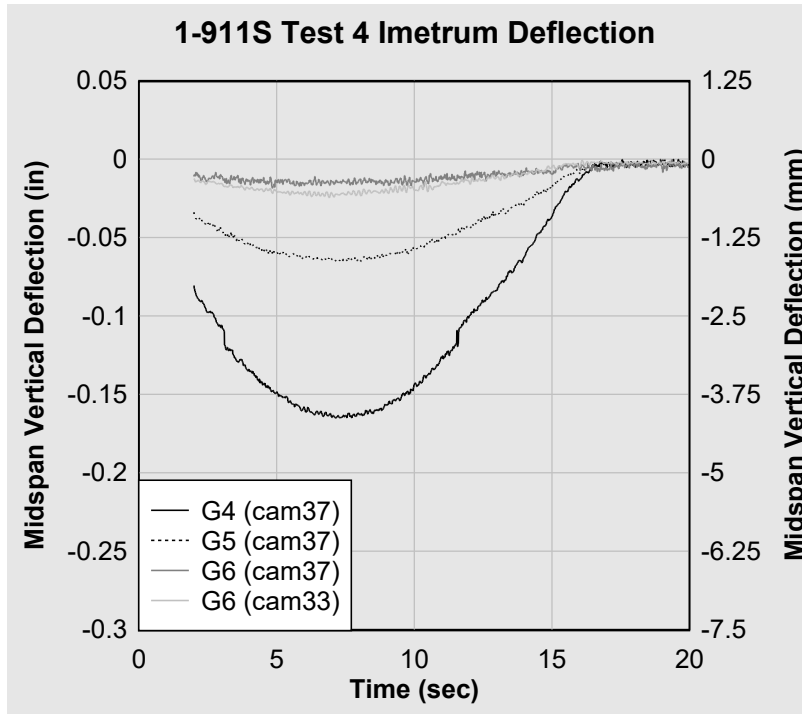
Figure 19. 1-911S Test 4 Imetrum midspan deflection.
