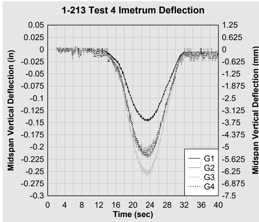
Figure 32. 1-213 Test 4 Imetrum midspan deflection.
