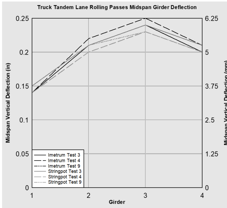
Figure 59. 1-213 Truck tandem lane rolling passes midspan girder deflection.
