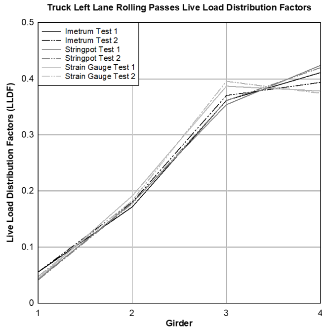
Figure 63. 1-213 Truck left lane rolling passes live load distribution factors.
