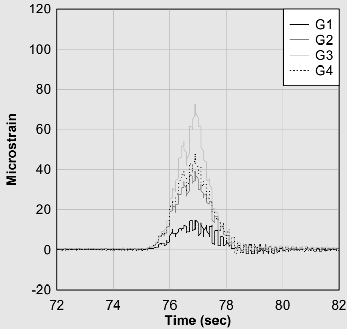
Figure 48. 1-213 Test 5 truck 2 midspan bottom flange BDI microstrain.
