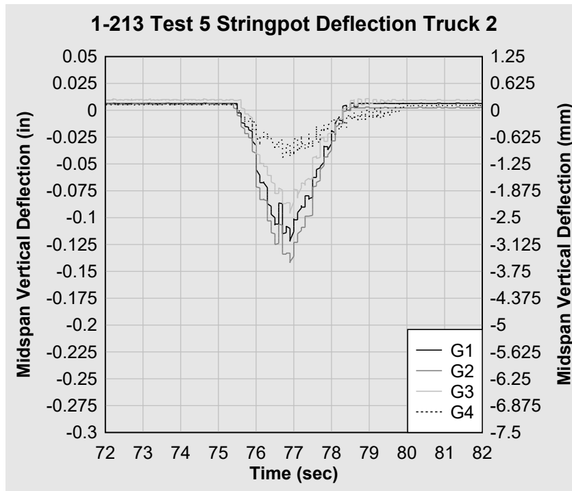
Figure 42. 1-213 Test 5 string pot truck 2 midspan deflection.
