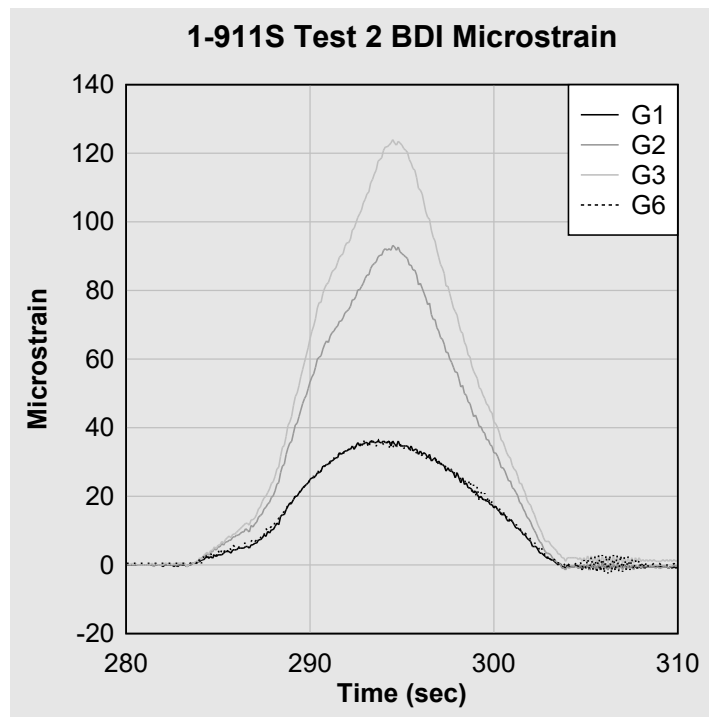
Figure 16. 1-911S Test 2 midspan bottom flange BDI microstrain.
