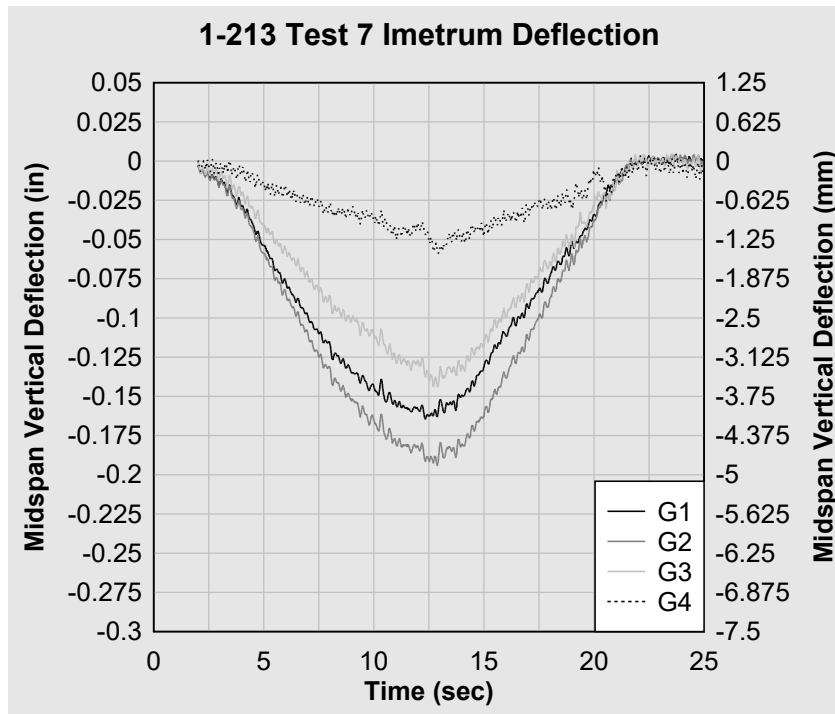
Figure 51. 1-213 Test 7 Imetrum midspan deflection.
