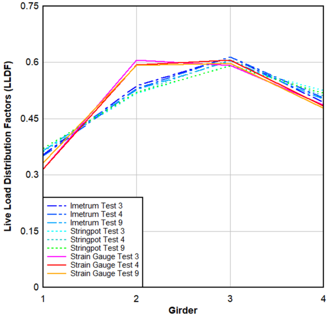
Figure 65. 1-213 Truck tandem lane rolling passes live load distribution factors.
