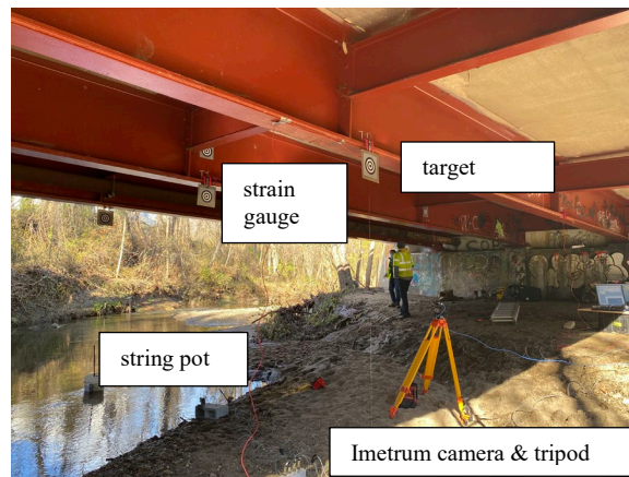
Figure 1. Overview of instrumentation placement under bridge.
