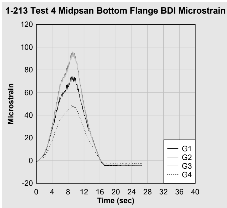
Figure 37. 1-213 Test 4 midspan bottom flange BDI microstrain.
