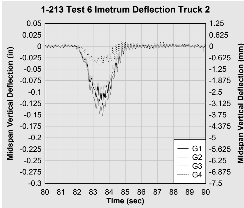
Figure 45. 1-213 Test 6 Imetrum truck 2 midspan deflection.
