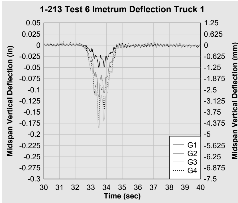
Figure 43. 1-213 Test 6 Imetrum truck 1 midspan deflection.
