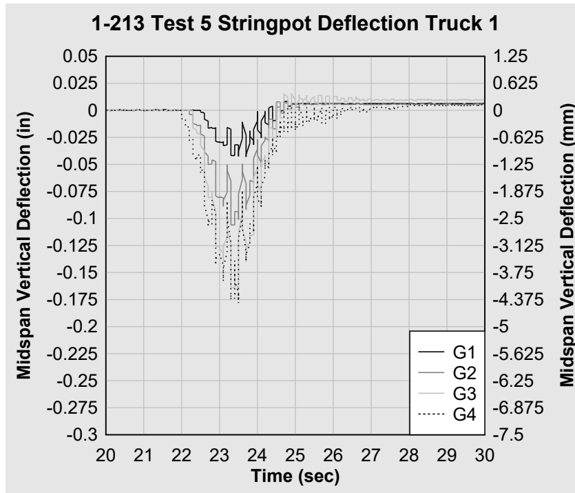
Figure 40. 1-213 Test 5 string pot truck 1 midspan deflection.
