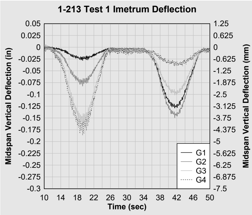
Figure 24. 1-213 Test 1 Imetrum midspan deflection.
