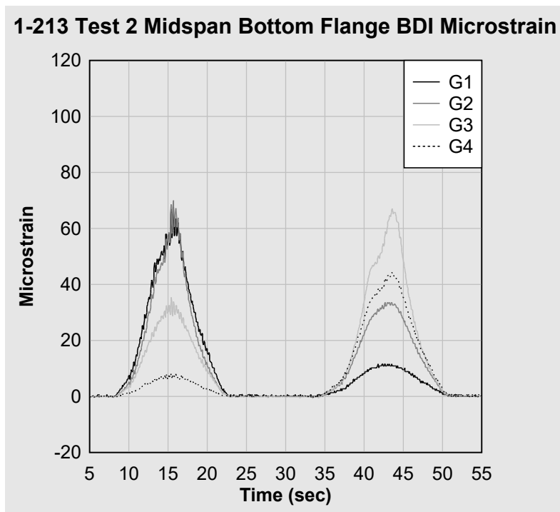
Figure 29. 1-213 Test 2 midspan bottom flange BDI microstrain.
