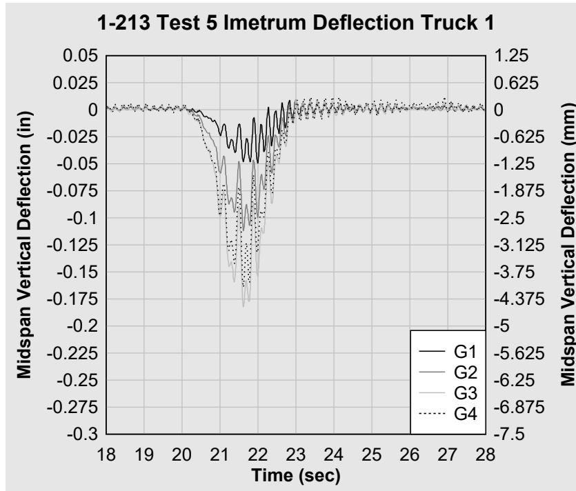
Figure 39. 1-213 Test 5 Imetrum truck 1 midspan deflection.
