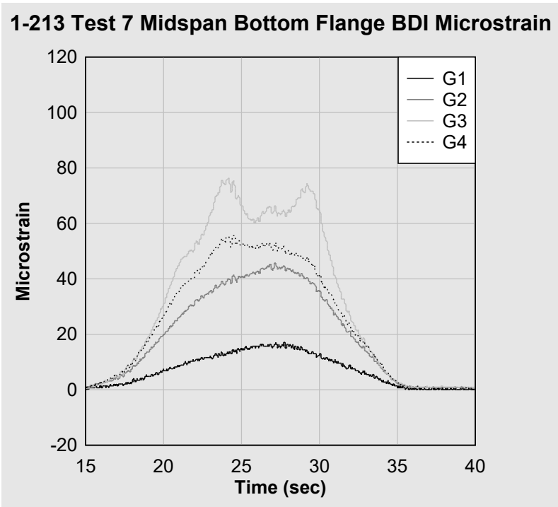
Figure 55. 1-213 Test 7 midspan bottom flange BDI microstrain.
