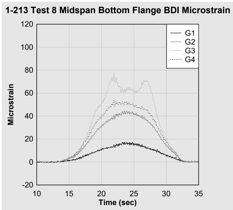
Figure 56 1-213 Test 8 midspan bottom flange BDI microstrain.
