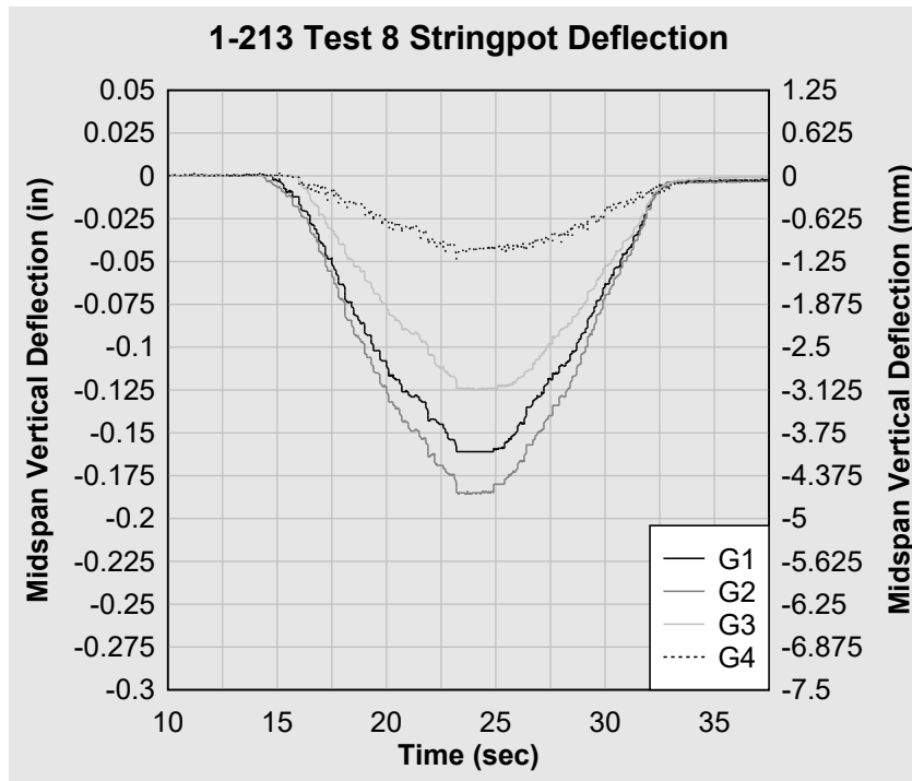
Figure 54. 1-213 Test 8 string pot midspan deflection.
