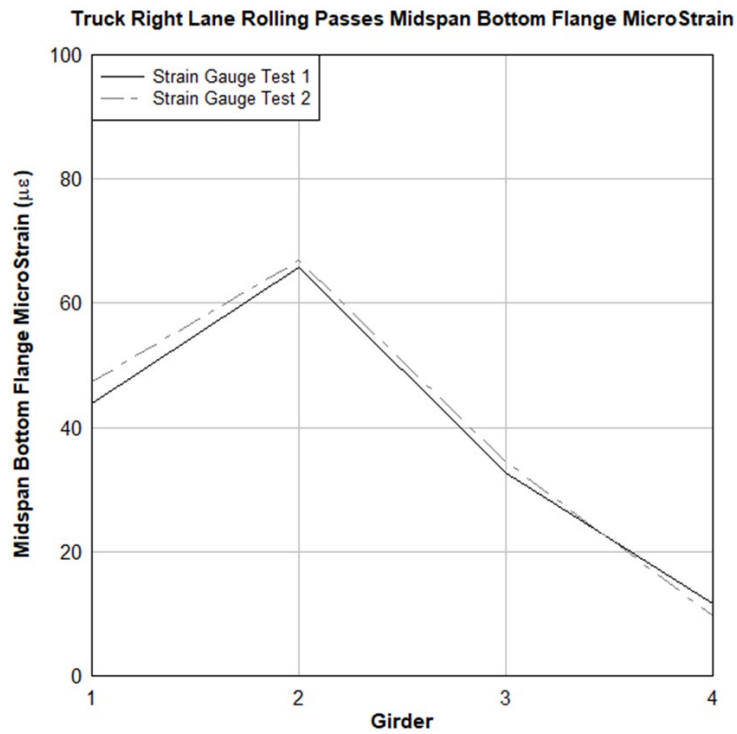
Figure 61. 1-213 Truck right lane rolling passes midspan bottom flange microstrain.
