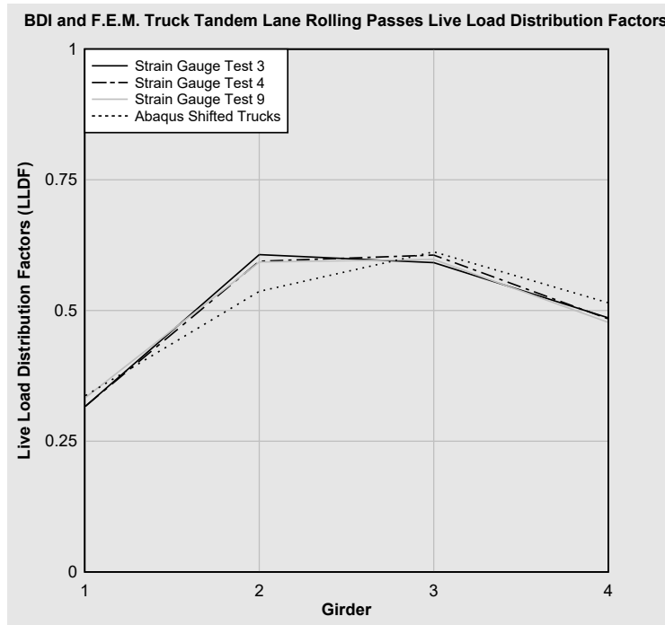
Figure 73. 1-213 Imetrum and F.E.M. truck tandem lane rolling passes strain live load distribution factors.
