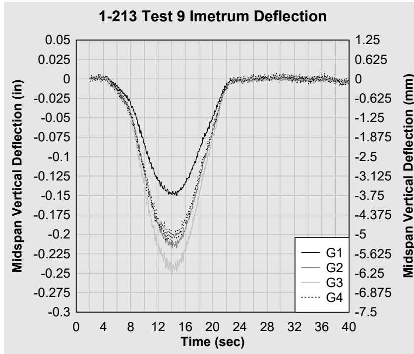
Figure 34. 1-213 Test 9 Imetrum midspan deflection.
