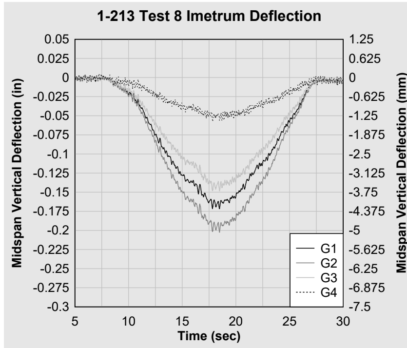
Figure 53. 1-213 Test 8 Imetrum midspan deflection.
