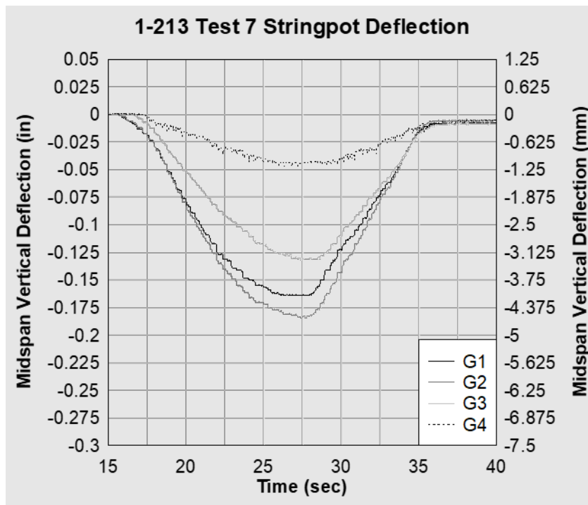
Figure 52. 1-213 Test 7 string pot midspan deflection.
