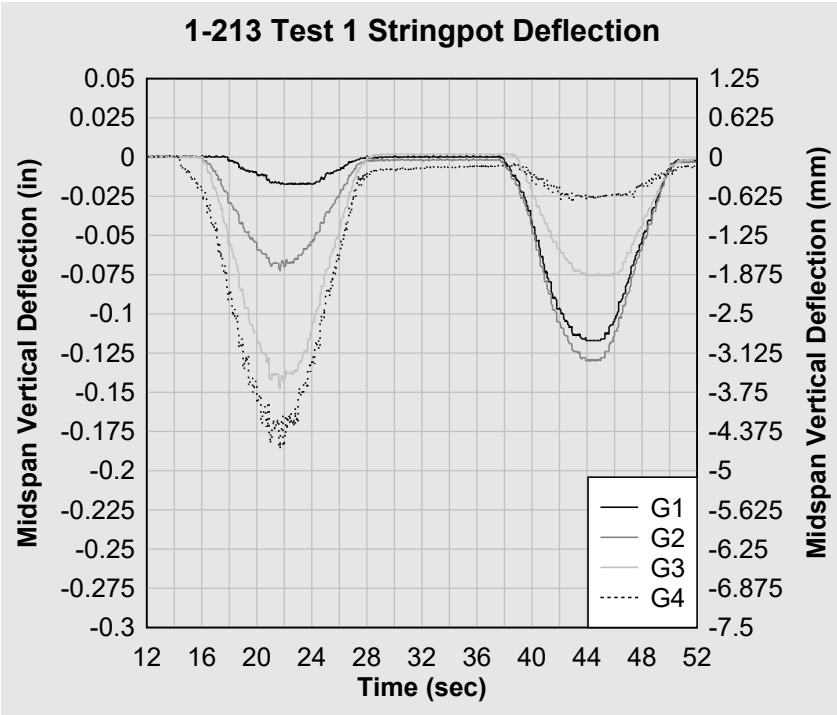
Figure 25. 1-213 Test 1 string pot midspan deflection.
