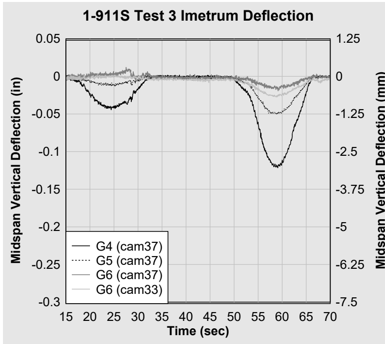
Figure 17. 1-911S Test 3 Imetrum midspan deflection.
