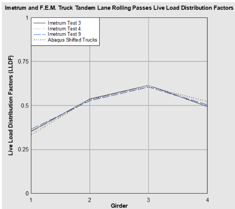
Figure 72. 1-213 Imetrum and F.E.M. truck tandem lane rolling passes deflection live load distribution factors.
