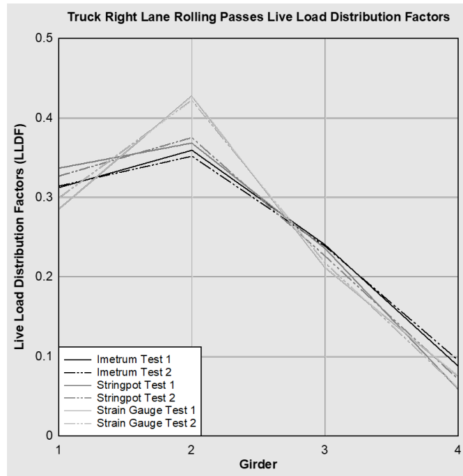
Figure 64. 1-213 Truck right lane rolling passes live load distribution factors.
