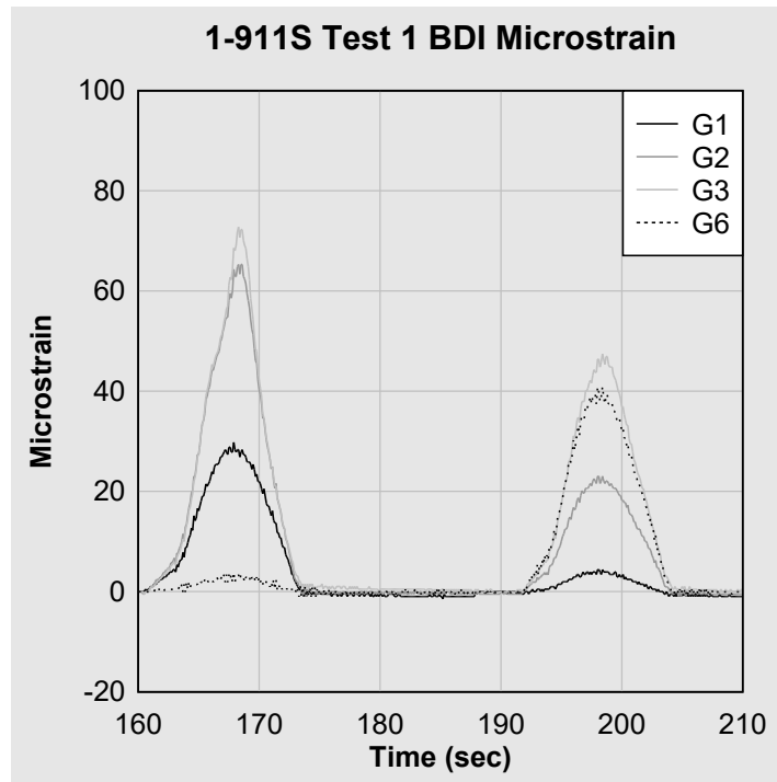
Figure 15. 1-911S Test 1 midspan bottom flange BDI microstrain.
