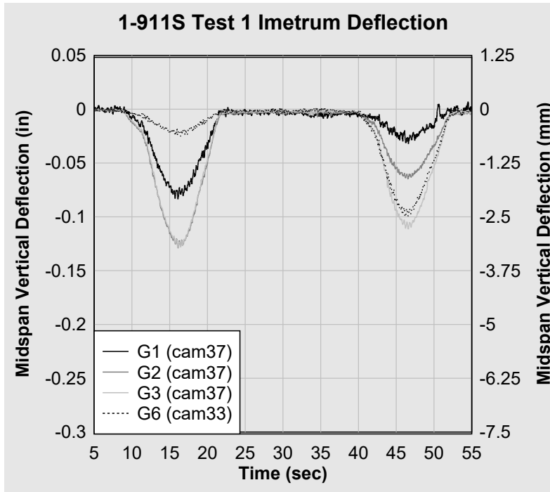
Figure 11. 1-911S Test 1 Imetrum midspan deflection.
