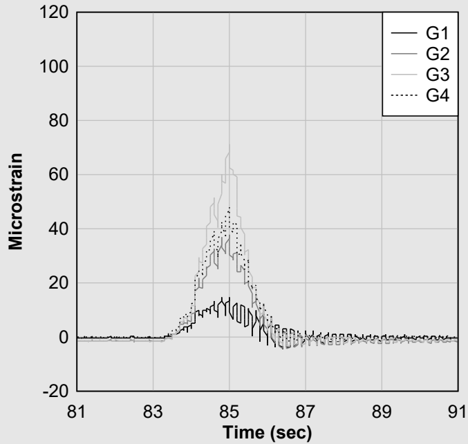
Figure 50. 1-213 Test 6 truck 2 midspan bottom flange BDI microstrain.
