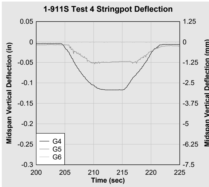
Figure 20. 1-911S Test 4 string pot midspan deflection.
