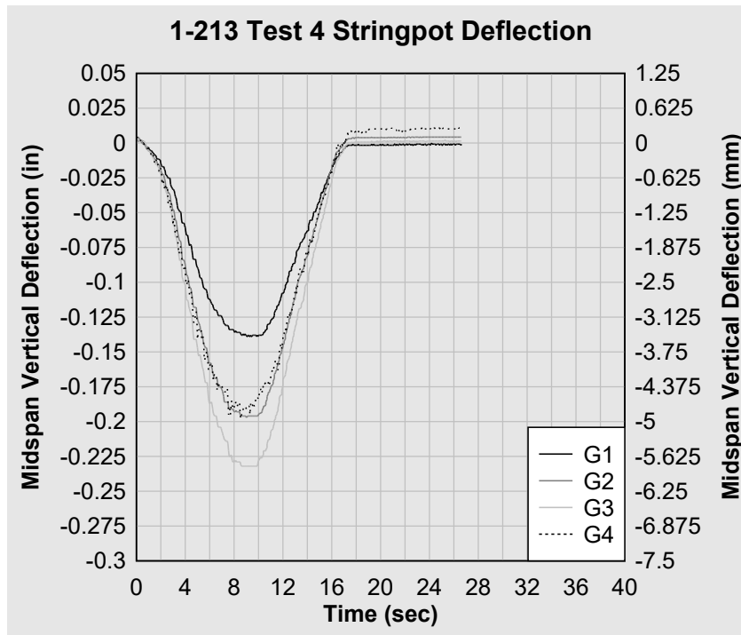
Figure 33. 1-213 Test 4 string pot midspan deflection.
