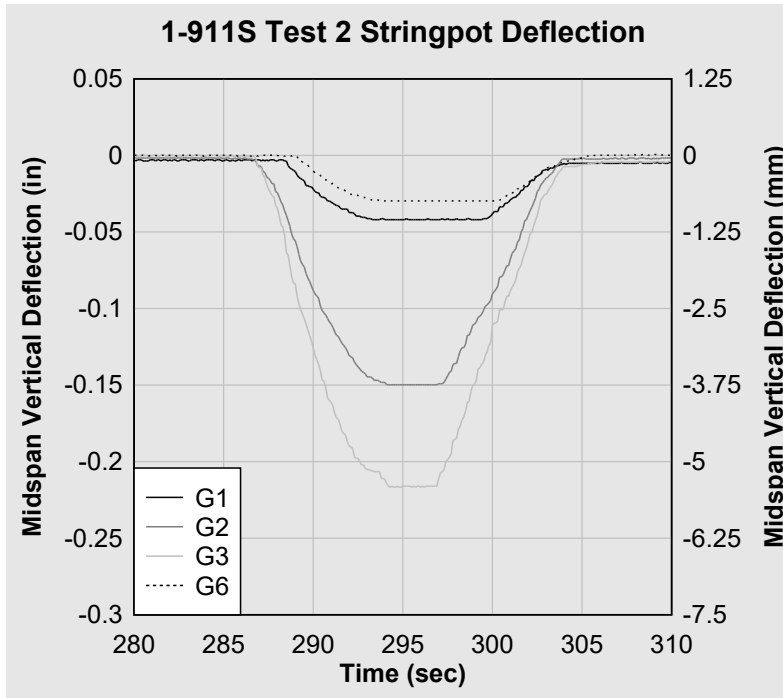
Figure 14. 1-911S Test 2 string pot midspan deflection.
