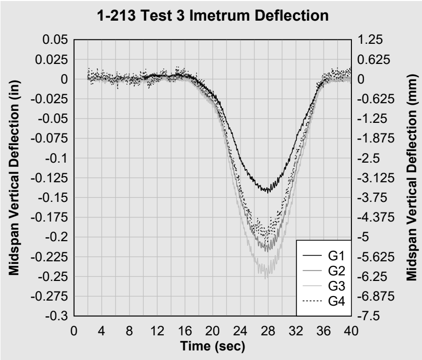
Figure 30. 1-213 Test 3 Imetrum midspan deflection.
