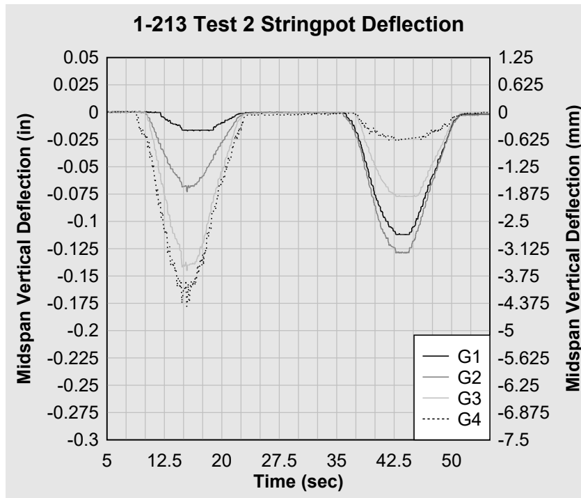
Figure 27. 1-213 Test 2 string pot midspan deflection.
