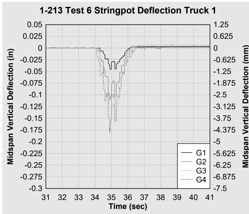
Figure 44. 1-213 Test 6 string pot truck 1 midspan deflection.
