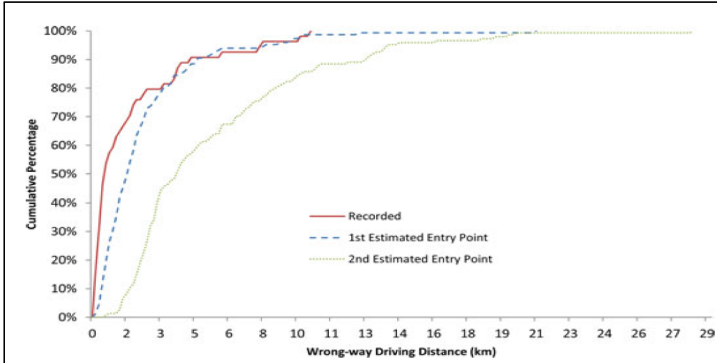
Figure 1. Cumulative distribution of distances between WWD crash locations and entry points estimated based on either the closest interchange locations or police reports of crashes (3)
