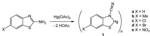
Scheme 1 Synthesis of [Hg(ocap)] n ( 1a–e ) upon dehydrogenative ring-opening of 2-aminobenzothiazoles upon addition of Hg(OAc) 2 .
