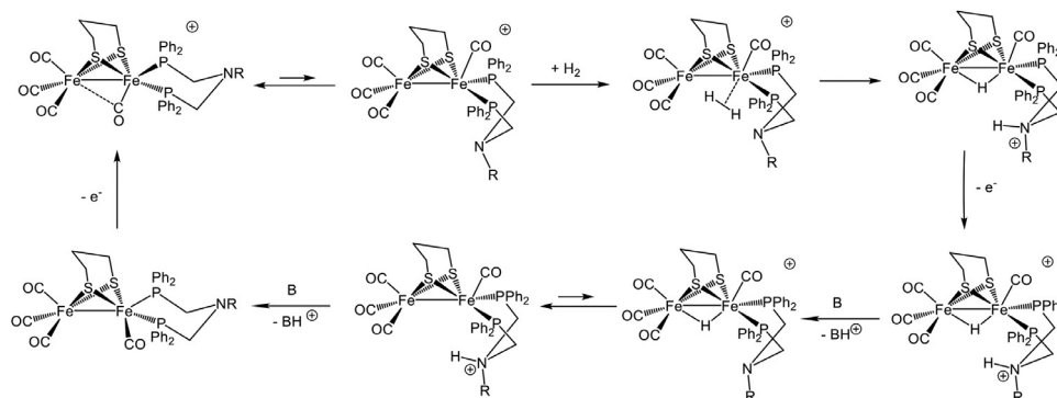
Scheme 5. Simplified version of the \text{H}_2 oxidation mechanism ( R = \text{Pr} ) proposed by Ahlquist and co-workers [13–15].
