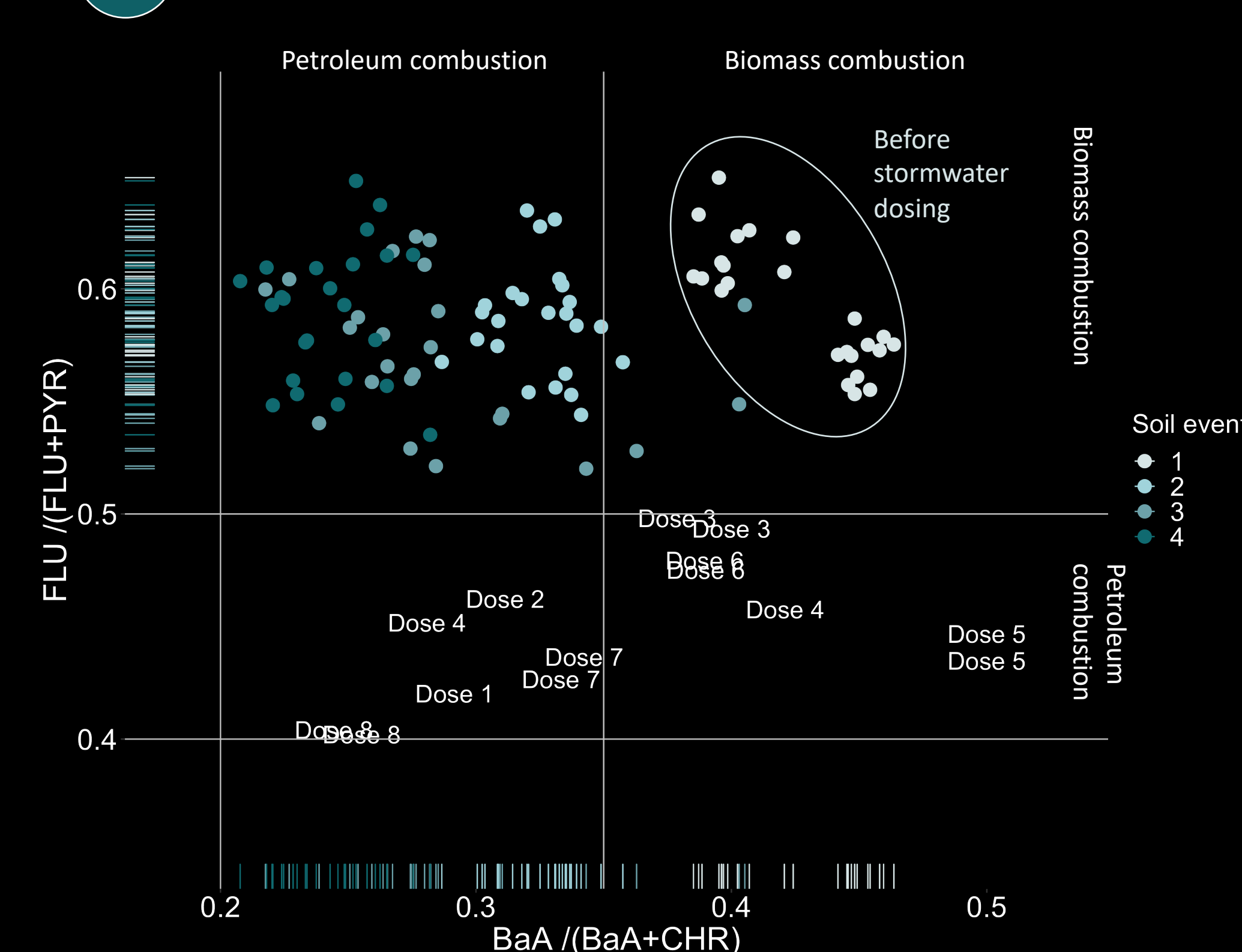
Figure 2. Diagnostic ratios of benzo(a)anthracene/chrysene and fluoranthene and pyrene for soil samples taken across 4 soil sampling events (points) and for influent samples across all dosing events (text). Duplicate influent samples are plotted.
