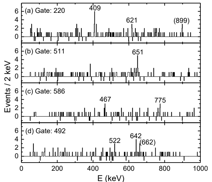
FIG. 3. Examples of \gamma - \gamma coincidence analyses when tagging with the proton decay of ^{147m}\text{Tm} , and setting a gate on the \gamma -ray energy as indicated.
