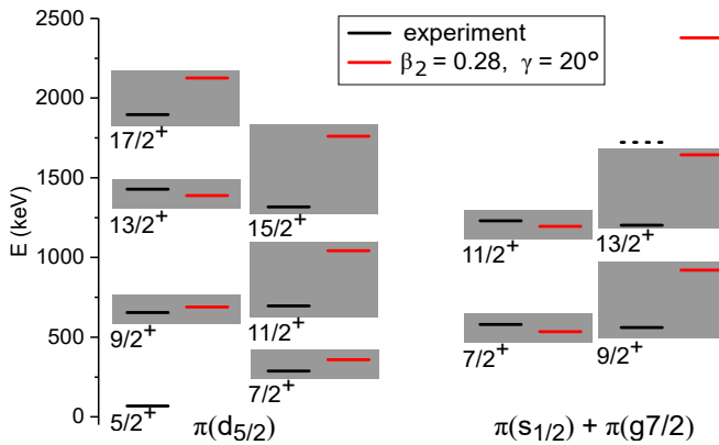
FIG. 6. Comparison of the measured level energies above the proton-decaying 5/2^+ state to those calculated using the nonadiabatic quasiparticle model. The gray boxes are to group similar states.
