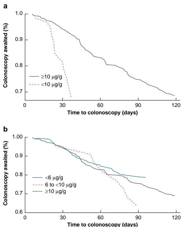
Fig. 3 Kaplan–Meier curves
