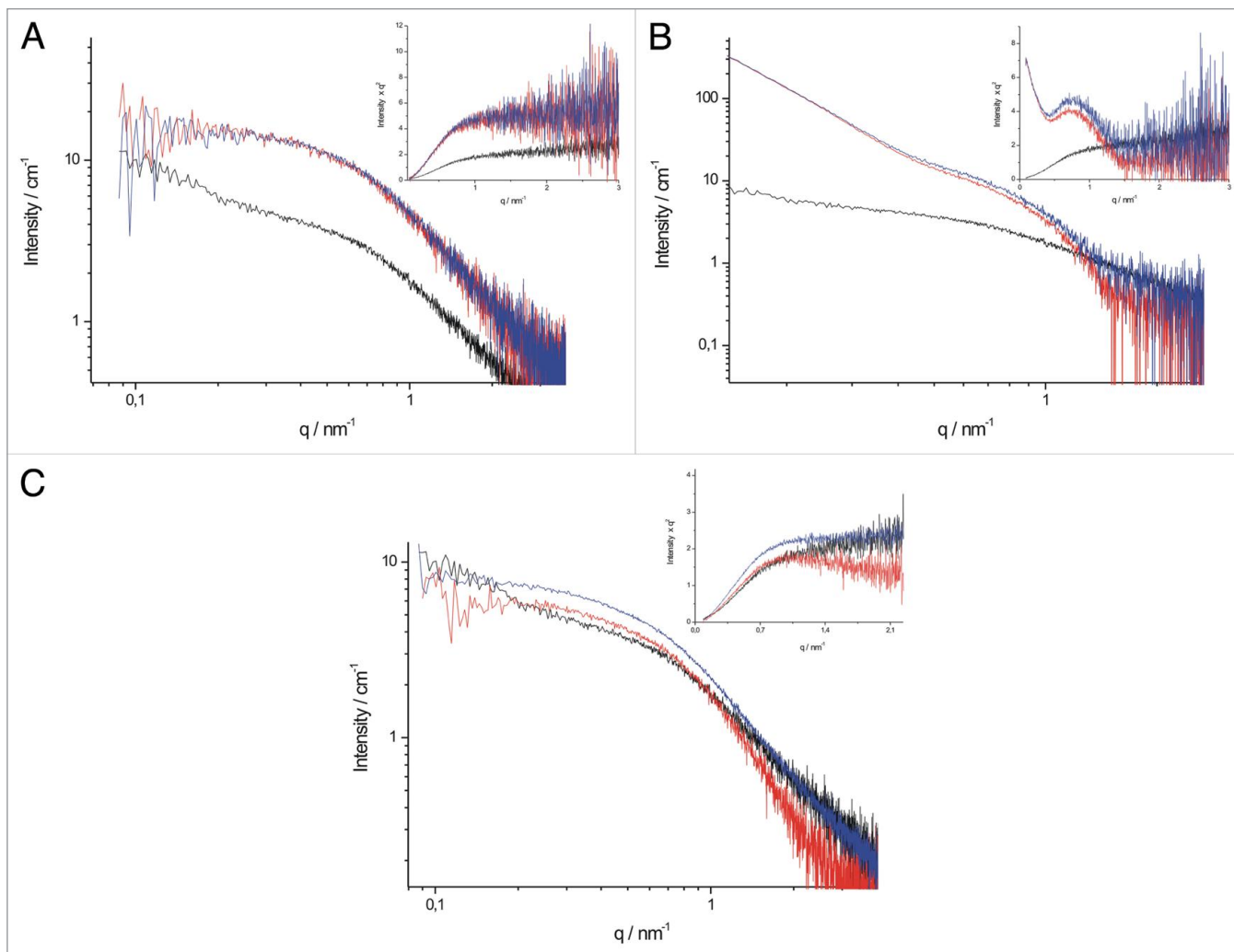
Figure 7. SAXS scattering curves and Kratky plots of T \beta 4 and its partners. (A) scattering curves of PINCH LIM4–5 in the absence of T \beta 4 (red), T \beta 4 in the absence of PINCH LIM4–5 (black) and PINCH LIM4–5 in the presence of T \beta 4 (blue). Inset: Kratky plot of PINCH LIM4–5, T \beta 4 and their complexes. Labeling is the same as in (A) . (B) scattering curves of ILK-Ank-GST in the absence of T \beta 4 (red), T \beta 4 in the absence of ILK-Ank-GST (black) and ILK-Ank-GST in the presence of T \beta 4 (blue). Inset: Kratky plot of ILK-Ank-GST, T \beta 4 and their complex. Labeling is the same as in (B) . (C) scattering curves of stabilin CTD in the absence of T \beta 4 (red), T \beta 4 in the absence of stabilin CTD (black) and stabilin CTD in the presence of T \beta 4 (blue). Inset: Kratky plot of stabilin CTD, T \beta 4 and their complex. Labeling is the same as in (C) .
