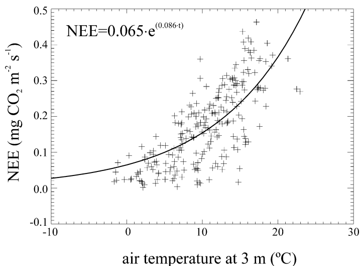
Fig. 3. Average night-time \text{CO}_2 efflux as a function of the average night-time air temperature measured at 3 m ( t ) for the growing period of the grassland. The fitted exponential curve is plotted as a solid line. The analytical form of the curve is also given.
