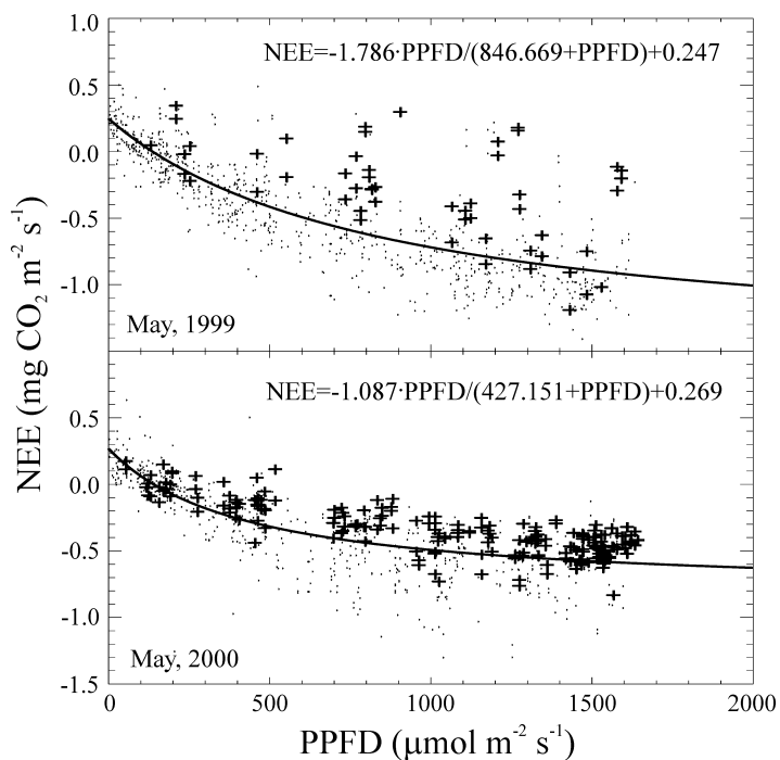
Fig. 2. Daytime NEE plotted against photosynthetically active photon flux density (PPFD) for May 1999 and May 2000. Negative NEE means \text{CO}_2 uptake by the ecosystem. Plus signs mark NEE measured at water vapor pressure deficit (VPD) greater than 1.5 kPa, dots mark NEE measured at VPD less than 1.5 kPa. The rectangular hyperbola function that was fitted to all monthly data is given for both months. ( 1 \text{ mg CO}_2 \text{ m}^{-2} \text{ s}^{-1} = 22.7 \mu\text{mol m}^{-2} \text{ s}^{-1} ).
