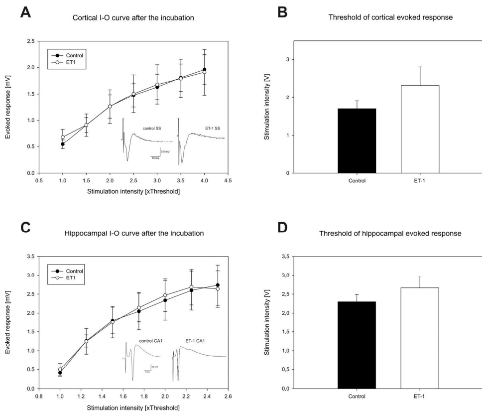
Fig. 2. ET-1 does not change the evoked responses nor the slope of the I-O curve in either hippocampal or cortical preparations ( A, C ). The threshold of evoked responses was not significantly increased in either region ( B, D ). These results indicate no significant effect of ET-1 on the excitability of the nervous tissue.
