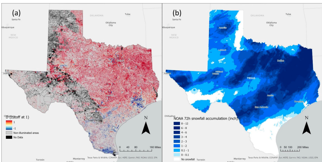
Figure 6. Comparison between NTL radiance change and snow accumulation: (a) spatial distribution of NTL radiance change ( D ), (b) snowfall accumulation from NOAA National Gridded Snowfall Analysis (72-hour snowfall accumulation) at 12:00 AM, Feb 16, 2021.
