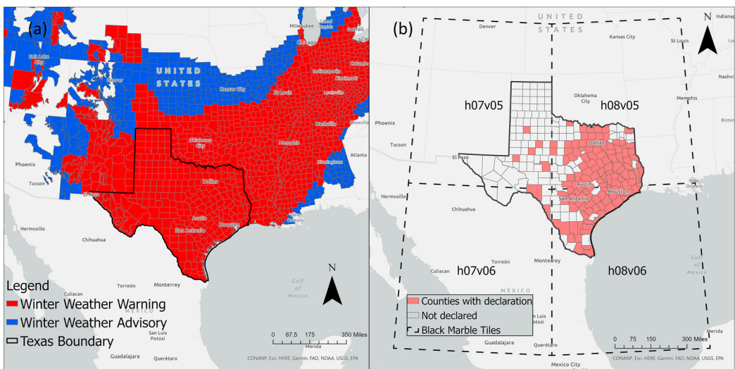
Figure 2. (a) National Weather Services (NWS) winter weather forecast near Texas, (b) counties that declared Winter Storm Uri as a major disaster.
