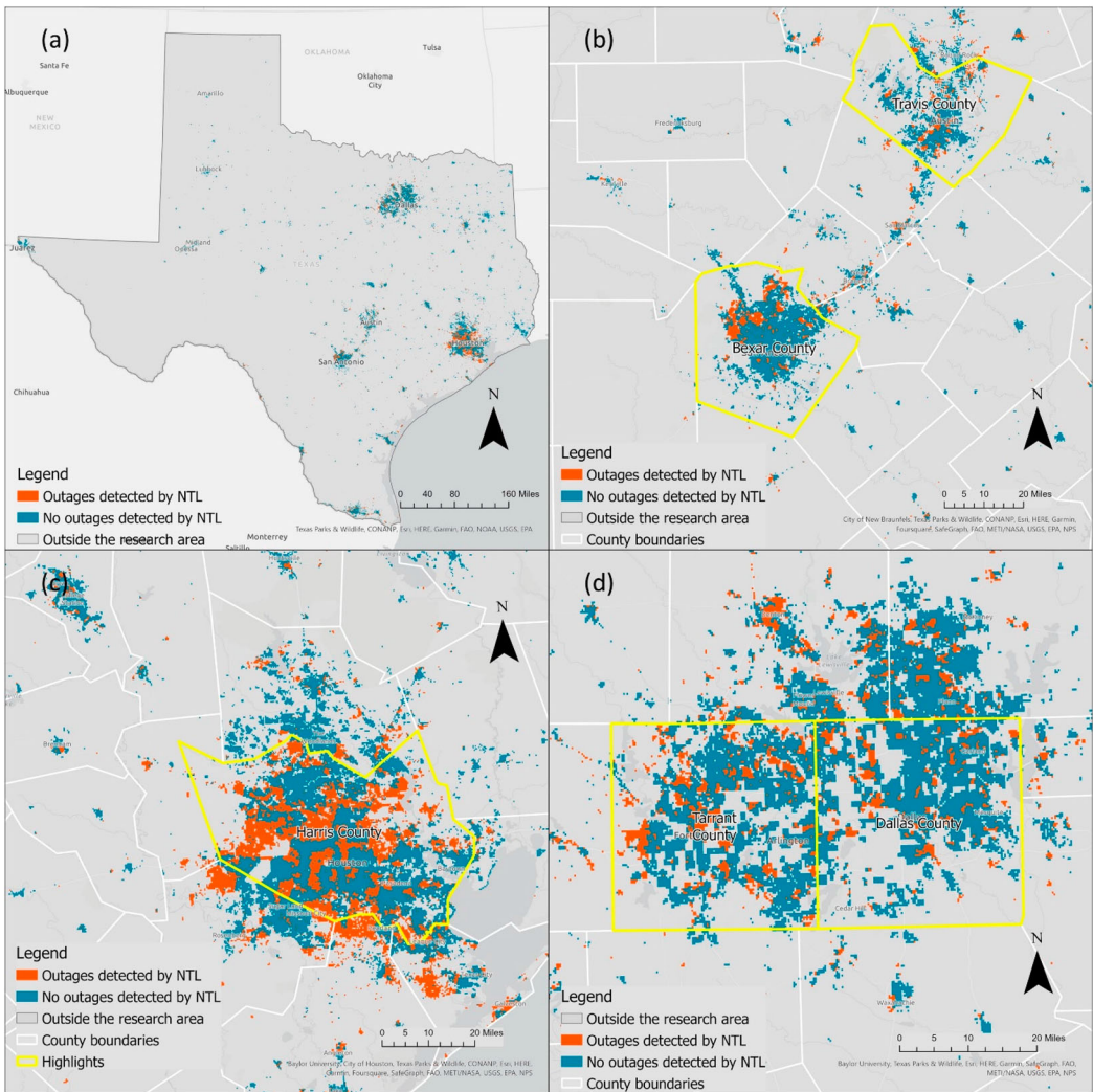
Figure 10. (a) Outage pixels from NTL images in the declared disaster counties in Texas, (b) zoom-in view of Austin (Travis County) and San Antonio (Bexar County), (c) zoom-in view of Houston (Harris County), (d) zoom-in view of Dallas (Dallas County) and Fort Worth (Tarrant County).
