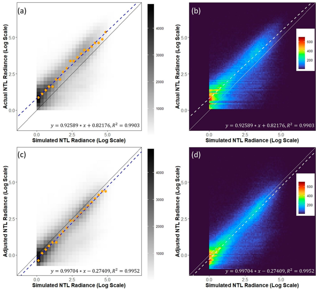
Figure 8. (a) Bin-fit scatterplot between the actual NTL radiance and simulated NTL radiance on Feb 16 (bin width = 0.25 unit), (b) density plots between the actual NTL radiance and simulated NTL radiance on Feb 16, (c) bin-fit scatterplot between the adjusted NTL radiance and simulated NTL radiance on Feb 16. Black lines in (a)&(c) and white lines in (b)&(d) indicate the adjustment target ( f(x) = x ). The blue dashed lines in (a)&(c) and white dashed lines in (b)&(d) indicate the actual bin fit to the target in all figures (equation and R^2 listed at the bottom of each graph).
