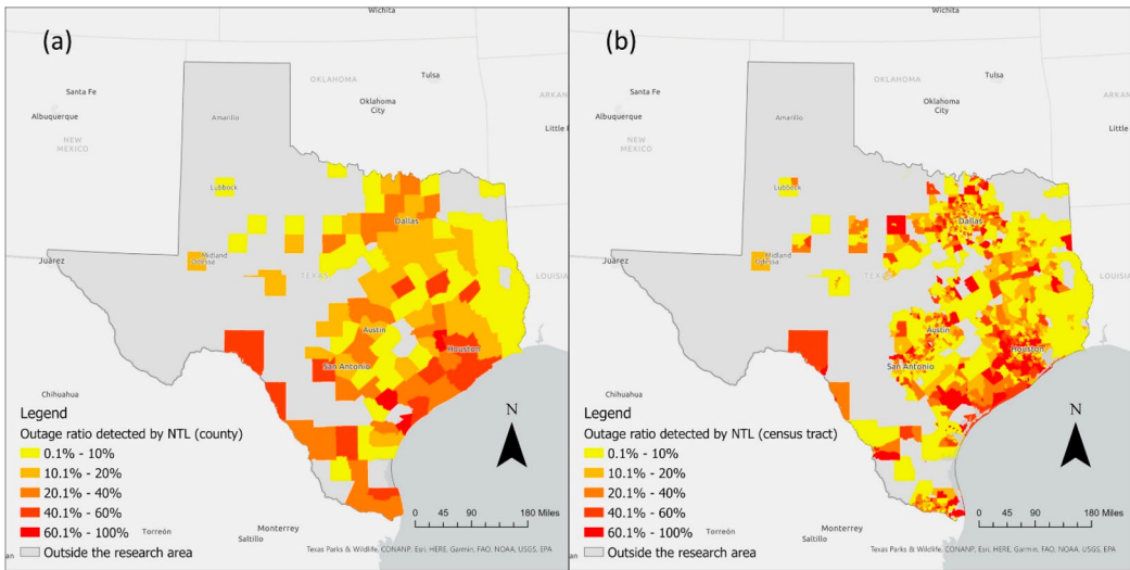
Figure 11. (a) Power outage ratios aggregated in counties, (b) power outage ratios aggregated in census tracts.
