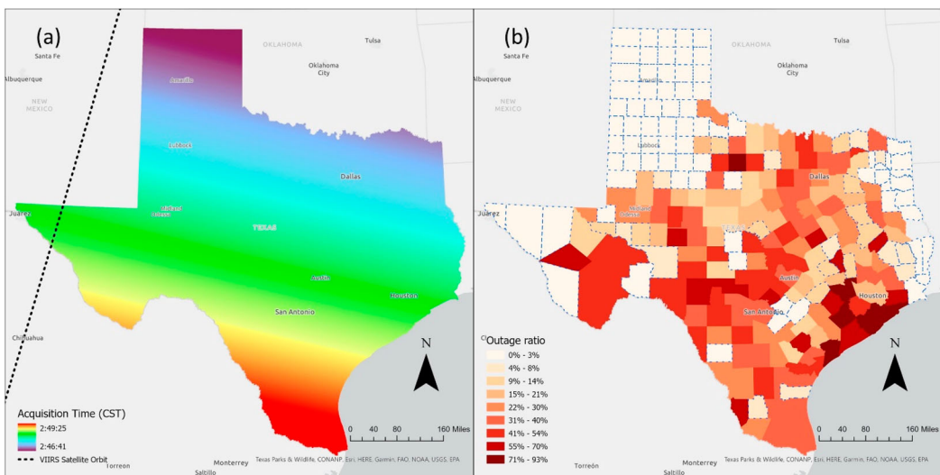
Figure 4. (a) Acquisition time in Central Standard Time (CST) and VIIRS satellite orbit from VNP46A2 on Feb 16, 2021, (b) power outage ratios (tracking data) between 2–3 AM in Texas counties, areas that did not experience extensive power outages are highlighted in blue dashed boundaries.
