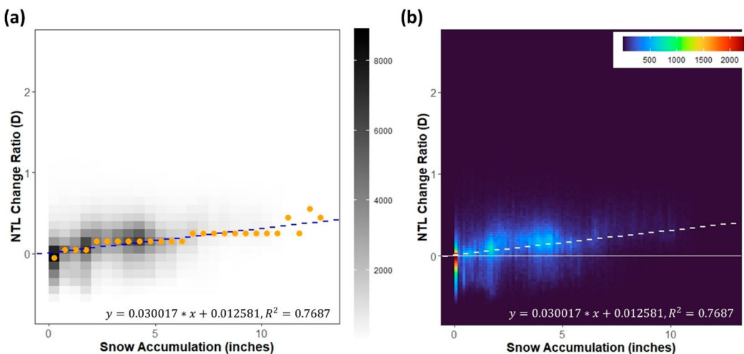
Figure 7. (a) Bin-fit scatterplot between 72-hour snowfall and NTL difference ratio ( D ) of pixels in the Feb 16 NTL image, (b) density plots between 72-hour snowfall and NTL difference ratio ( D ) of pixels in the Feb 16 NTL image. The white horizontal line ( D = 0 ) represents no change in NTL. The blue dashed line in (a) and white dashed line in (b) indicate the actual bin fit to the target (equation and R^2 listed at the bottom of each graph).
