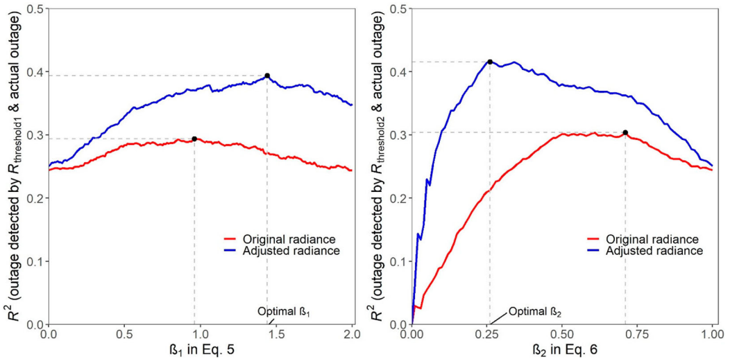
Figure 9. Changes of R^2 with increasing \beta_1 (left) and \beta_2 (right) in the iterative program. Blue and red curves are calculated with adjusted and original radiance, respectively.
