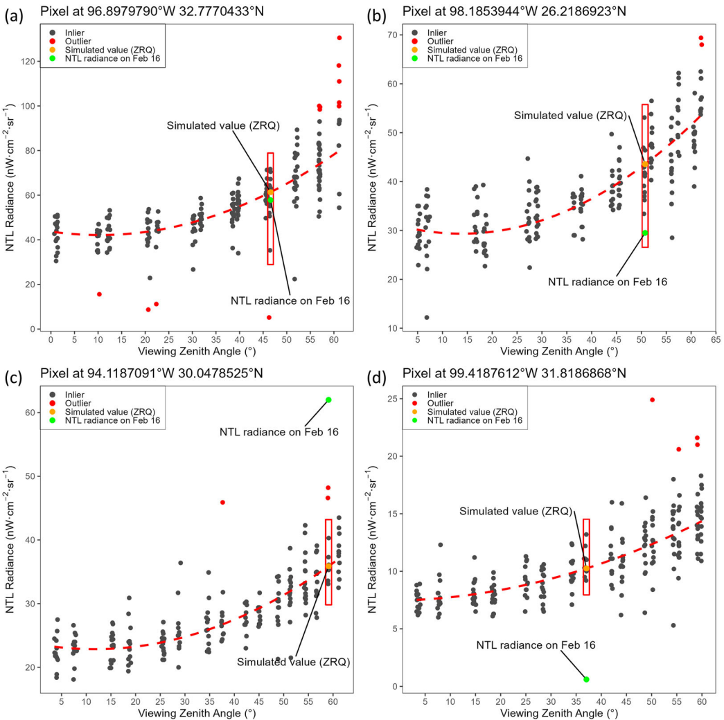
Figure 5. Scatterplots of radiance by zenith angle from Jan 1, 2020, to Mar 2, 2021, in random four pixels in the study area. The red box indicates the radiance values on dates that have a similar viewing zenith angle as Feb 16, 2021.
