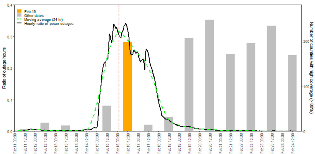
Figure 3. Hourly ratio of power outage from Feb 11 to Feb 24 (lines, left axis) and the number of counties where > 80% area is covered by high-quality NTL pixels (bars, right axis). The red dashed line indicates the general NTL acquisition time (close to 2:45 AM Central Standard Time) of NTL images on Feb 16, 2021.
