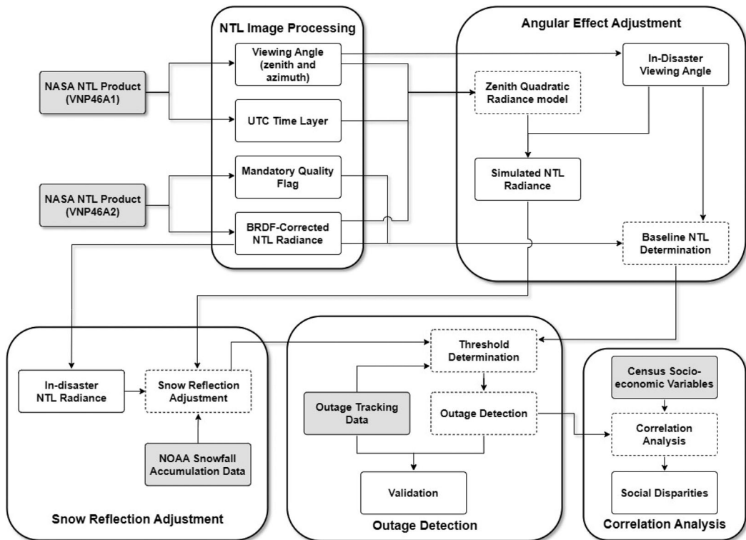
Figure 1. Workflow of outage detection using NASA's Black Marble product suites.
