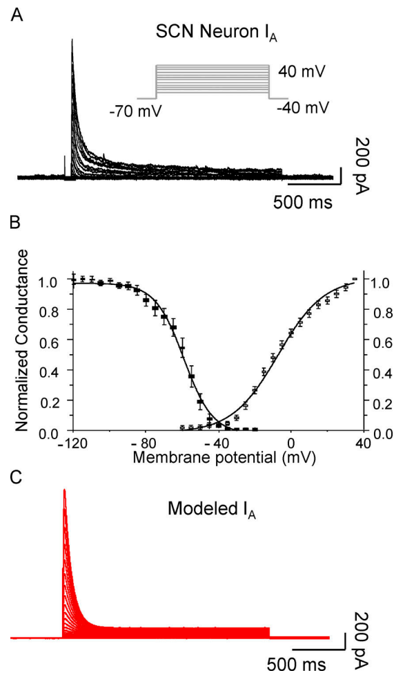
Figure S3. Cybercyte modeled I_A . A Markov model describing the gating of the K^+ channels that generate I_A in WT SCN neurons was developed based on a previously described model of the rapidly activating and inactivating, I_A -like, K^+ current in (ferret) ventricular myocytes (Campbell et al., 1993), and was populated using previously acquired voltage-clamp data detailing the time- and voltage-dependent properties of I_A in mouse SCN neurons (Hermanstyn et al., 2017). (A) Representative I_A waveforms recorded from a WT SCN neuron (Hermanstyn et al., 2017) in response to voltage steps to test potentials ranging from -40 to +40 mV (in 5 mV increments) from a HP of -70 mV are shown; the voltage-clamp paradigm is illustrated above the current records. (B) The voltage-dependences of activation and inactivation for I_A in WT SCN neurons (Hermanstyn et al., 2017) were determined using protocols identical to those described above for the CX4-sensitive currents. The V_{1/2} and the k values derived from these fits for current activation (open symbols) and inactivation (closed symbols) were V_{1/2} = -9.3 \pm 1.3 mV; k = 12.7 \pm 0.8 ( n = 12 ) and V_{1/2} = -59.4 \pm 2.1 mV, k = 7.9 \pm 0.7 ( n = 12 ), respectively. (C) These parameters were used to tune the model. (C) The waveforms of the currents produced by the Cybercyte I_A model reliably reproduced I_A recorded from WT SCN neurons (A).
