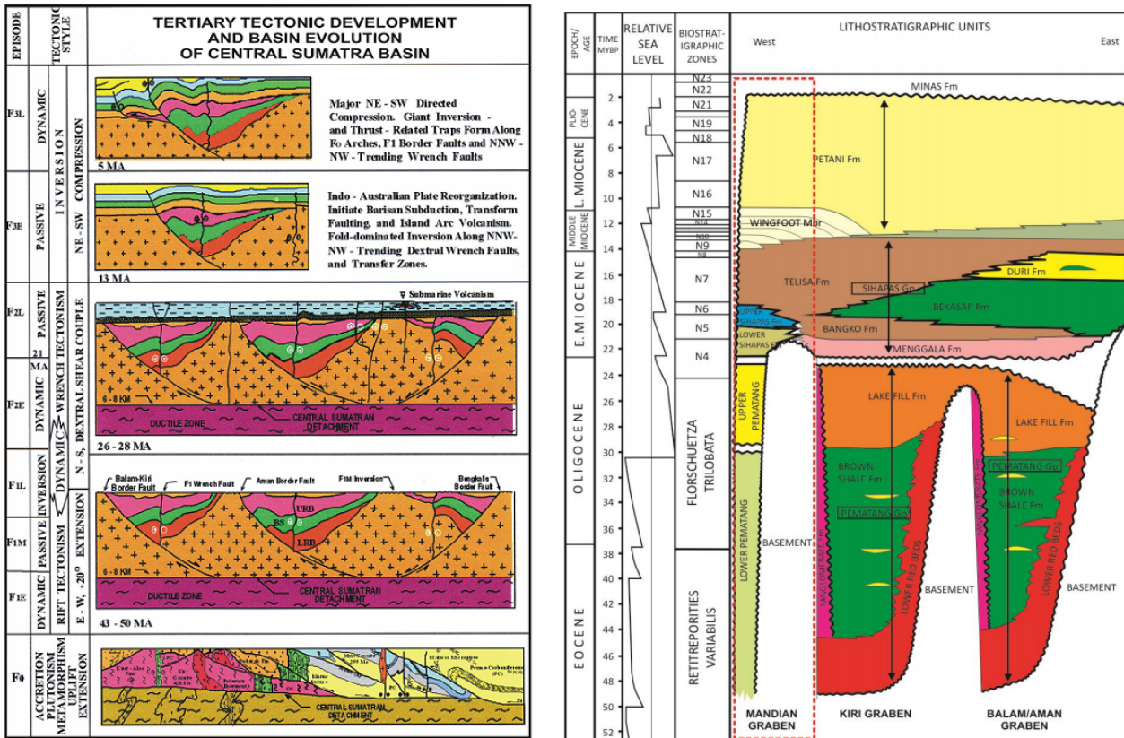
FIGURE 2. a) Tectonic development of Central Sumatra Basin (Heidrick & Aulia, 1993) b) Stratigraphic column in the study area (dashed red polygon) within the Central Sumatra Basin (Williams & Eubank, 1995).
