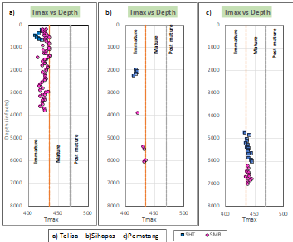
FIGURE 5. Plotting of Tmax vs depth in three available wells a.) Telisa Formation, b.) Sihapas Formation, c.) Pematang Formation.
