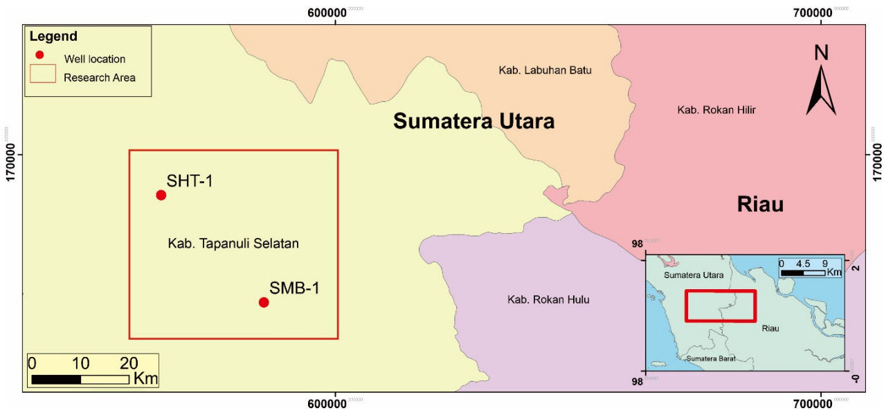
FIGURE 1. Research area with two available wells located in Tapanuli Selatan (Source: Peta Indonesia Geospasial, 2019).
