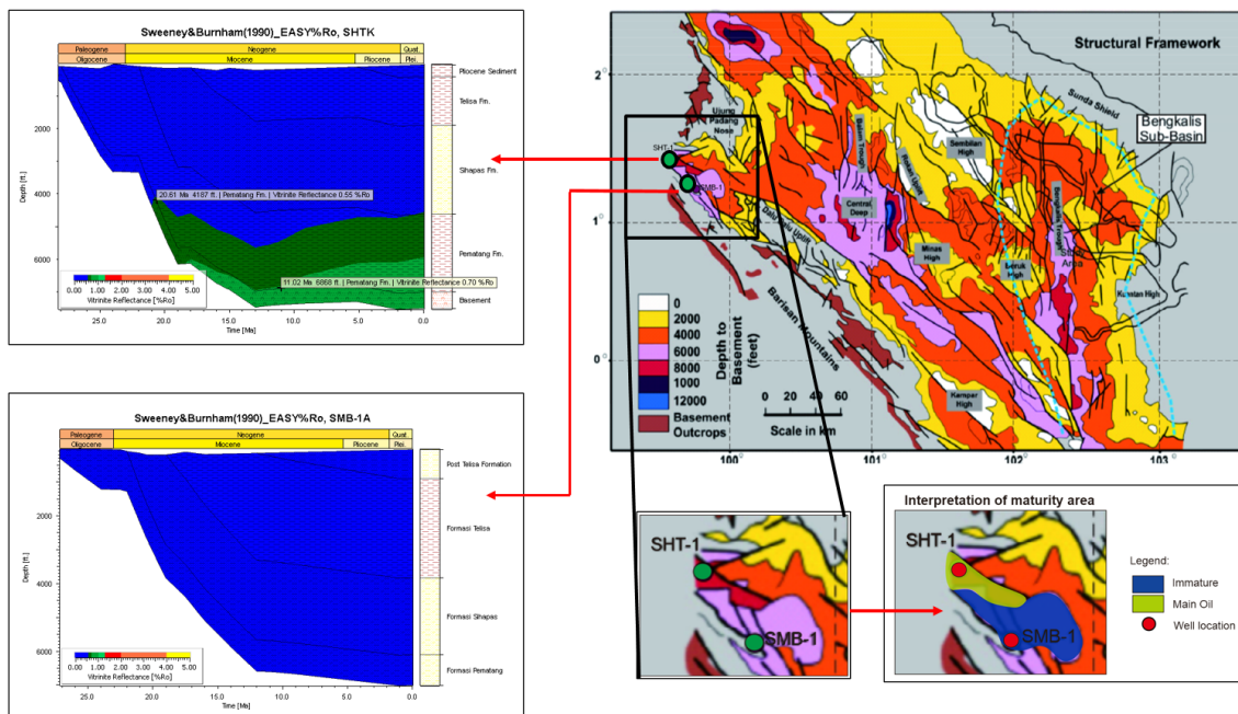
FIGURE 7. Interpretation of maturity area in Structural Pattern Map (modified after Pertamina BPPKA, 1996).
