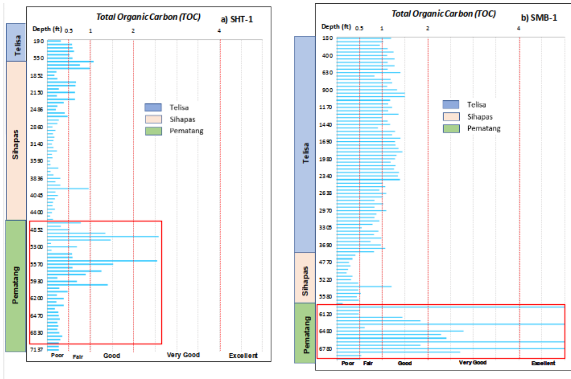
FIGURE 3. Quantity of organic matter by the amount of TOC in the a.) SHT-1 well, and SMB-1 well.
