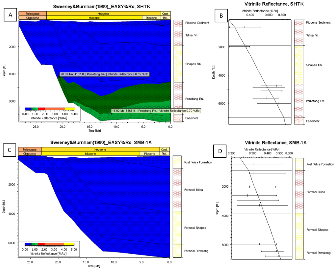
FIGURE 6. The simulated vitrinite reflectance value and the associated geohistory of all formations in research well (SHT-1) (a and b). (c) 1D maturity model of the SMB-1 well indicates that this well has not reached the maturity window. (d) The Ro Model and Ro calibration were measured to build the SMB-1 model.
