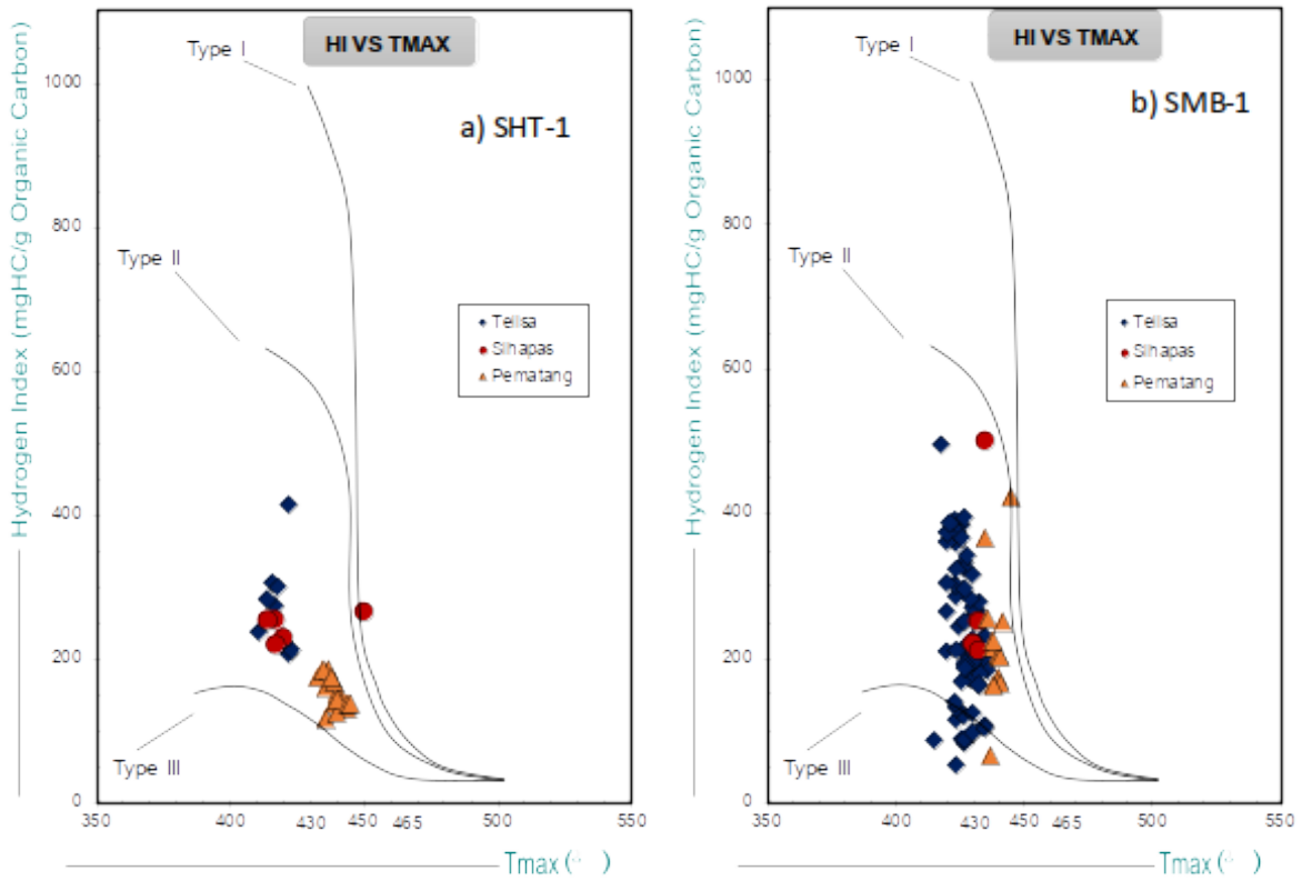
FIGURE 4. Hydrogen Index vs Tmax (Mukhopadhyay et al., 1995) showing the type of kerogen of a.) SHT-1 well, and b.) SMB-1 well.
