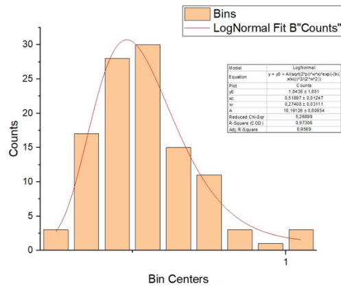
Figure 4. Particle diameter distribution on hap from kupang shell
