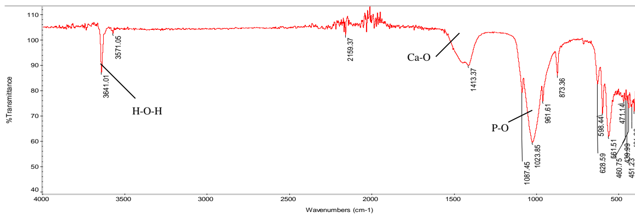
Figure 1. Results of FT-IR HAp analysis from kupang shells
