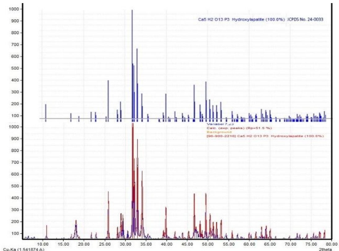
Figure 2. XRD results of the hydroxyapatite synthesis from
