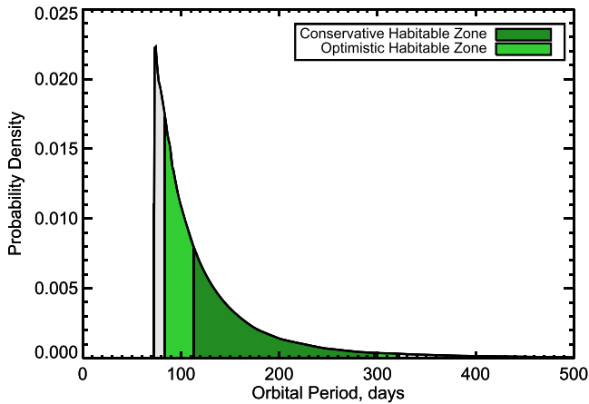
Figure 8. Constraints on the orbital period of HD 283869 b. The black curve shows the probability distribution of the orbital period from our analysis in Section 3.5. The light green and dark green shaded regions represent orbits that fall in the optimistic and conservative circumstellar habitable zones, respectively (Kopparapu et al. 2013). Despite our weak constraint on orbital period, we can say fairly confidently that if real, HD 283869 b is temperate, with a 71% chance of orbiting within the star’s habitable zone and a 99% upper limit on equilibrium temperature of 327 K.
