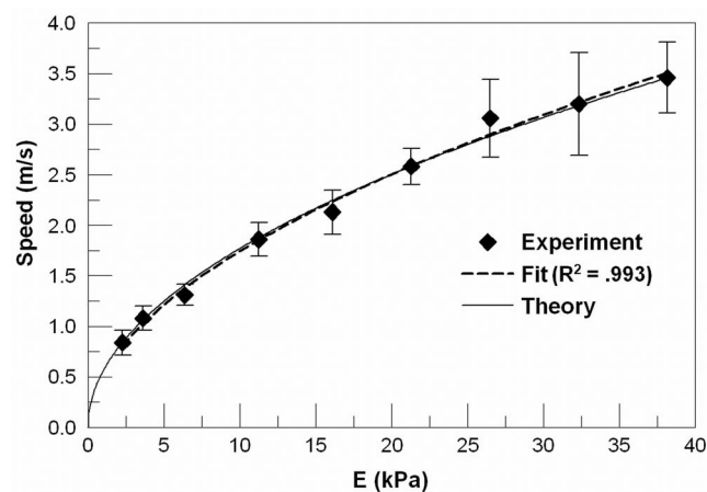
Fig. 3 Variation in SAW speed as a function of the Young's modulus in homogeneous tissue phantoms follows the expected relationship of Eq. (6).
