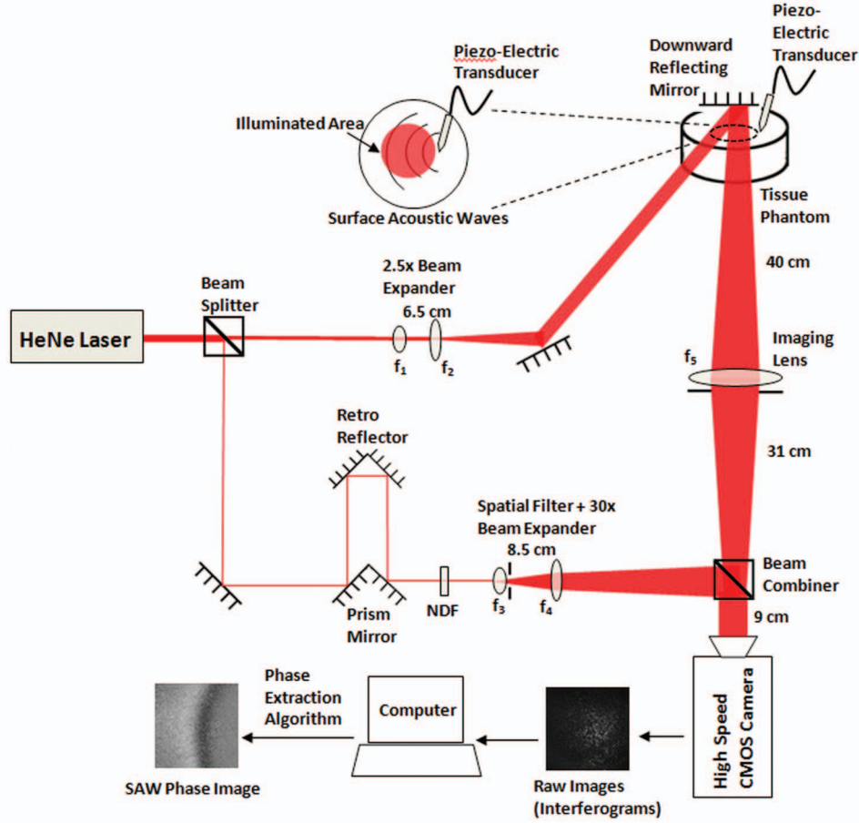
Fig. 1 Schematic diagram of holographic elastography experimental setup. NDF: neutral density filter, f_1 = 40 mm, f_2 = 100 mm, f_3 = 5 mm; f_4 = 150 mm, and f_5 = 200 mm.
