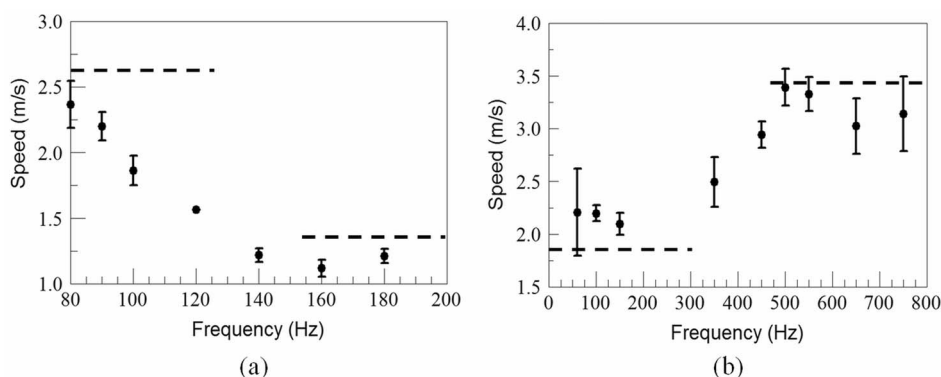
Fig. 4 SAW speed variation with driving frequency for (a) a phantom with upper softer layer and (b) a phantom with upper stiffer layer.
