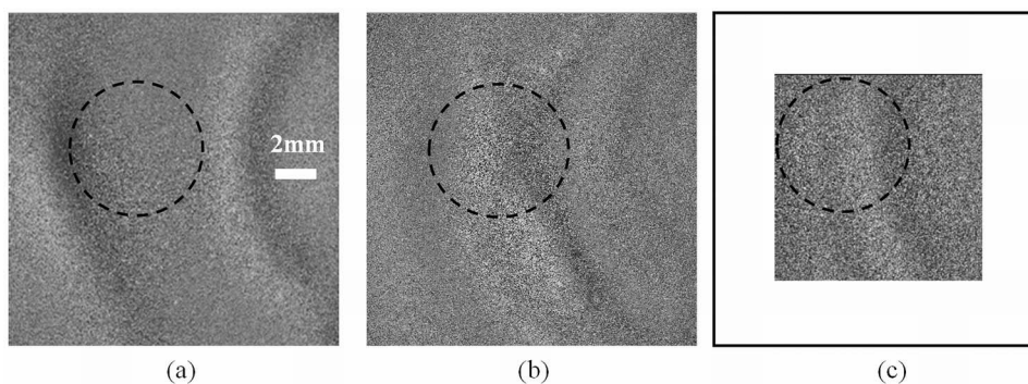
Fig. 5 SAW propagation in a phantom with a local inhomogeneity at frequencies of 65 Hz (a) (Video 3), 89 Hz (b) (Video 4), and 200 Hz (c) (Video 5). The image at 200 Hz has a smaller field of view due to the increased frame rate. The dashed circle indicates the lateral position of the metal ring. (Video 3, QuickTime, 728 KB) [URL: http://dx.doi.org/10.1117/1.3646211.3 ]; (Video 4, QuickTime, 878 KB) [URL: http://dx.doi.org/10.1117/1.3646211.4 ]; (Video 5, QuickTime, 986 KB) [URL: http://dx.doi.org/10.1117/1.3646211.5 ]
