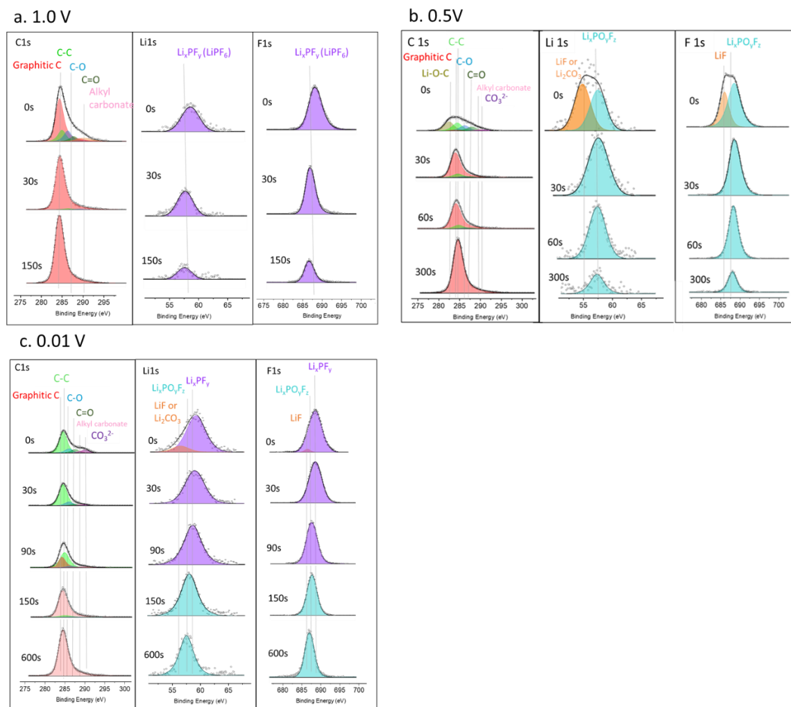
Figure 8. High resolution XPS spectra of C 1s, O 1s, Li 1s, F 1s before and after Ar ion sputtering in SEI formed on HOPG which has been scanned from OCP to 1V, 0.5V and 0.01V vs Li/Li + .
