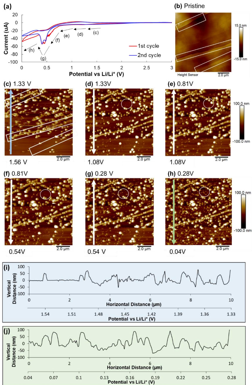
Figure 2. Operando EChem-AFM (10 \mu\text{m} x 10 \mu\text{m} ) of an HOPG electrode in an electrolyte of 1.2 M \text{LiPF}_6 in EC: EMC (3:7 w/w), with a scan rate of 0.5 mV/s. (a) Cyclic voltammograms for the first two cycles of an HOPG electrode; the arrows indicate the potential range in which the corresponding AFM images were collected; (b) AFM image of a pristine surface of HOPG, boxed areas indicate \sim 10 layers of step edges; (c-h) Operando AFM collected during the cathodic scan of the first cycle at different potential ranges, the circled areas highlighted a small basal plane region; (i-j) representative height profile of (c) and (h) taken along the blue and green arrow, respectively.
