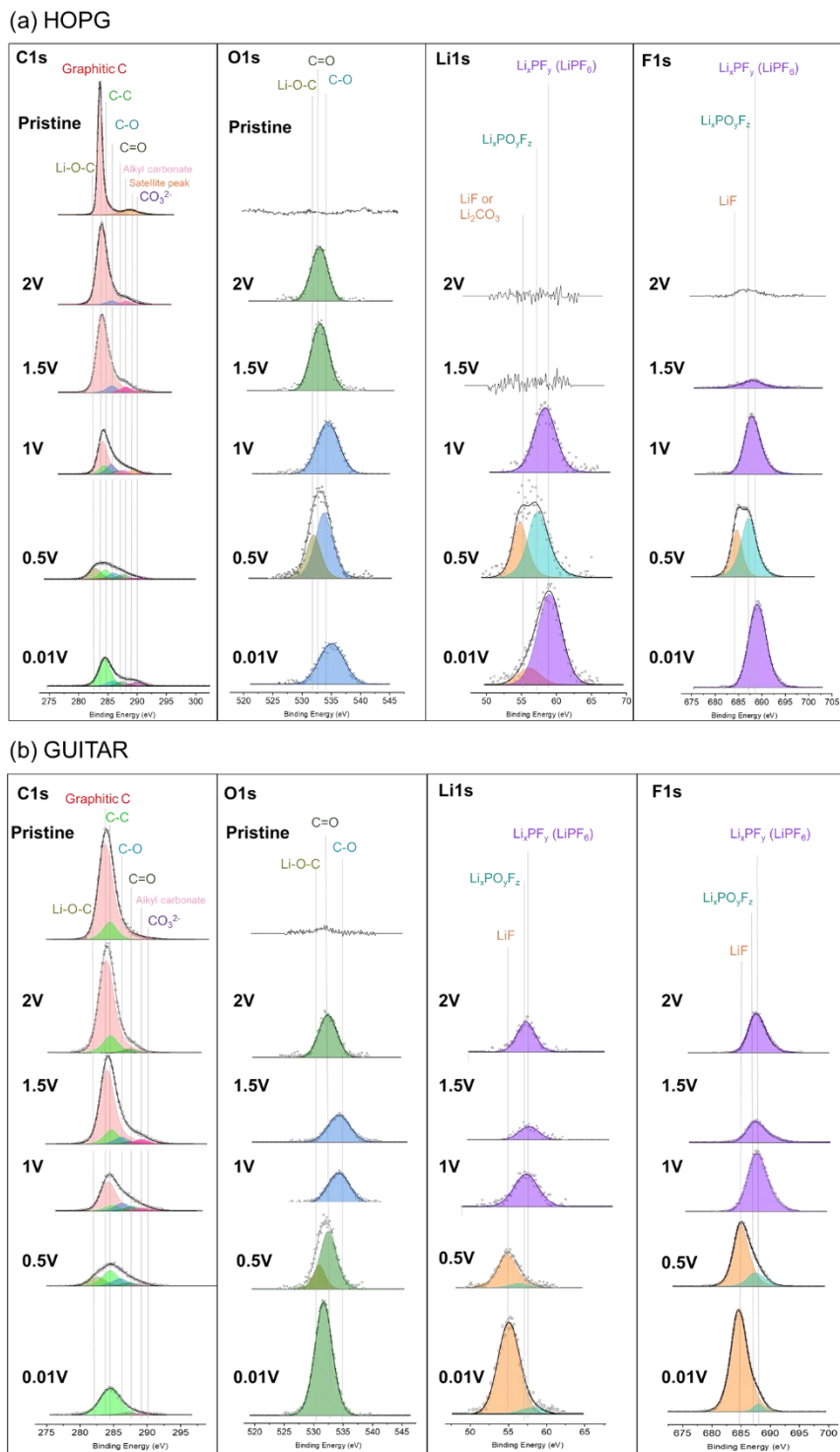
Figure 6. High resolution XPS spectra of C 1s, O 1s, Li 1s, F 1s in (a) HOPG and (b) GUITAR electrodes scanned through the potential ranges as indicated.
