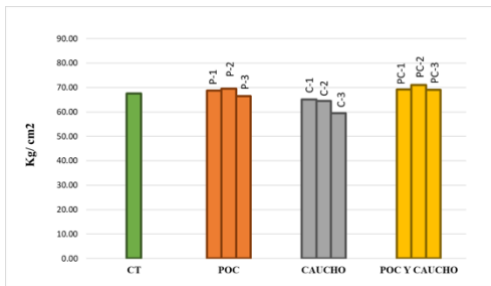
Figure 3. PC flexural strength respect to CT
