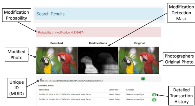
Fig. 4: Use Case 1 search result, using kodim23 image from Kodak dataset [28].
