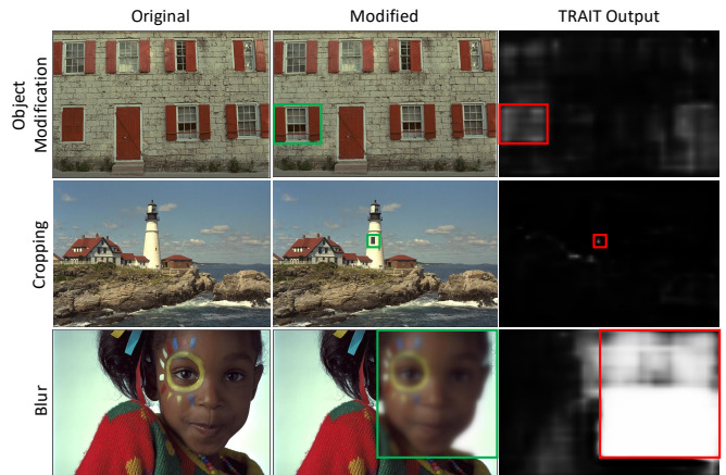
Fig. 1: Examples of fake media (image manipulation): object modification, cropping and blur. 1st and 2nd columns are the original and the modified versions of images, and 3rd column represents the output of TRAIT framework. The modified regions have been highlighted in green (2nd column) and red colors (3rd column).
