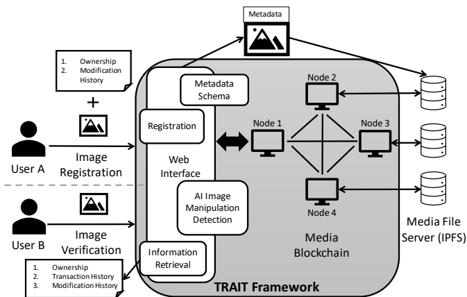
Fig. 2: Overview of the TRAIT Framework.
