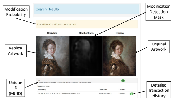
Fig. 5: Use Case 2 search result, using Fragonard’s Young Woman [31].
