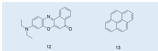
Fig. 11 Chemical structures of NR (12) and pyrene (13).
