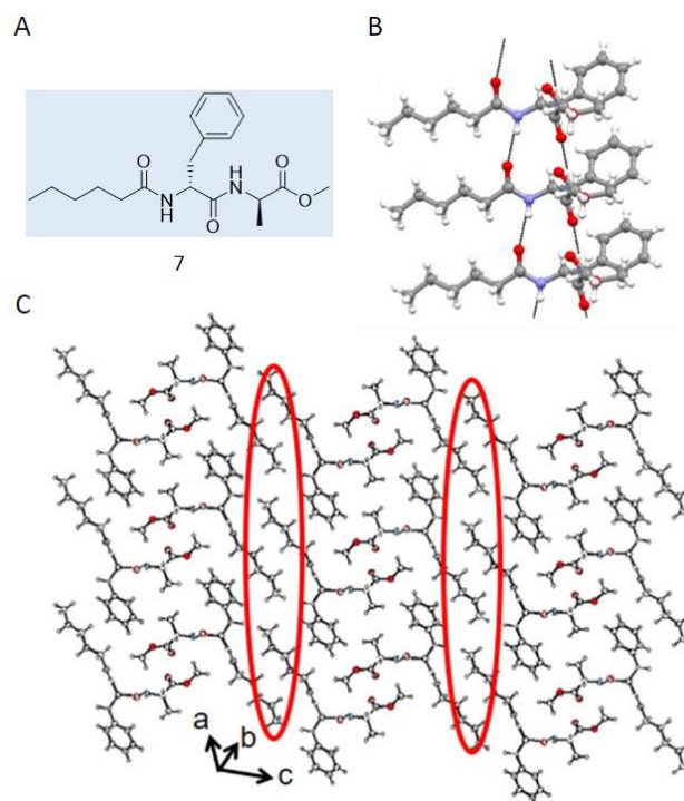
Fig. 7 A) Chemical structure synthesised by Halder and co-workers 7 . B) Crystal structure of 7 showing a hydrogen bonded sheet stabilised by \pi - \pi interactions. C) Extended crystal structure, showing how hydrophobic interactions (circled in red) stabilise interactions between sheets. Carbon = grey, oxygen = red, nitrogen = blue, hydrogen = white. Reproduced/adapted from ref. 76 with permission from MDPI Chemistry.
