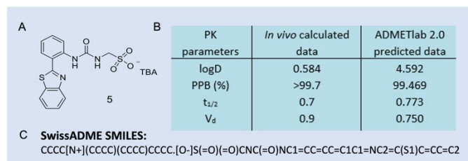
Fig 21 A) The structure of 5 , TBA = tetrabutylammonium. B) Table of in vivo data (mouse blood PK studies, n = 3, intravenous route, and dose of 1 mg/kg) versus in silico generated
