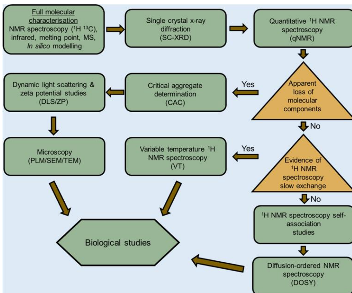
Fig. 25 Systematic method for the characterisation of SSAs. 11,15,34,36,37,41,47,48,181,182 Rectangle/hexagon = action; triangle = decision. Reproduced/adapted from ref. 15 with permission from MDPI Molecules
