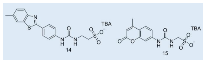
Fig. 12 Chemical structures of SSAs 14 and 15 used to develop the CAC OD-based microplate methodology. TBA = tetrabutylammonium.
