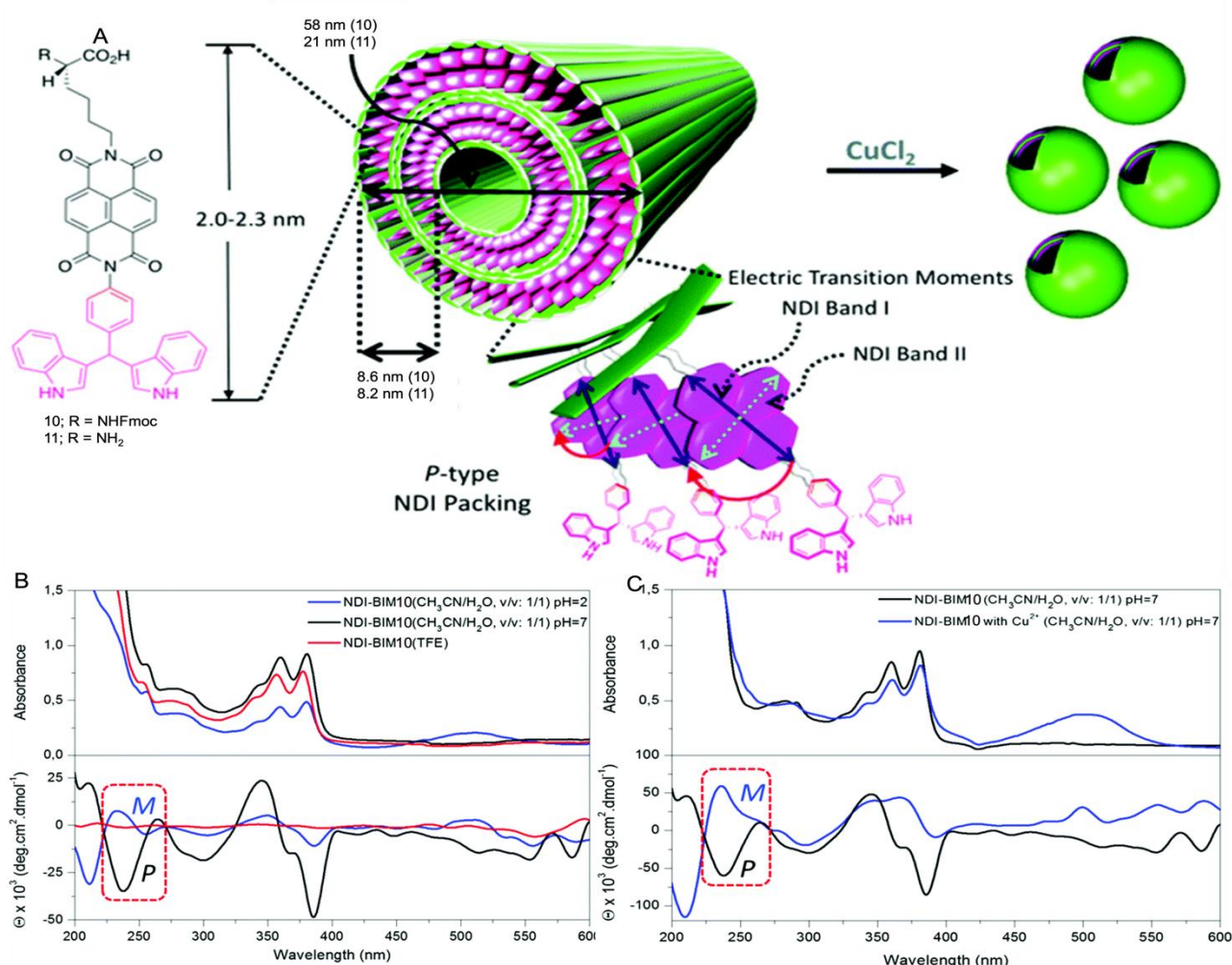
Fig. 9 A) Self-assembly of NDI-BIMs 10 and 11 . B) UV-Vis and CD spectra of 10 in \text{CH}_3\text{CN}:\text{H}_2\text{O} (1:1) in pure TFE. C) UV-Vis and CD spectra of 10 and 10-Cu in \text{CH}_3\text{CN}:\text{H}_2\text{O} (1:1) at pH 7. Reproduced/adapted from ref. 93 with permission from RSC Dalton Transactions .
