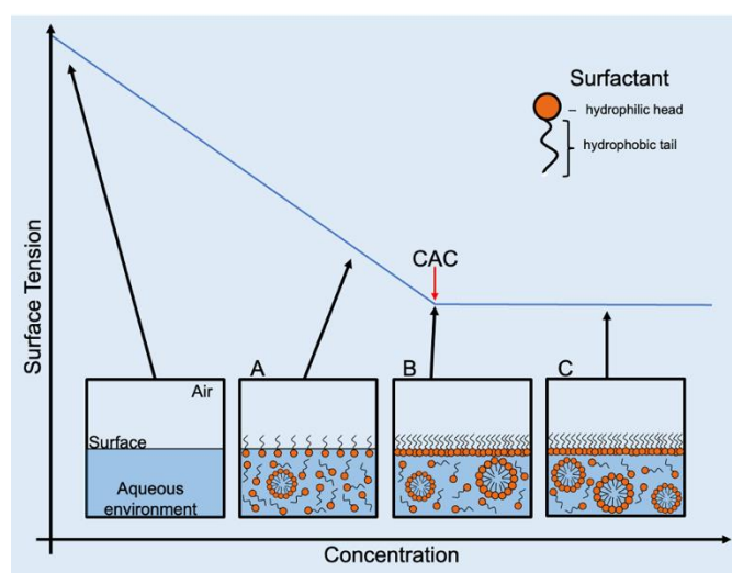
Fig. 10 Graphical depiction of CAC determination for amphiphilic species in an aqueous environment (including supramolecular amphiphiles): A) amphiphiles adsorb at the surface in equilibrium with aggregate formation, B) surface is fully saturated, and CAC is
