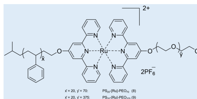
Fig. 8 Structures of the two micelle-forming copolymers PS 20 -[Ru]-PEO 70 8 and PS 20 -[Ru]-PEO 375 9 . Reproduced/adapted from ref. 85 with permission from the Wiley Journal of Polymer Science Part A: Polymer Chemistry .
