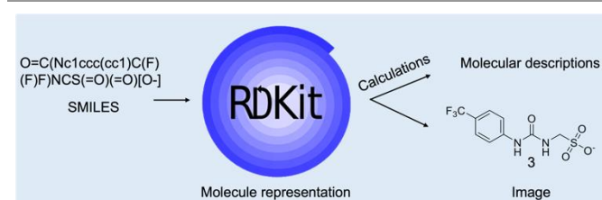
Fig. 23 The generation of molecular descriptors from a SMILES string using the RDKit library. The figure depicts the anionic group from 3.
