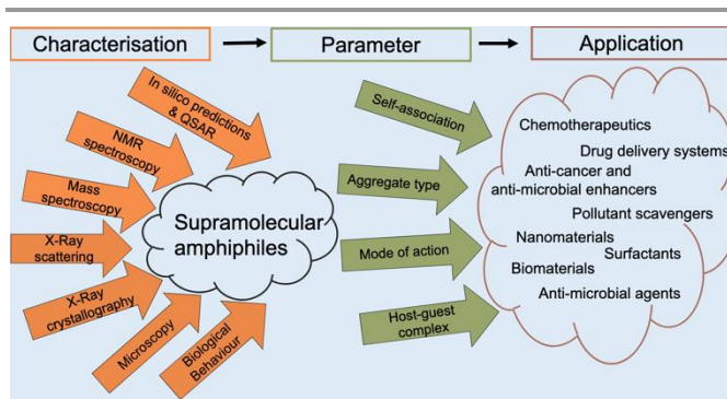
Fig. 2 Different techniques for characterising supramolecular amphiphiles (orange), the subsequent parameters obtained from the characterisation (green), and the various applications of supramolecular amphiphiles (brown).
