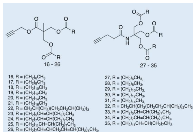
Fig. 13 Structures of amphiphiles 16–35 synthesised by Feast and co-workers. Reproduced/adapted from ref. 114,115 with permission from Beilstein Journal of Organic Chemistry .
