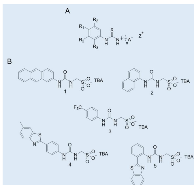
Fig. 3 A) General chemical structure of an SSA. R = any group; X = S or O; n = 1, 2, or 3; A - = sulfonate or carboxylate; Z + = counter cation. B) Molecular structures of SSAs developed by Hiscock and co-workers (1 - 5). 11 TBA = tetrabutylammonium. Reproduced/adapted from ref. 11 with permission from RSC Chemical Science .
