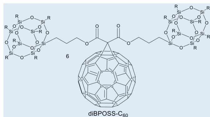
Fig. 5 Chemical structure of diBPOSS-C 60 6 . Reproduced/adapted from ref. 63 with permission from Elsevier Polymer .
