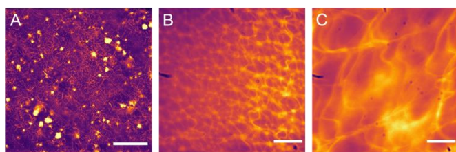
Fig. 15 Fluorescent microscopy images of self-associated fibres formed from A) 4 , B) 14 and C) 36 (5 mg/mL) in and aqueous solution of Na 2 SO 4 at 0.505 M. Scale bar A = 120 μm, B and C = 20 μm. Reproduced/adapted from ref. 5 with permission from RSC Journal of Material Chemistry B .
