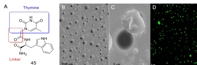
Fig. 19 A) TrpT, 45 . B) and C) Morphology of TrpT self-assembly in aqueous media (SEM analysis). D) Curcumin encapsulated (green) by TrpT nanovesicles (confocal microscopy analysis). Reproduced/adapted from ref. 170 with the permission of Creative Commons Attribution 4.0 International License ( http://creativecommons.org/licenses/by/4.0/ ).
