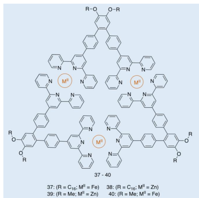
Fig. 16 Structure of metallotriangles 37-40 , synthesised by Ludlow and co-workers. Reproduced/adapted from ref. 119 with permission from Taylor and Francis Supramolecular Chemistry .
