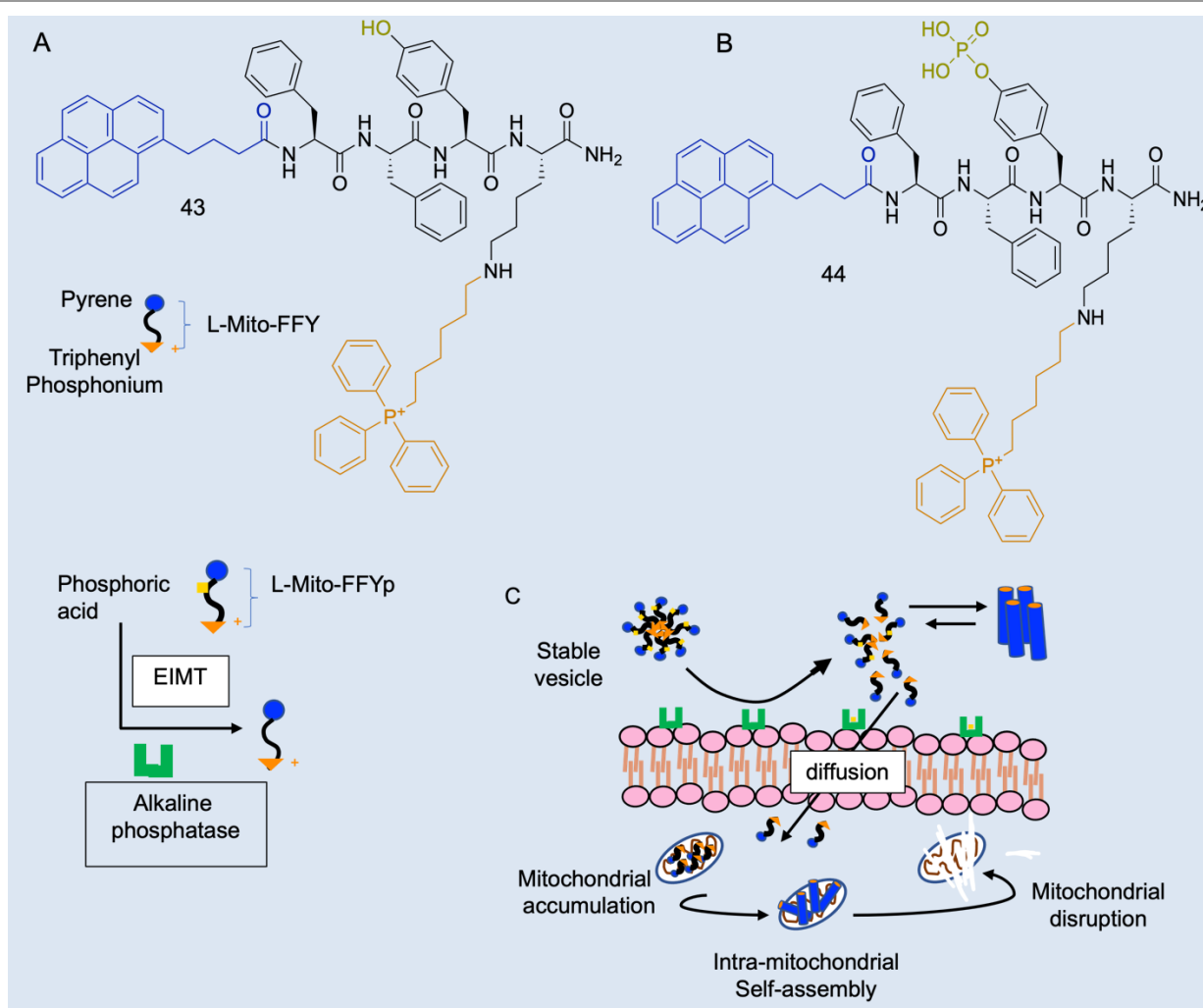
Fig. 18 Schematic illustration of the enzyme-instructed morphology transformation (EIMT) of an ALP-responsive micelle. A) Chemical structure L-Mito-FFY 43 . B) Chemical structure of L-Mito-FFYp 44 and schematic
