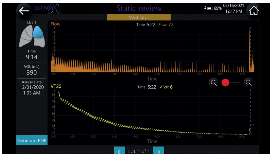
Figure 5 - Chartis measurement output image showing the “volume trend for the previous 20 s” (VT20) value plotted for an assessment with continued high spikes in air flow (flow of 72 \text{ mL}\cdot\text{min}^{-1} at 5:22 min) values for the duration of the assessment.
