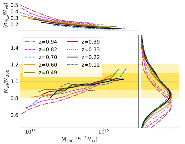
Fig. 13. Average weak lensing mass bias as a function of the cluster halo mass M_{200} for different lens redshifts. Right and top subpanels are the same as Fig. 6.
