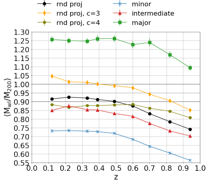
Fig. 14. Average cluster weak lensing mass bias as a function of the lens redshift. The various data points and colours refer to different ways of computing the cluster masses. Black circles display the case of random projections and modelling both the halo mass and concentration, orange diamonds, and olive-coloured pentagons consider the cases in which we assume a fixed concentration parameter – three and four, respectively – and we fit only the halo mass. Light-blue crosses, red triangles and green squares show the average mass bias for the three particular projections, along the minor, the intermediate, and the major axis, respectively.
