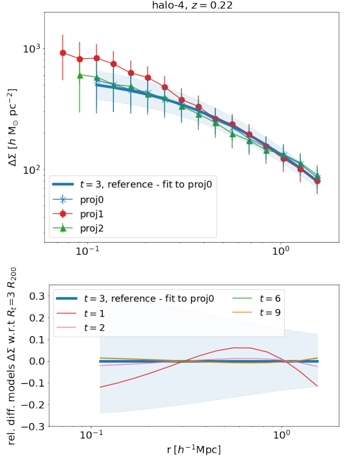
Fig. 4. Top panel: Excess surface mass density profiles of the three random projections for a cluster-size halo at z_1 = 0.22 , as displayed in Fig. 3. The blue, red and green data points show the circular averaged profiles of the halo projected along the z , y , and x axis of the re-simulation box. The error bars on the data points account for both the dispersion of the intrinsic ellipticity of background galaxies and the error associated with the average measure in the considered radial bin. The blue solid line displays the best fit model to proj0, while the shaded region represents the model within the 68% of confidence. Bottom panel: relative difference of the best fit models assuming different values of the truncation radius R_t with respect to the reference case with t = 3 .
