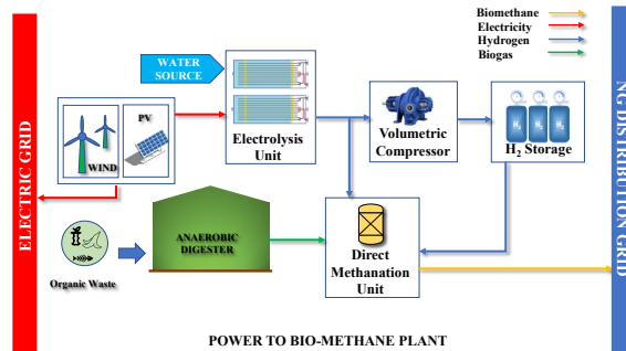
Fig. 1. Power to Bio-methane plant concept
