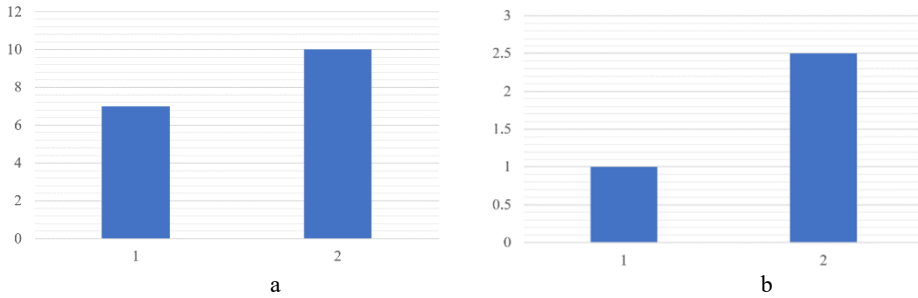
Fig. 2. Comparison of recycling desalination machines: a – heating water consumption; b – productivity; 1 – heating water temperature at the evaporator inlet is 60 °C; 2 – heating water temperature at the evaporator inlet is 80 °C.
