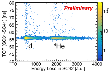
Fig. 5. Particle identification plot with the FRS setting for {}^4\text{He} and deuteron during the HypHI experiment. The abscissa shows energy deposition measured by SC42, and the ordinate shows TOF between SC31 and SC41.
