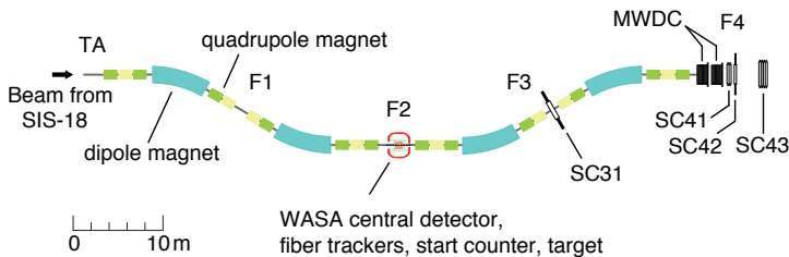
Fig. 1. A schematic view of the general experimental setup integrating the WASA central detector at the fragment separator FRS. See the text for details.
