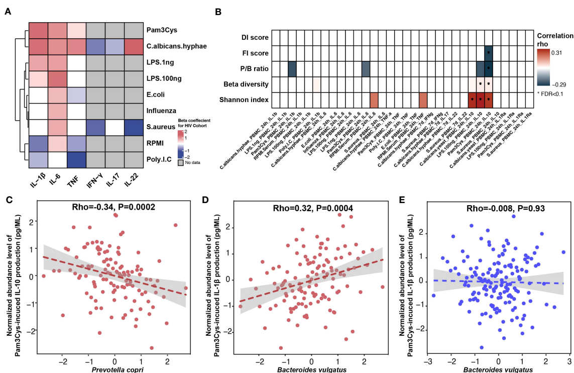
FIGURE 3 Association between gut microbiome and inflammatory cytokine production. (A) Heatmap showing ex vivo cytokine production enriched (red) and depleted (blue) in PLHIV as compared with HCs from 500FG. A linear regression model (age and sex included as covariates) was used to calculate the P-values. Box color indicates the Spearman correlation rho for those associations that were significant at p-value < 0.05 level. The associations at FDR < 0.1 level were highlighted with *. White box indicates associations with p-value > 0.05, and gray box indicates no measurement. (B) Heatmap showing Spearman correlation rho between cytokine production and HIV-associated bacterial signature (Shannon index, beta diversity, P/B ratio, and DI and FI scores), with correction for age, sex, read counts, and sexual behavior. White box indicates P > 0.05. The row labels indicating the cytokine produced and the name of stimulation. (C, D) Association between relative abundance of species and cytokine production in PLHIV: (C) Prevotella copri with Pam3Cys-induced IL-10 production and (D) Bacteroides vulgatus with Pam3Cys-induced IL-1 \beta production. (E) Association between relative abundance of Bacteroides vulgatus and Pam3Cys-induced IL-1 \beta production in HCs from 500FG. The relative abundance of the species was CLR- and inverse-rank-transformed. Association was corrected for age, sex, read counts, and sexual behavior using linear regression. Pam3Cys, synthetic TLR2 ligand; LPS.1ng, PBMC cytokine production in response to LPS (1 ng/mL) stimulation; LPS.100ng, PBMC cytokine production in response to LPS (100 ng/mL) stimulation; RPMI, serum-free medium; Poly IC, TLR3 ligand.
