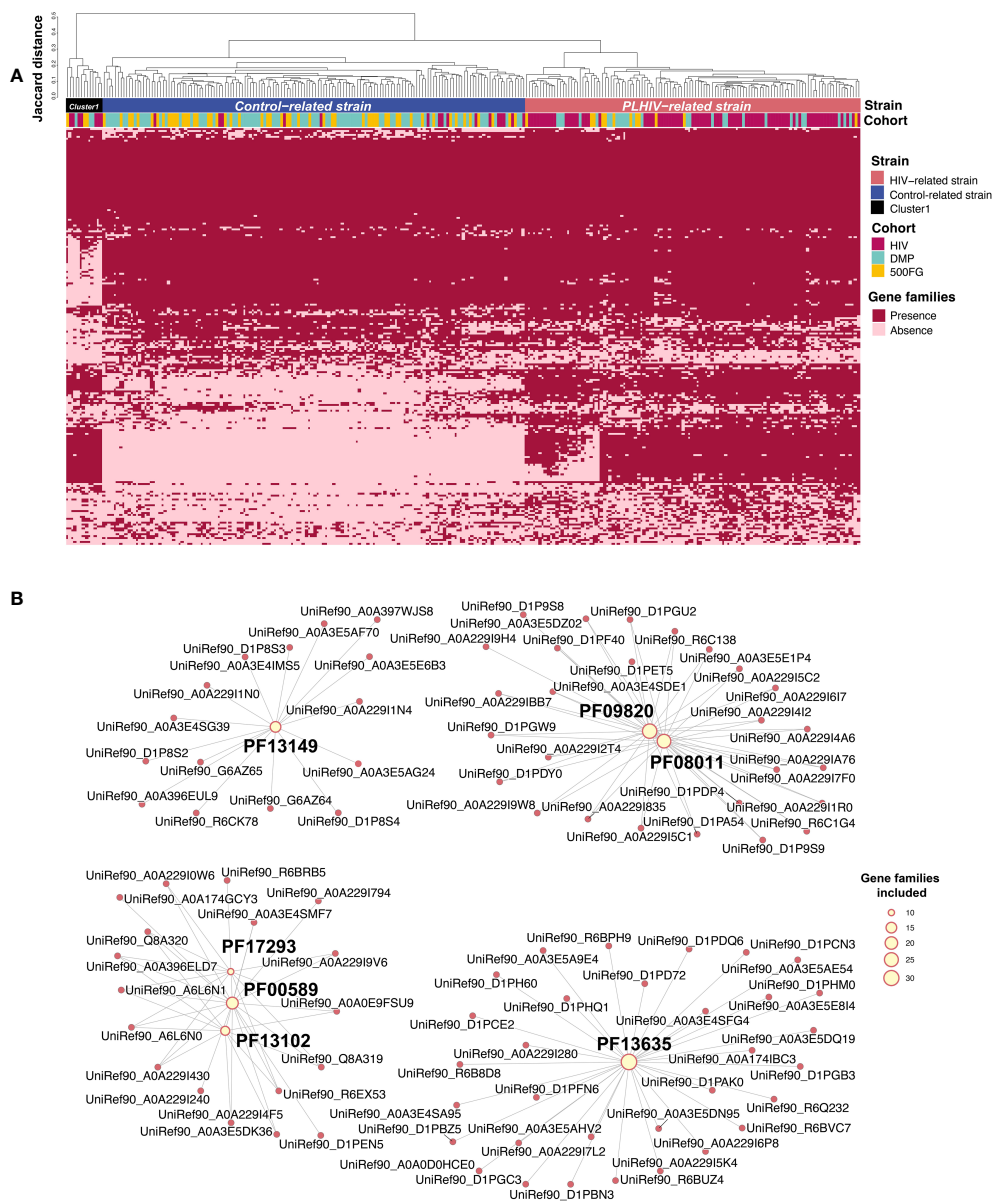
FIGURE 4 Prevotella copri strains with different genetic content. (A) Heatmap showing the gene family profiles of P. copri strains in samples from the three cohorts (282 samples total: 102 PLHIV, 111 DMP, and 69 500FG). Each column represents a sample. Each row represents the presence or absence of a gene family. The clustered tree above the heatmap shows the three clusters of P. copri strains. Most samples from PLHIV were binned together into the PLHIV-related strain (right), but 16 PLHIV samples (middle) showed different profiles and were binned into the control-related strain. (B) Network figure showing that the gene families increased in PLHIV-related strain are enriched in seven Pfams (FDR < 0.05). Pink dots represent different gene families. Yellow dots represent Pfams, and their sizes indicate how many gene families annotated to themselves. Lines indicate that the gene families are annotated to the corresponding Pfam. PF00589, phage integrase family; PF13102, phage integrase SAM-like domain; PF17293, Arm DNA-binding domain.
