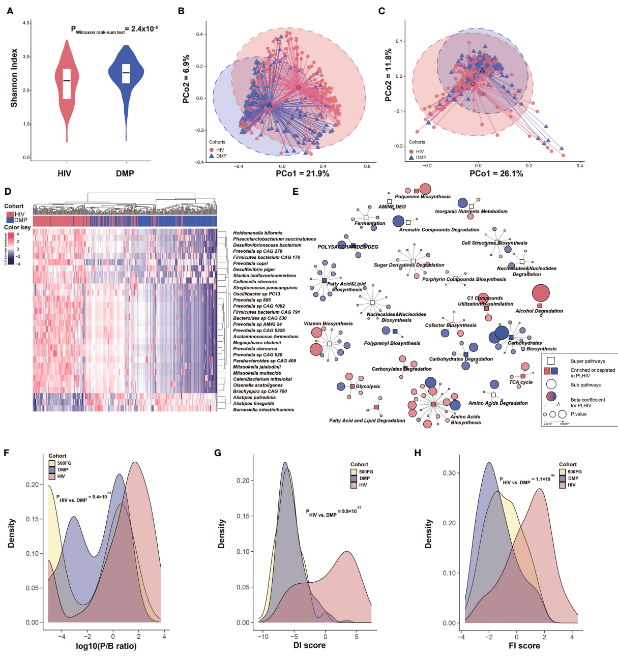
FIGURE 1 PLHIV show a distinct gut microbiome composition and function compared with HCs. (A) Comparison of microbial alpha diversity between the PLHIV cohort and HCs from the DMP cohort. Y-axis refers to the Shannon index at the species level. (B, C) Beta diversity based on Bray–Curtis distance of species and pathway abundance is shown in a principal coordinates analysis (PcoA) plot with centroids for PLHIV and HCs. The coordinates of the centroids are set as the mean value of the principal components for each cohort. (D) Heatmap depicting the relative abundance of the top 30 species that differed significantly between PLHIV and HCs. Data are CLR-transformed and then inverse-rank-transformed to follow a normal distribution. Differentially abundant species were selected using a linear regression model with correction for BMI, read counts, and smoking status. (E) Network of bacterial pathways that were significantly different between PLHIV and HCs. Rectangular nodes represent super-pathways, with the colors showing enrichment (pink) or depletion (blue) in PLHIV. Circular nodes show sub-pathways belonging to the super-pathways. The color of circles shows the log2 value of fold change between the relative abundance of pathway in PLHIV and HCs, where a gradient is applied depending on fold change. Circle size indicates p-value. Lines connect each pathway to its respective super-pathway. Only super-pathways including two or more pathways and sub-pathways with FDR < 0.05 are shown. Differentially abundant pathways were selected using a linear regression model with correction for BMI, read counts, and smoking status. (F–H) Density curves of the P/B ratio, DI score, and FI score for the three cohorts depicting the different distribution of these bacterial signatures in these cohorts. Significance was tested using Dunn’s test.
