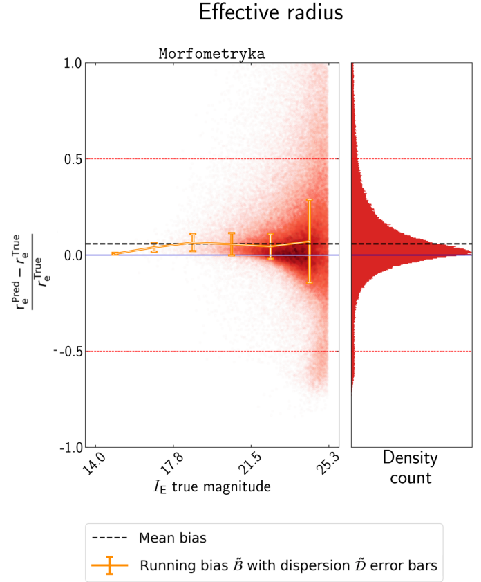
Fig. D.6. Trumpet plot for the single-Sérsic effective radius fitting, removing the objects flagged as “stars” by Morfometryka. We see that the bi-modality seen in Fig. 3 vanishes here.
