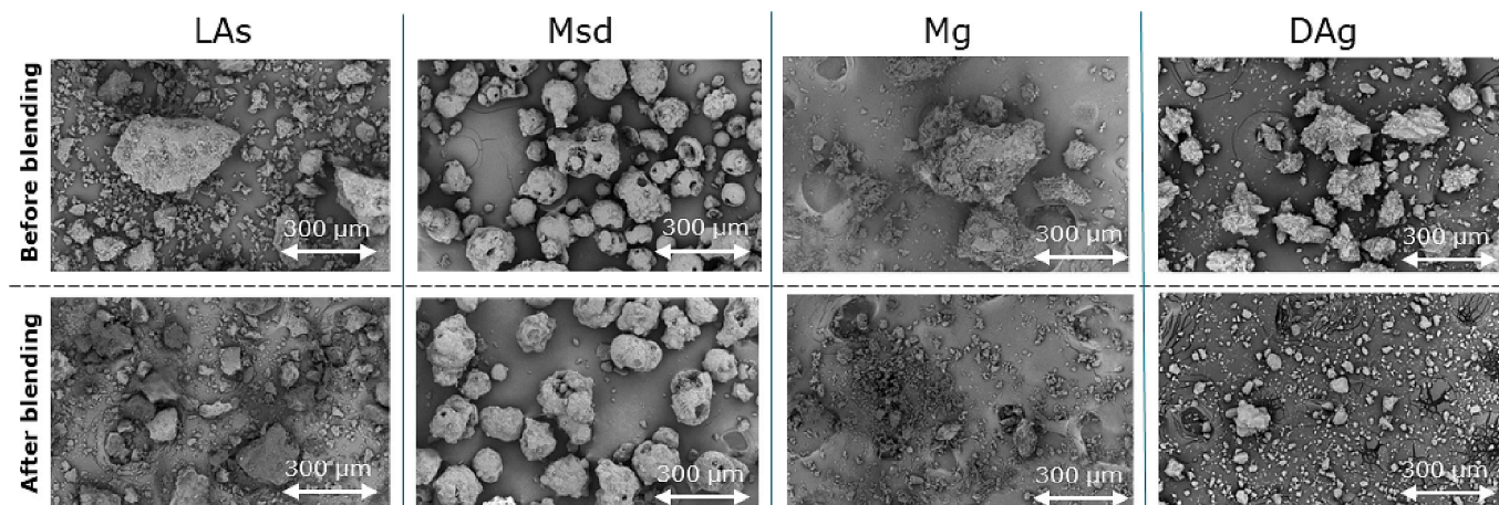
Fig. 3. SEM images of sieved lactose anhydrous (LAs), spray-dried mannitol (Msd), granular mannitol (Mg) and granular DCP anhydrate (DAG), before (top) and after (bottom) blending. LAs and Msd attrition is dominated by surface abrasion, while Mg and DAG attrition is dominated by fragmentation.
