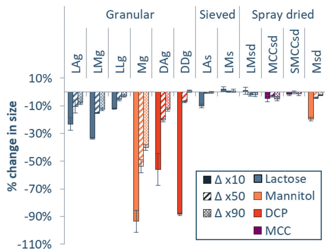
Fig. 2. Relative change in particle size distribution parameters x_{10} (solid bars), x_{50} (lined bars) and x_{90} (dotted bars) after blending lactose (blue), mannitol (orange), DCP (red), and MCC (purple) in a high shear blender. Error bars indicate the standard deviation. (For interpretation of the references to colour in this figure legend, the reader is referred to the web version of this article.)
