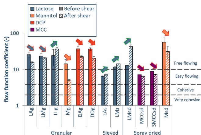
Fig. 5. Absolute change in flow function coefficient after blending different grades of lactose (blue), mannitol (orange), DCP (red), and MCC (purple) in a high shear blender. Error bars indicate the standard deviation. (For interpretation of the references to colour in this figure legend, the reader is referred to the web version of this article.)
