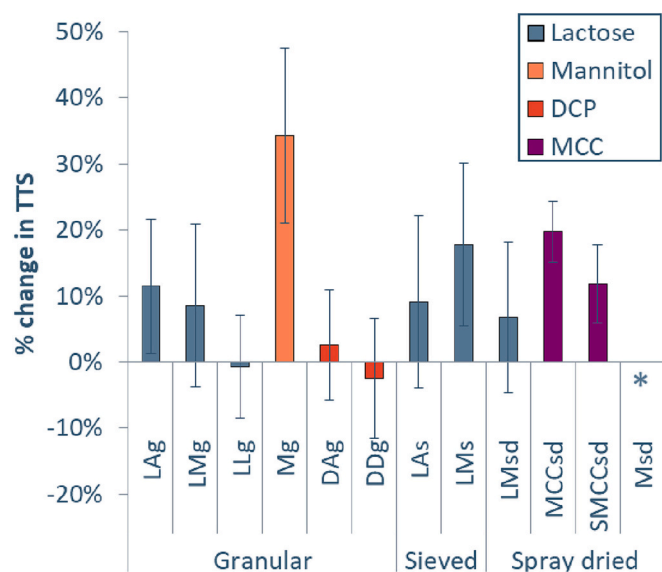
Fig. 6. Relative change in tablet tensile strength after blending lactose (blue), mannitol (orange), DCP (red), and MCC (purple) grades in a high shear blender. No data is available for Msd, due to punch sticking and capping of the tablets produced with this material. Error bars indicate the standard deviation. (For interpretation of the references to colour in this figure legend, the reader is referred to the web version of this article.)
