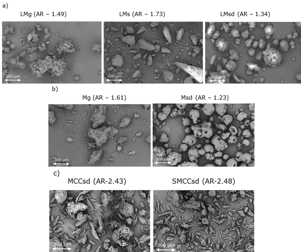
Fig. 1. SEM images and aspect ratios of starting material: Granular lactose monohydrate (LMg), sieved lactose monohydrate (LMs), spray-dried lactose monohydrate (LMsd) (a); granular mannitol (Mg), spray-dried mannitol (Msd) (b) and spray dried microcrystalline cellulose (MCCsd) and co-spray dried silicified microcrystalline cellulose (SMCCsd) (c). LMsd and Msd have a spherical morphology while LMg, LMs and Mg show an irregular surface morphology. MCC grades have a high aspect ratio due to their fibrous structure.
