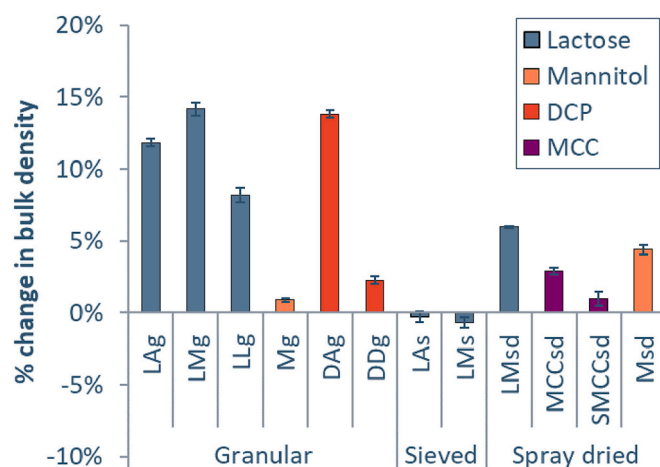
Fig. 4. Relative change in bulk density after blending different grades of lactose (blue), mannitol (orange), DCP (red), and MCC (purple) in a high shear blender. Error bars indicate the standard deviation. (For interpretation of the references to colour in this figure legend, the reader is referred to the web version of this article.)
