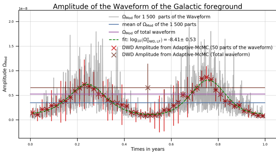
Fig. 43 Measurement of the orbital modulation of the white dwarf binary foreground. In grey: 1500 estimates of \Omega_{\text{Mod},i} = \frac{4\pi^2}{3H_0^3} \left(\frac{c}{2\pi L}\right)^2 A_i^2 ( A_i amplitude of the characteristic strain). In red: 50 MCMC results with 8 parameters (2 parameters for BBHs, 4 parameters for white dwarf binaries, 2 parameters for the LISA noise). In green, fit to the 50 MCMC run results to estimate the modulation from the LISA antenna pattern amplitude at 3 mHz. Modulation model: \Omega_{\text{Mod},i} = \Omega_{\text{DWD,LF}}^u (F_{+,i}^2 + F_{\times,i}^2) . Image reproduced with permission from Boileau et al. (2021b)
