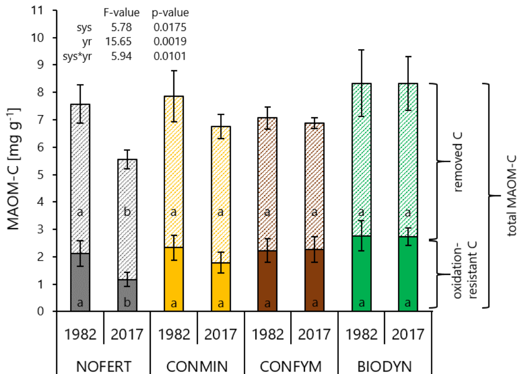
Figure 3.2: Efficiency of C removal in MAOM in all farming systems via treatment with NaOCl for the first (1982) and last year (2017) of observation. Filled columns show the C proportion that was not removed by NaOCl, i.e. resistant to oxidation, and shaded columns show the C proportion that was removed by NaOCl. Error bars show the standard deviation of the individual plots ( n = 4 ) per farming system. Results of a repeated two-way ANOVA (sys = farming system, yr = year) are depicted, using a linear mixed effect model that accounts for the spatial arrangement of plots within the experimental design. Post-hoc Tukey letters give significant differences between 1982 and 2017 at p < 0.05 .
