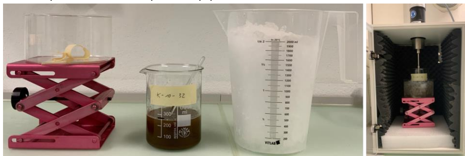
Figure S1.7: Laboratory equipment required for ultrasonication of the mineral soil.
