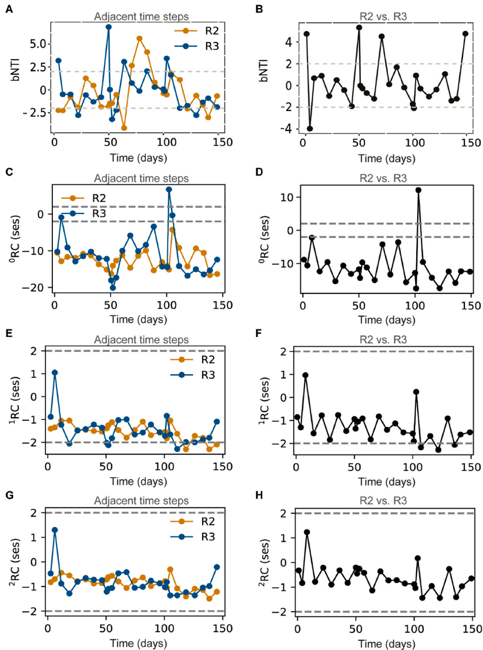
Fig. 6. Null model analysis results for \beta NTI and {}^n RC. A, \beta NTI between two successive sample points; B, \beta NTI between replicate reactors; C, {}^0 RC between two successive sample points; D, {}^0 RC between the replicate reactors; E, {}^1 RC between two successive sample points; F, {}^1 RC between the replicate reactors; G, {}^2 RC between two successive sample points; H, {}^2 RC between the replicate reactors.
