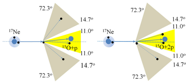
Fig. 1 Schematic illustration of the two types of reactions with a ^{17}\text{Ne} beam on a hydrogen target. i Proton knockout from a proton halo (left). ii Excitation of ^{17}\text{Ne} , leading to the formation of ^{15}\text{O} and two protons (right). The angular regions covered by the two detector complexes, at small angles and at large angles, are shown in yellow and beige coloured shadows. The proton knockout reaction channel is obtained by requiring either two protons in the Crystal Ball or one proton at small angles
