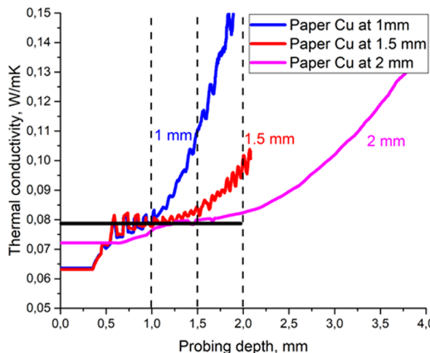
FIG. 2. Thermal conductivity in the normal direction vs depth profile of the paper stack with defects at different locations. The constant black line represents the \lambda_{through-plane} obtained using the anisotropic method. 12
