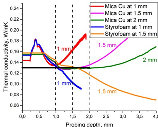
FIG. 1. Thermal conductivity in the normal direction vs depth profile of the mica stack with defects at different locations. The constant black line represents the \lambda_{through-plane} obtained using the anisotropic method. 12
