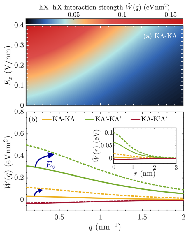
Fig. 2 Hybrid exciton–exciton interactions. (a) Momentum- and electric-field dependent interaction strength involving KA hX. The interaction strength increases as the interlayer component is enhanced under the application of an out-of-plane electric field, E_z . (b) Momentum-dependent interaction strengths for different electric fields and between different types of hybrid excitons. Solid lines correspond to the case E_z = 0 and dashed lines to the case of E_z = 0.3 \text{ V nm}^{-1} . The inset shows the corresponding real-space interaction, \tilde{W}(r) .
