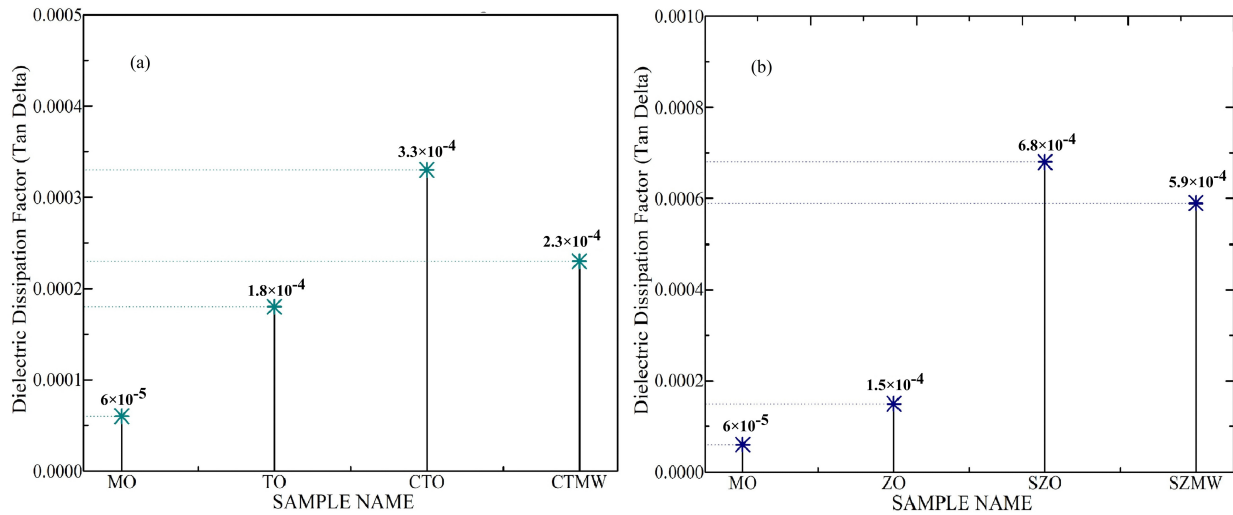
Figure 9. (a) tan δ value of different titania nanofluid samples, (b) tan δ value of different zinc nanofluid samples.
